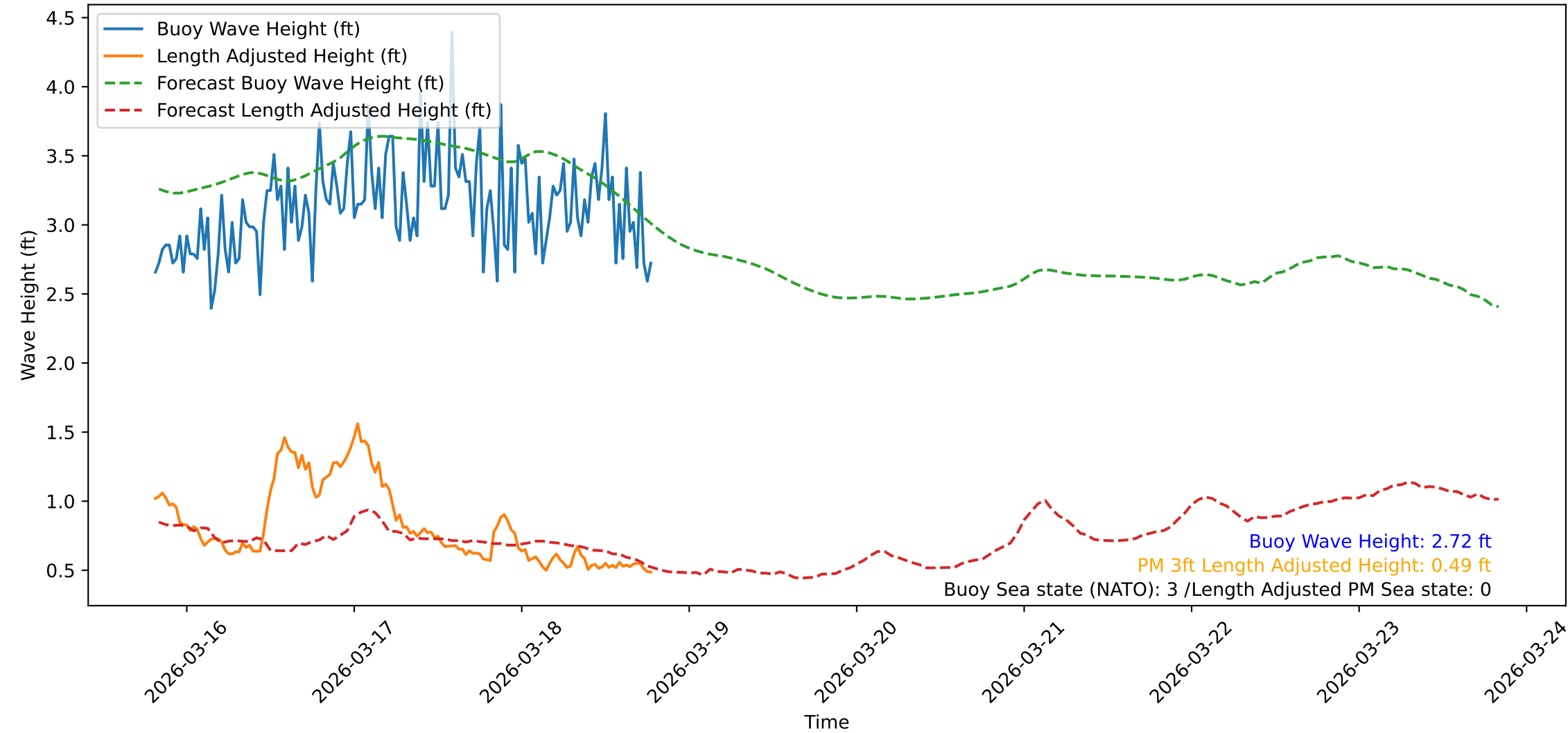
Wave Heights over Time for Oceanside Harbor at 2026-03-18 19:30:31
