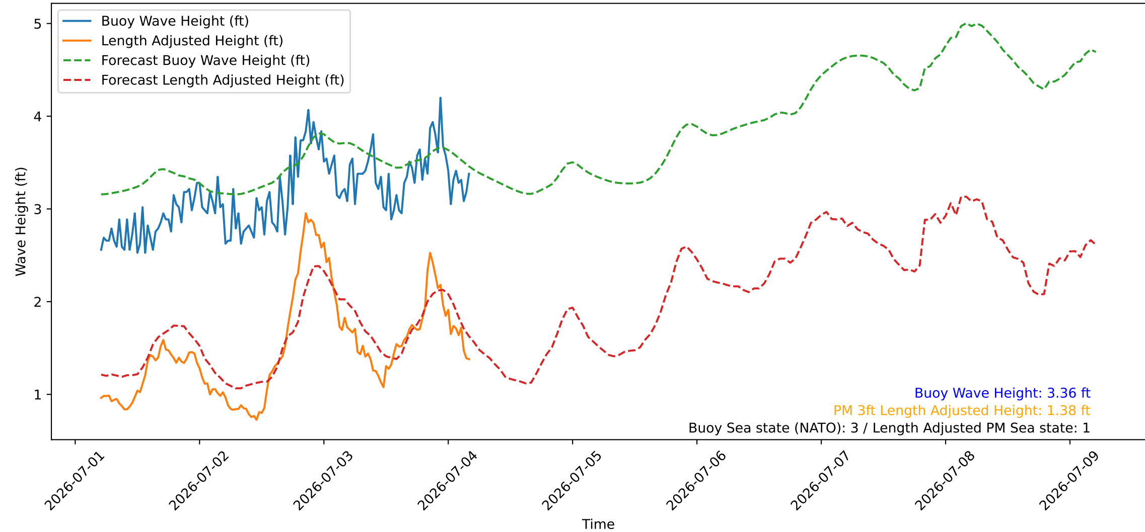
Wave Heights over Time for Green Beach at 2026-07-04 04:51:09
