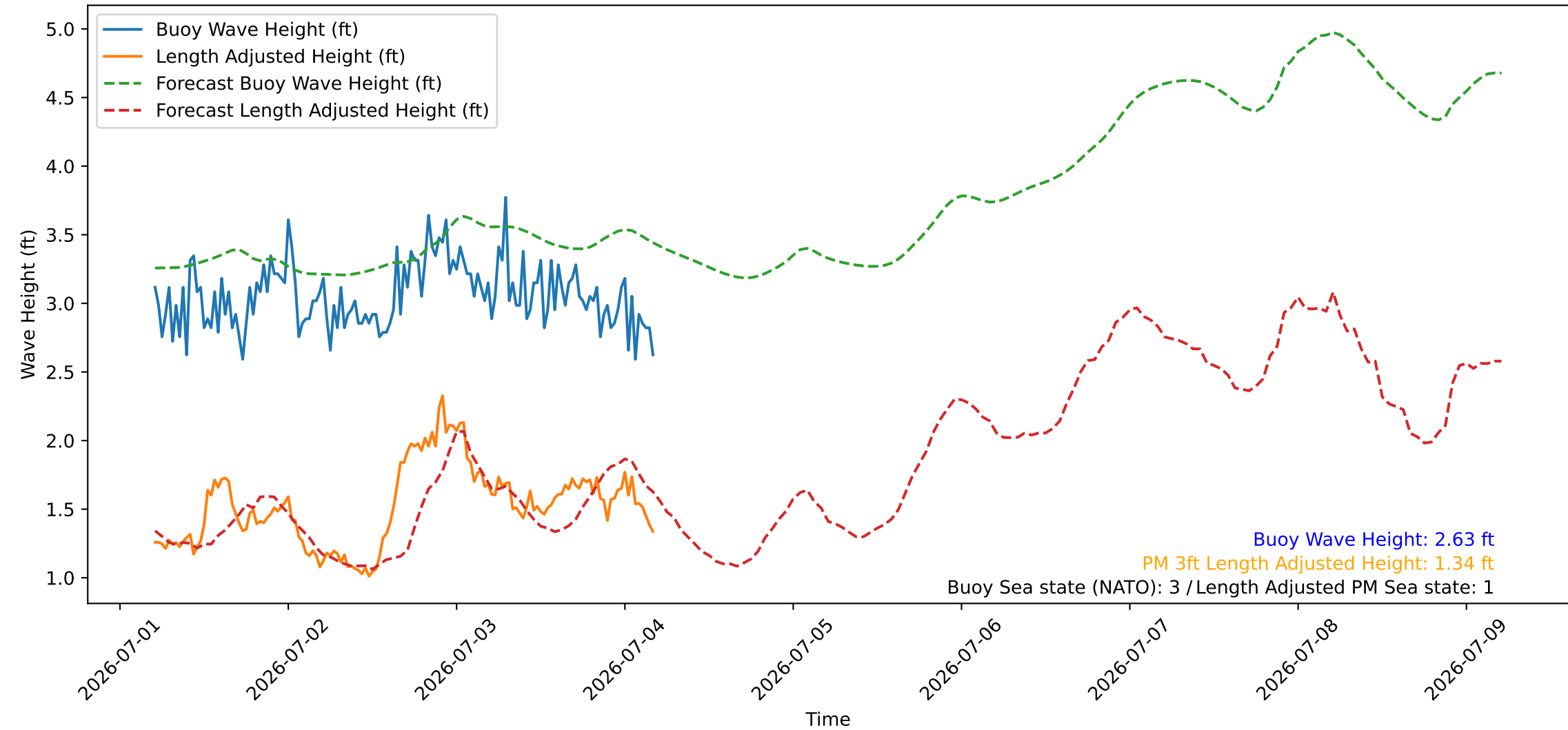
Wave Heights over Time for Oceanside Harbor at 2026-07-04 04:50:26
