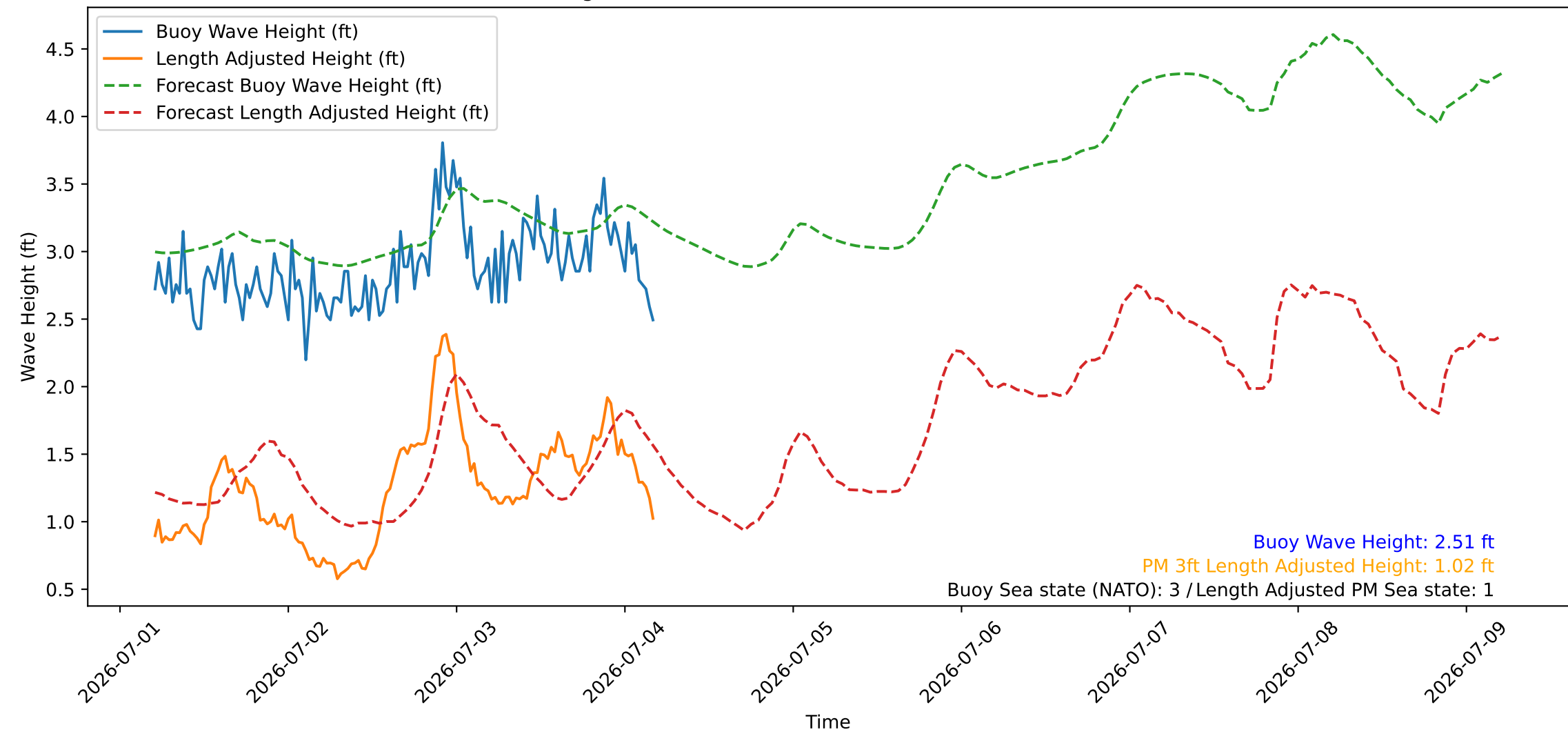
Wave Heights over Time for Red Beach at 2026-07-04 04:50:47
