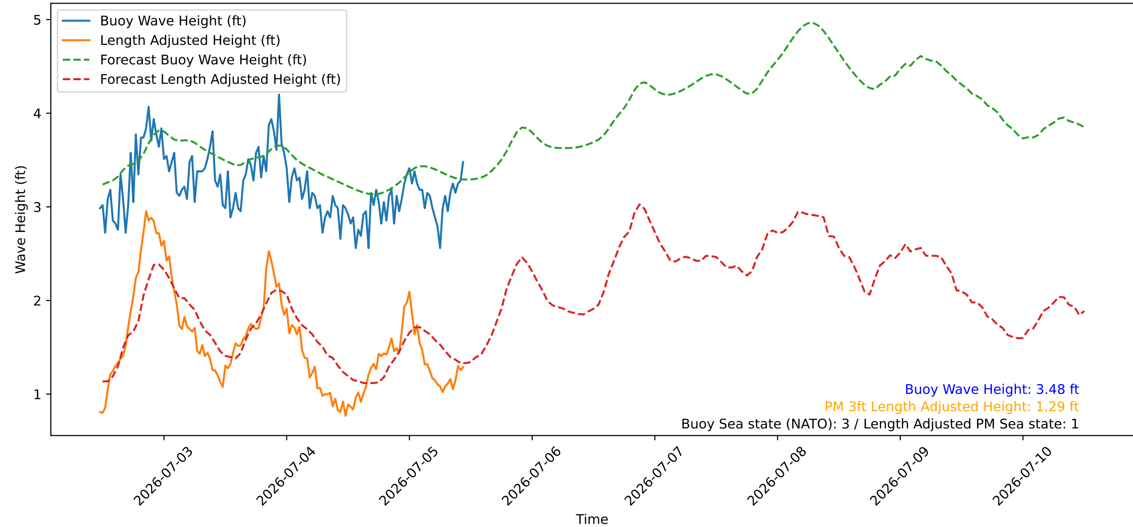
Wave Heights over Time for Green Beach at 2026-07-05 11:31:10
