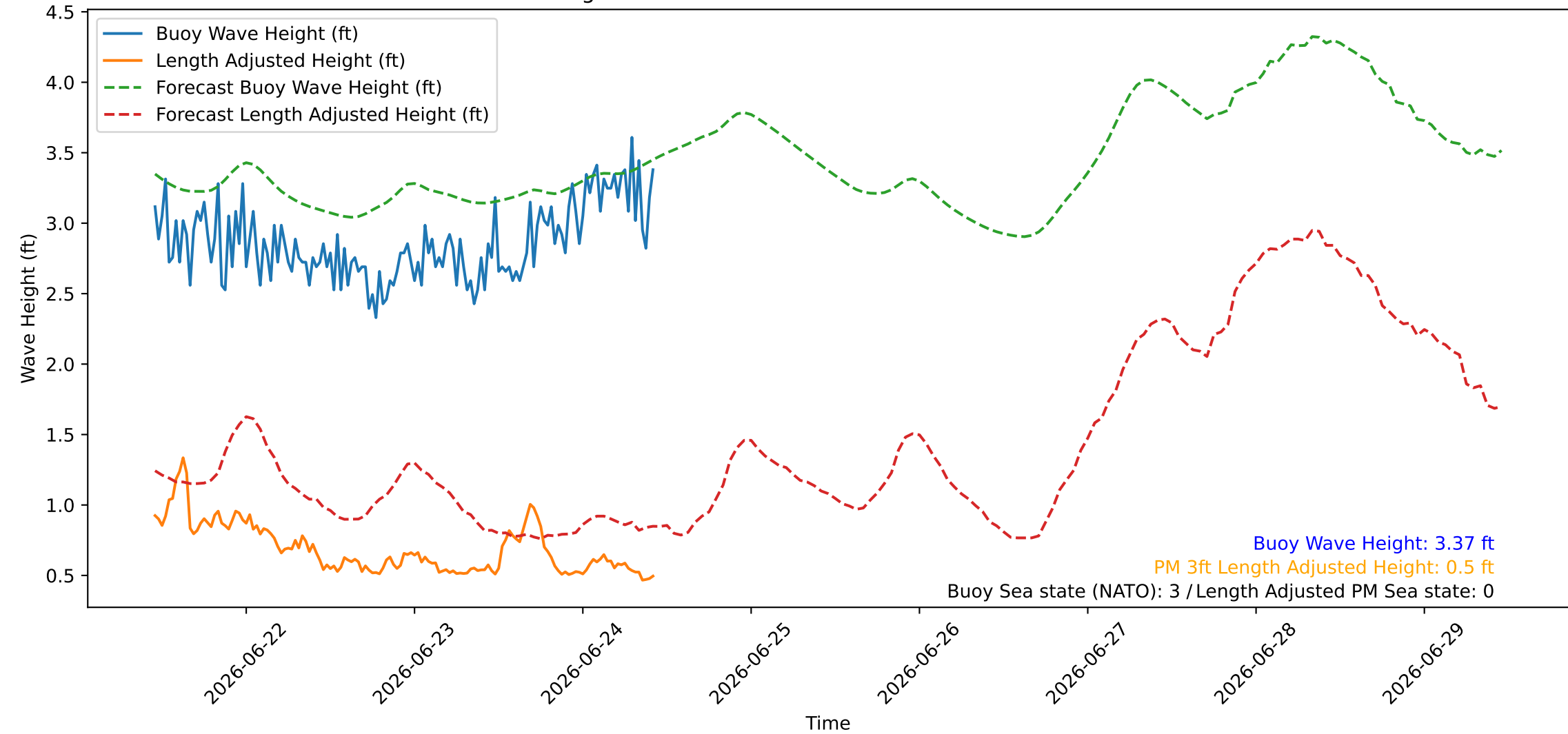
Wave Heights over Time for Red Beach at 2026-06-24 10:40:45
