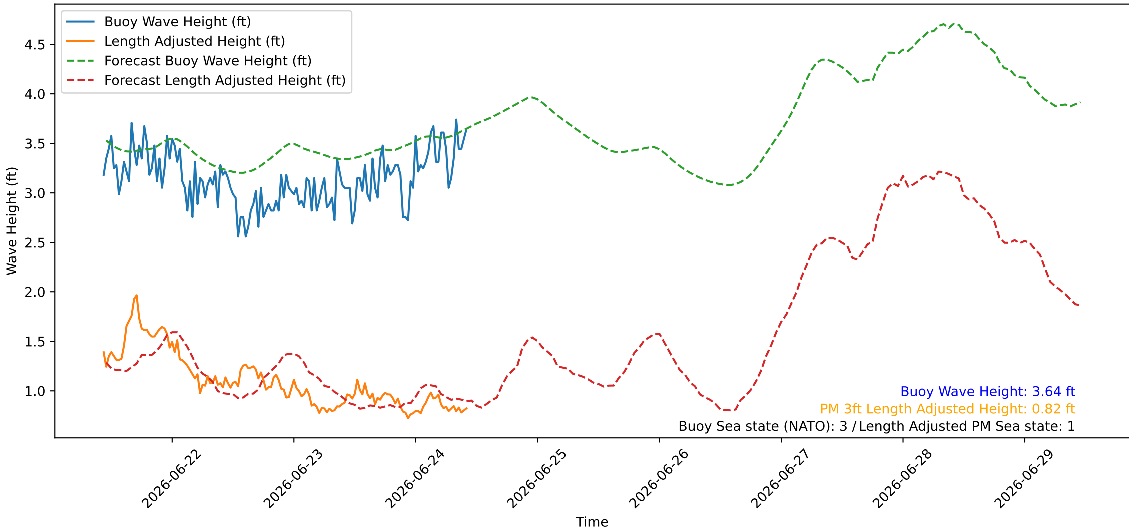
Wave Heights over Time for Oceanside Harbor at 2026-06-24 10:40:26
