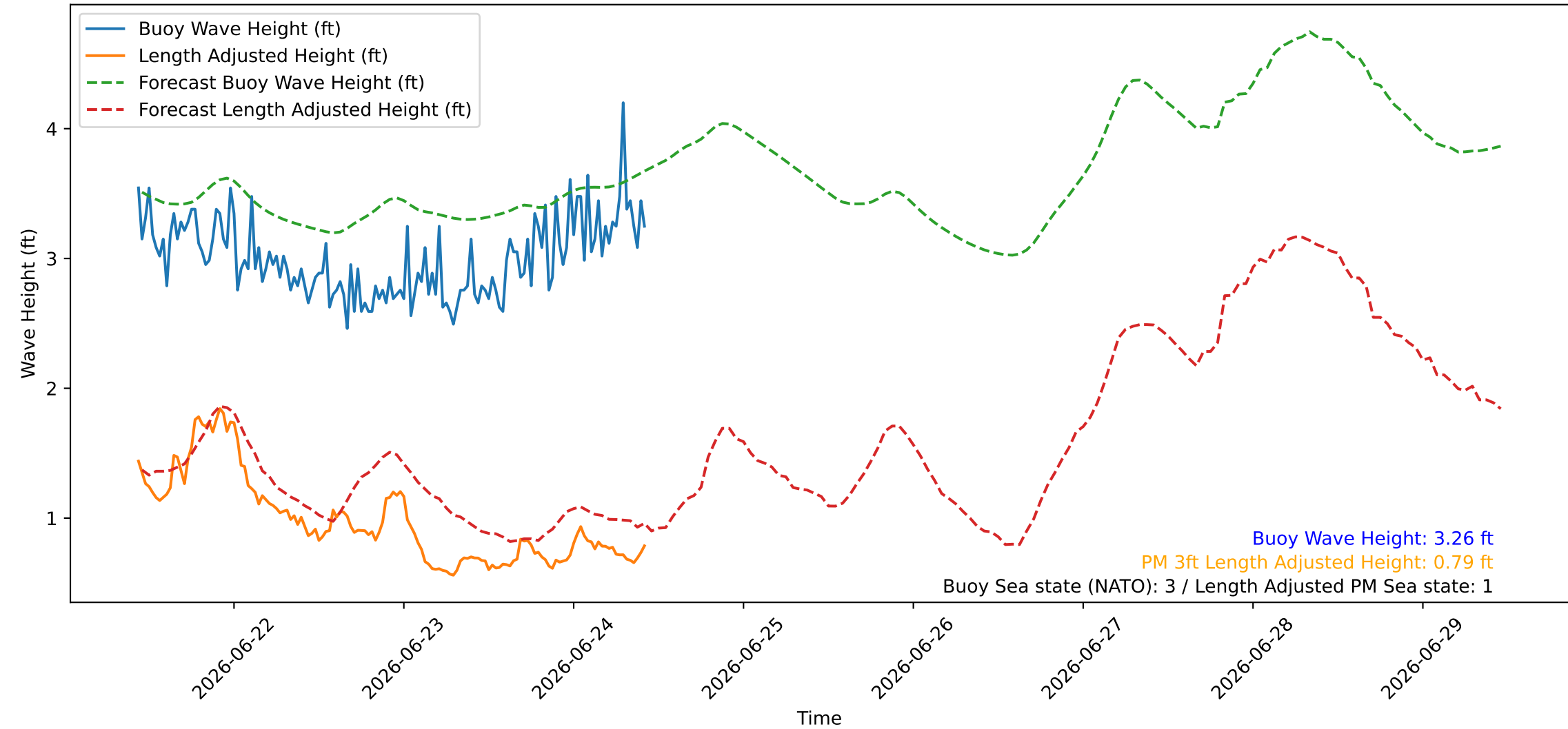
Wave Heights over Time for Green Beach at 2026-06-24 10:41:08
