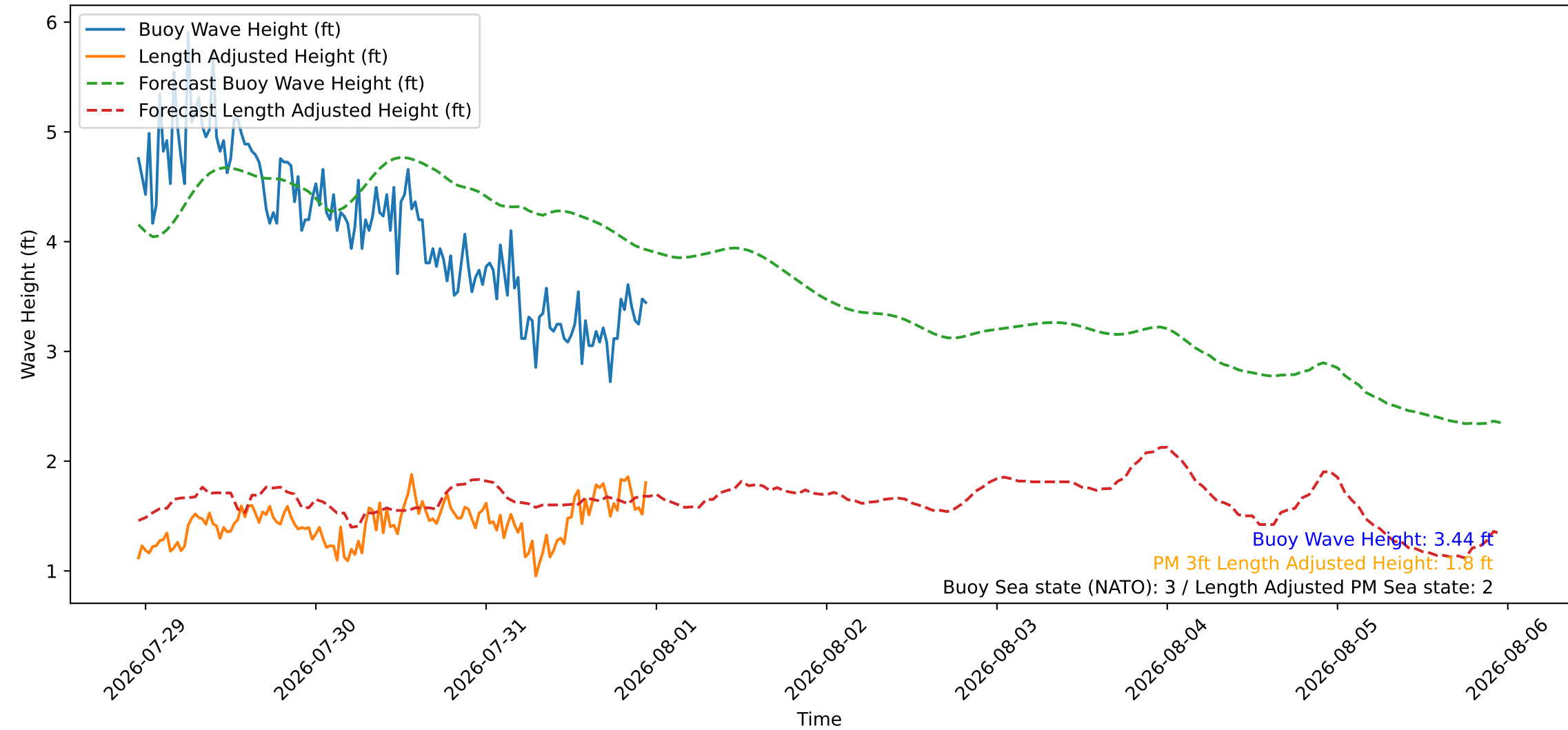
Wave Heights over Time for Oceanside Harbor at 2026-07-31 23:10:27
