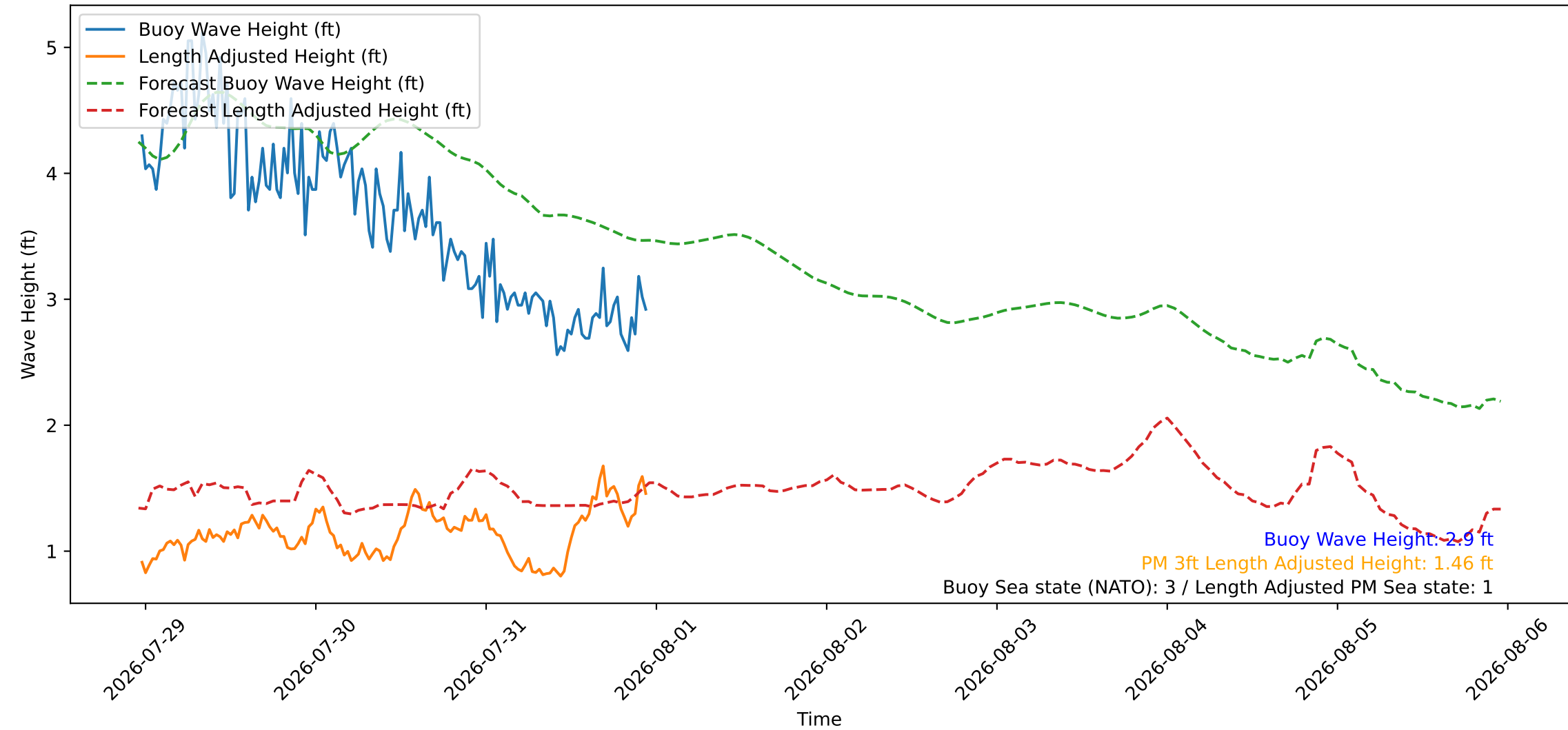
Wave Heights over Time for Red Beach at 2026-07-31 23:10:46
