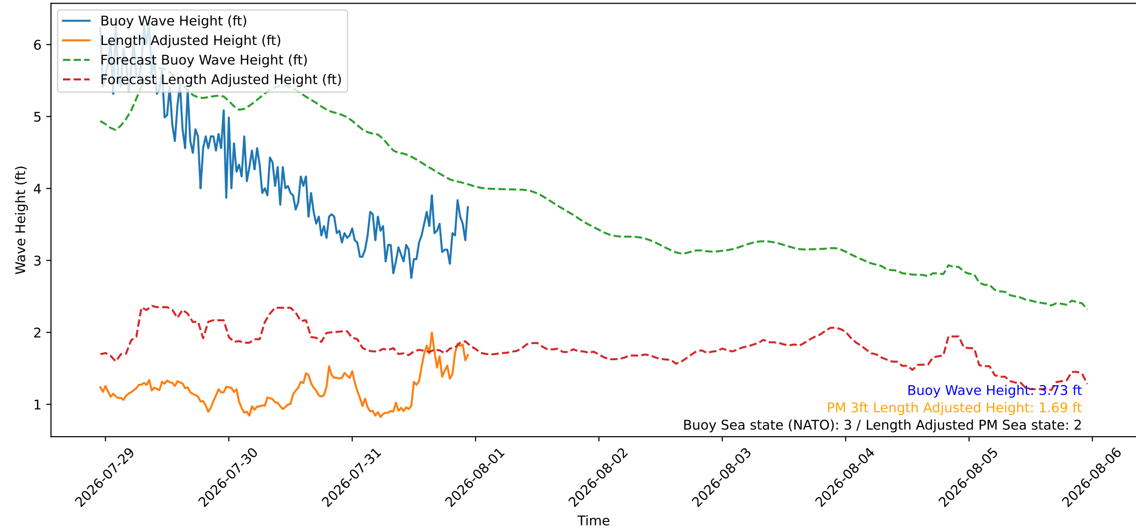
Wave Heights over Time for Green Beach at 2026-07-31 23:11:09
