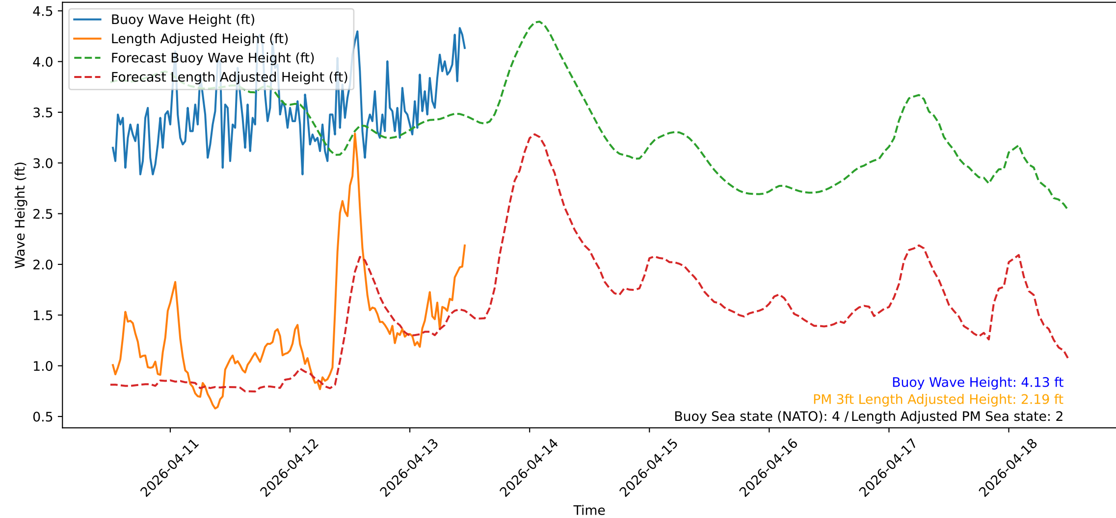
Wave Heights over Time for Red Beach at 2026-04-13 12:00:50
