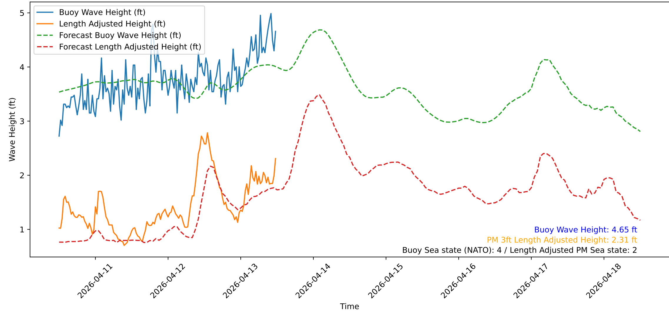
Wave Heights over Time for Oceanside Harbor at 2026-04-13 12:00:31
