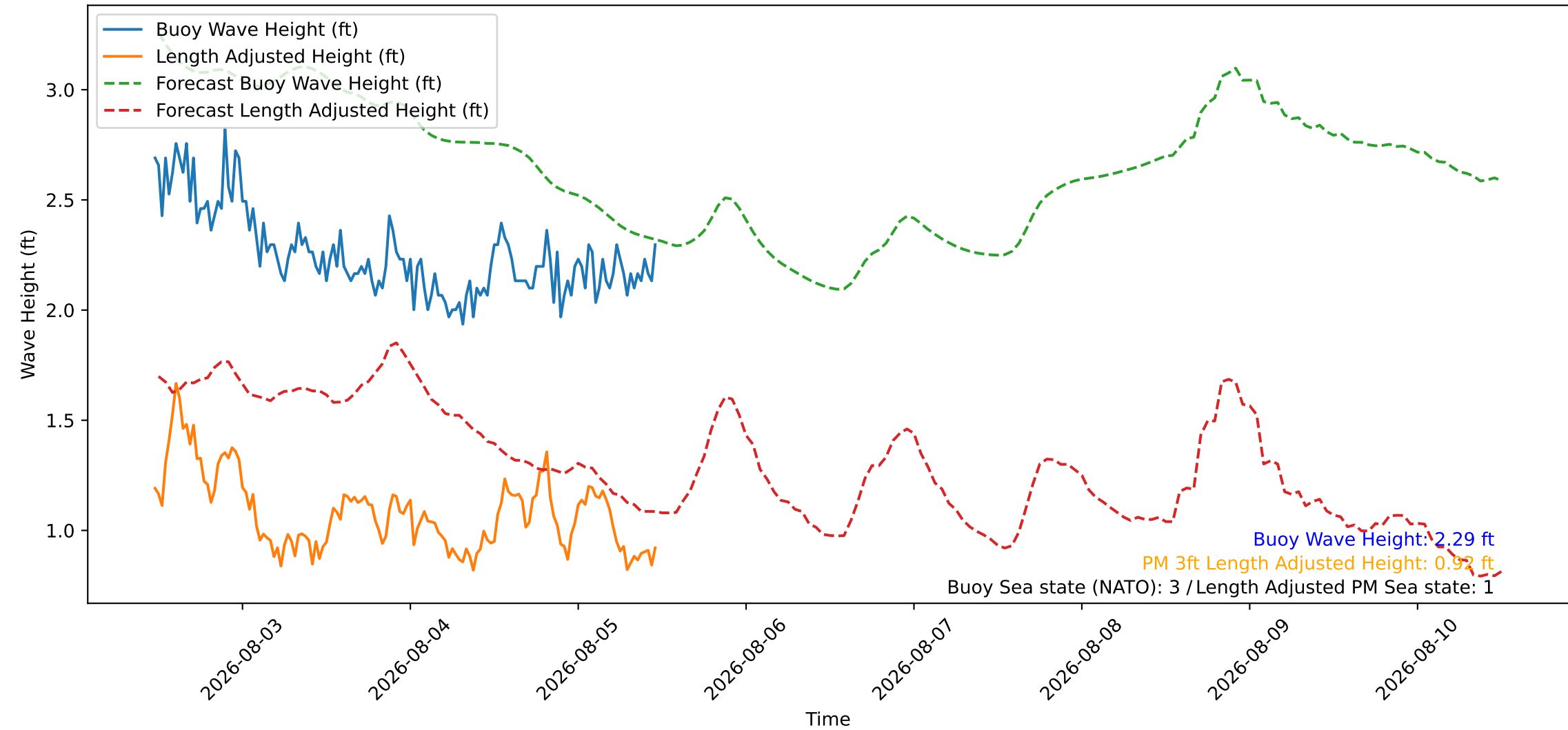
Wave Heights over Time for Green Beach at 2026-08-05 11:41:09
