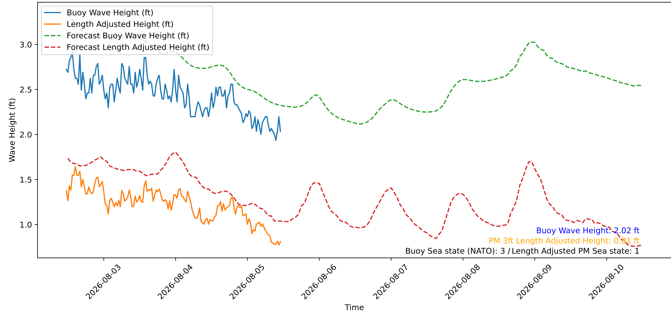
Wave Heights over Time for Oceanside Harbor at 2026-08-05 11:40:27
