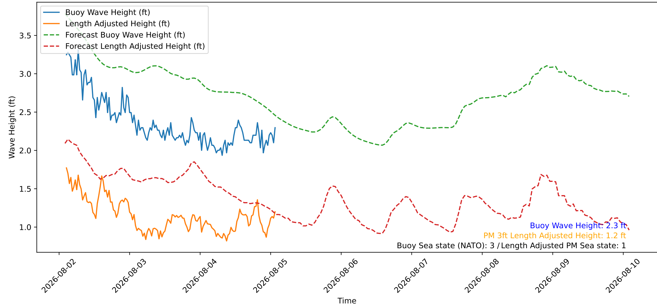
Wave Heights over Time for Green Beach at 2026-08-05 02:21:09
