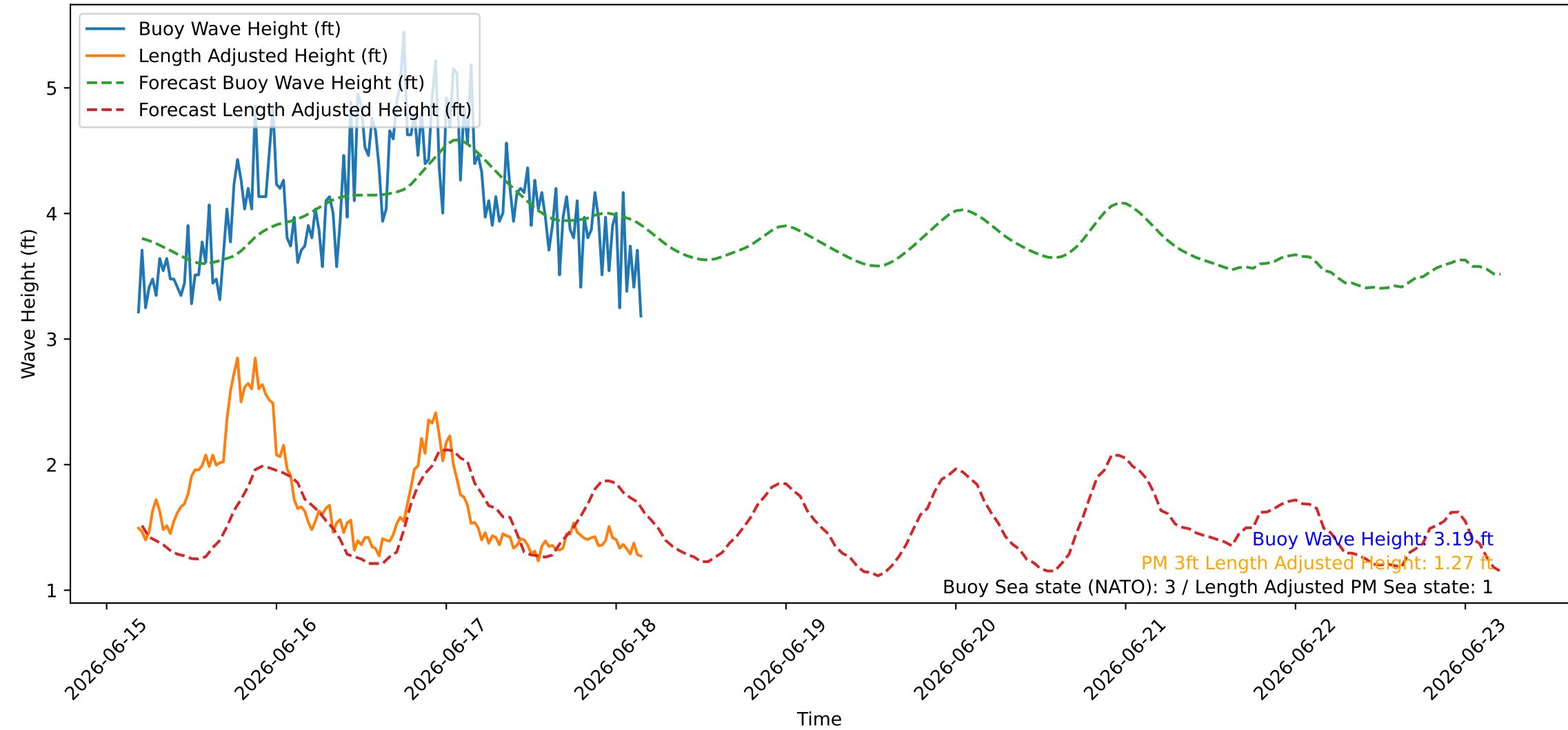
Wave Heights over Time for Oceanside Harbor at 2026-06-18 04:40:26
