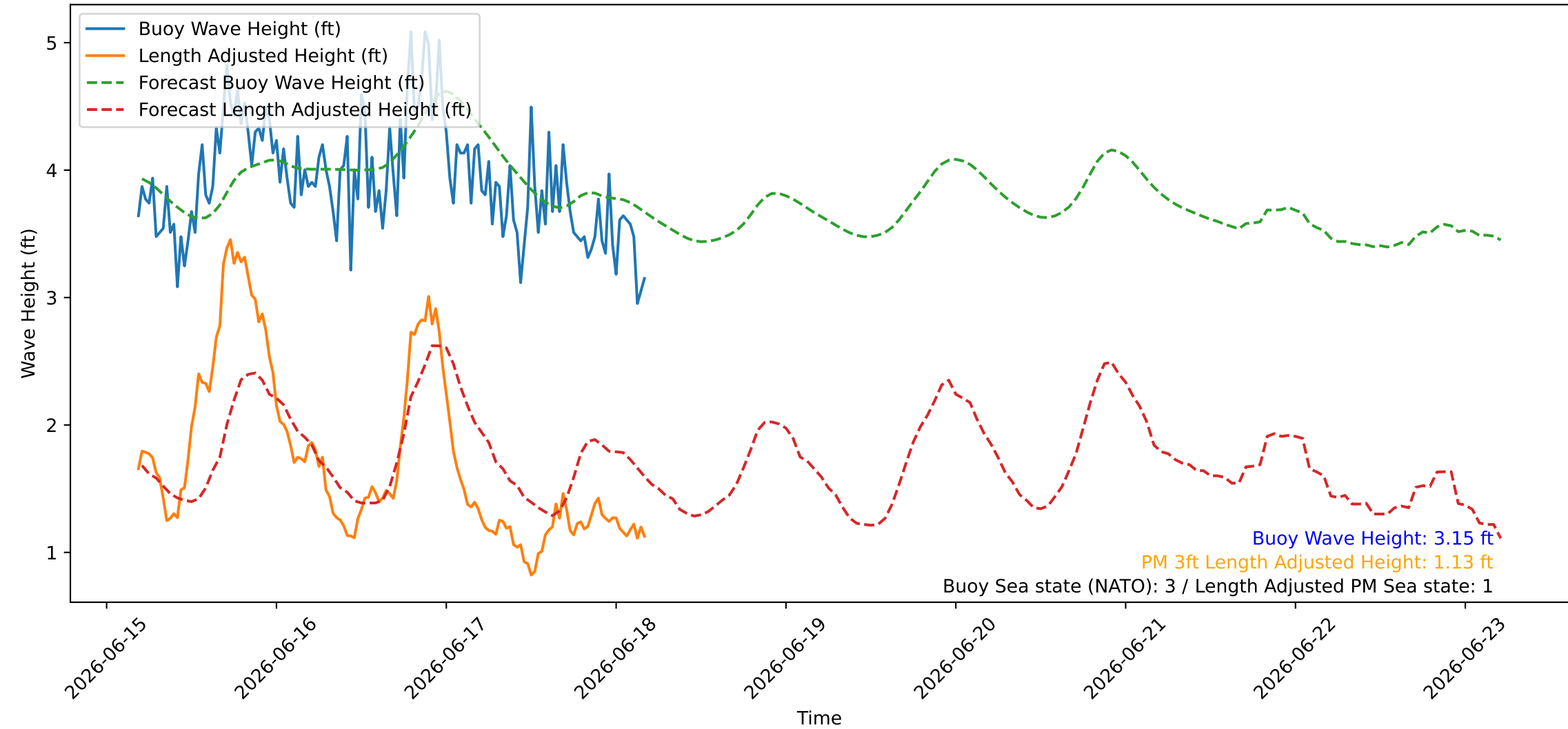
Wave Heights over Time for Green Beach at 2026-06-18 04:41:08
