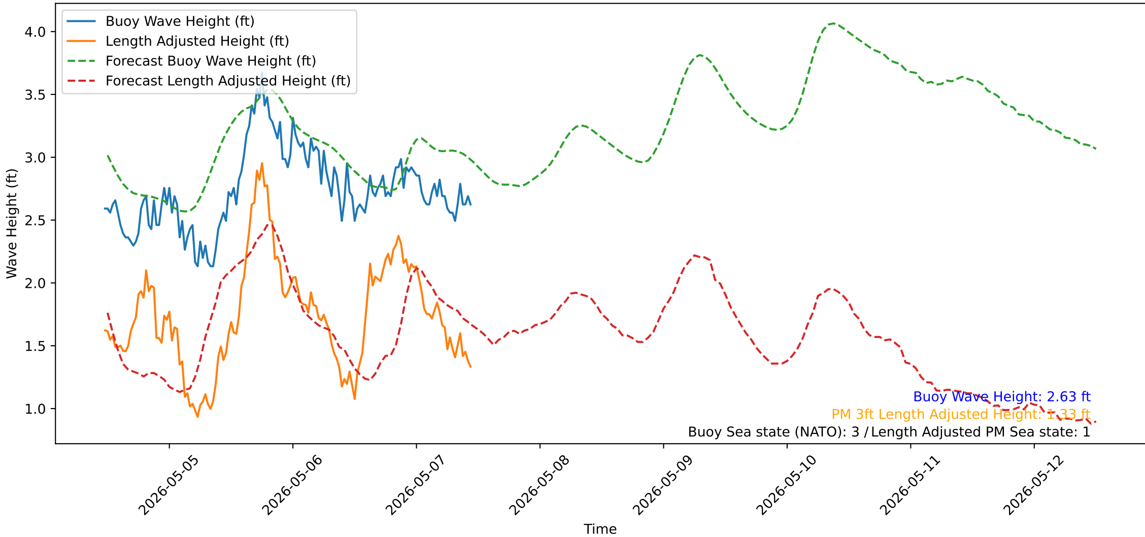
Wave Heights over Time for Green Beach at 2026-05-07 11:31:12
