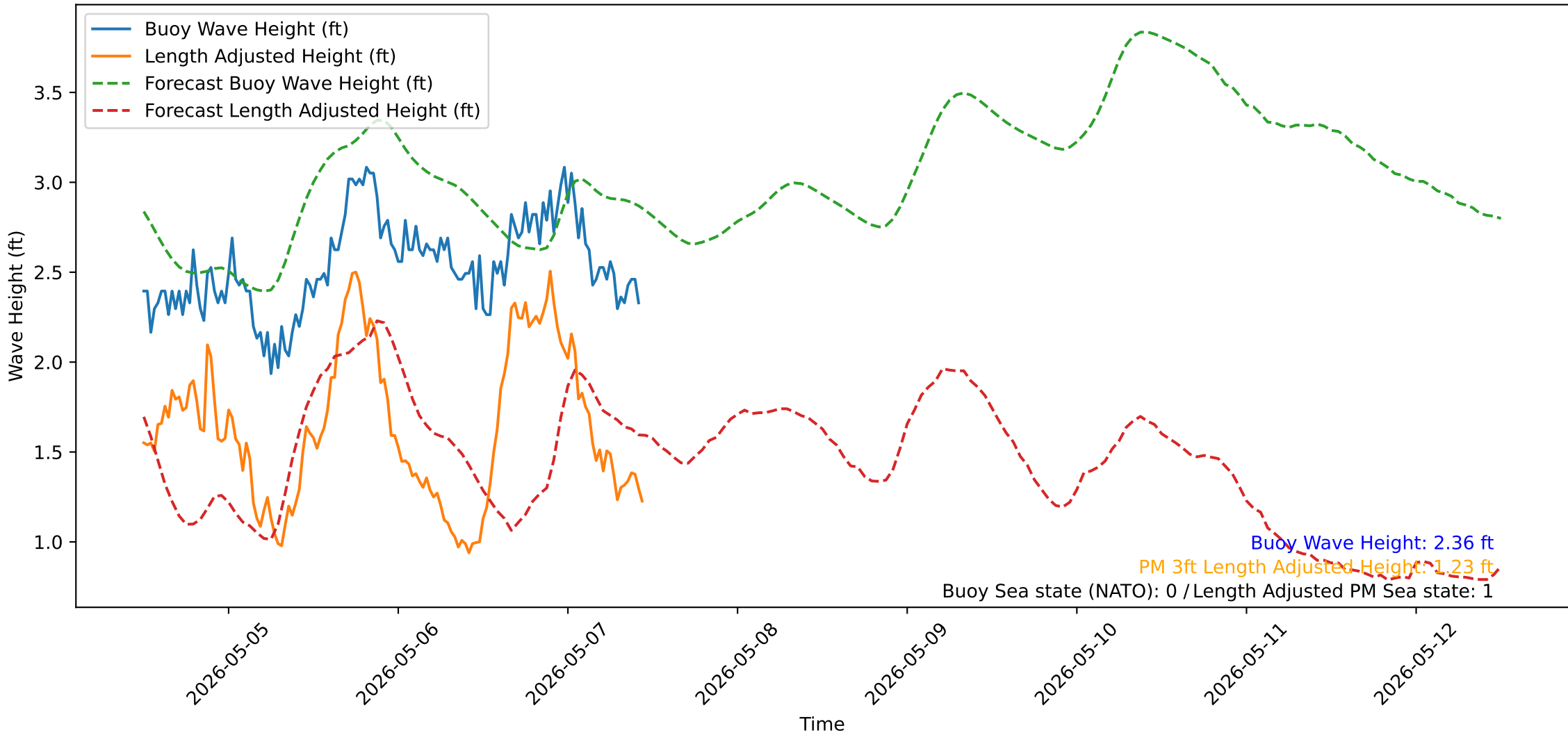
Wave Heights over Time for Red Beach at 2026-05-07 11:30:50
