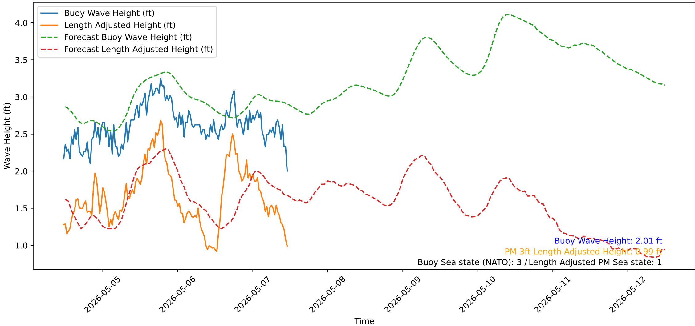
Wave Heights over Time for Oceanside Harbor at 2026-05-07 11:30:31
