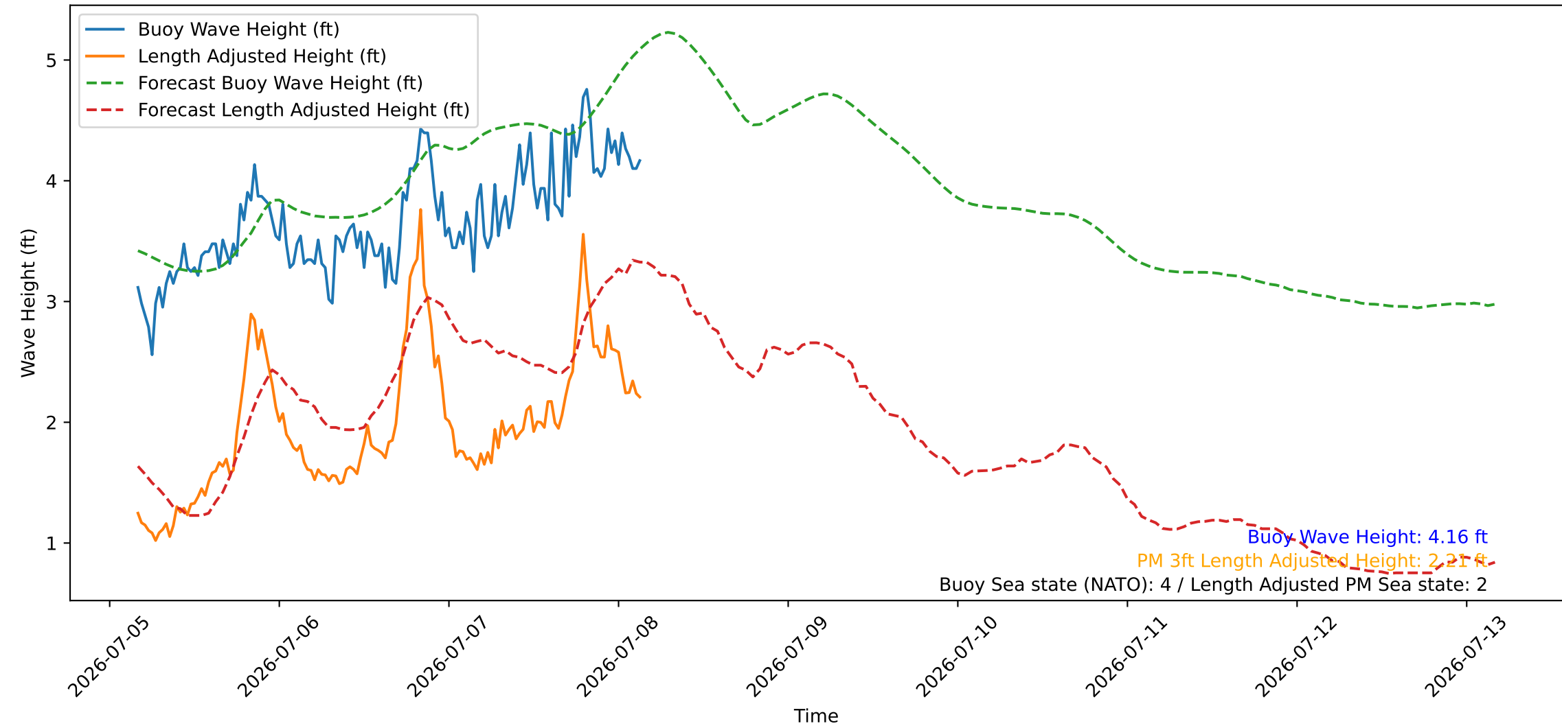
Wave Heights over Time for Green Beach at 2026-07-08 04:01:07
