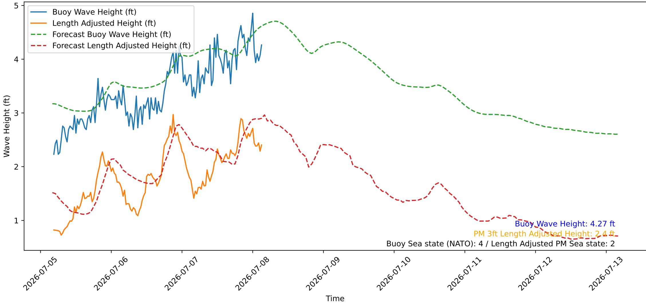
Wave Heights over Time for Red Beach at 2026-07-08 04:00:45
