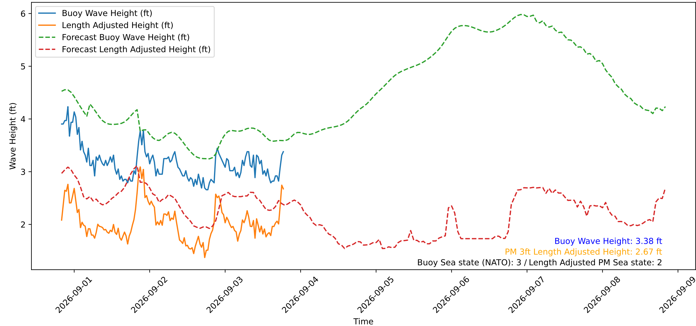
Wave Heights over Time for Green Beach at 2026-09-03 19:51:15
