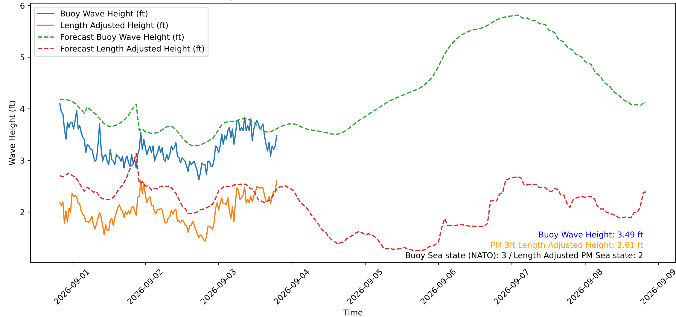
Wave Heights over Time for Oceanside Harbor at 2026-09-03 19:50:30
