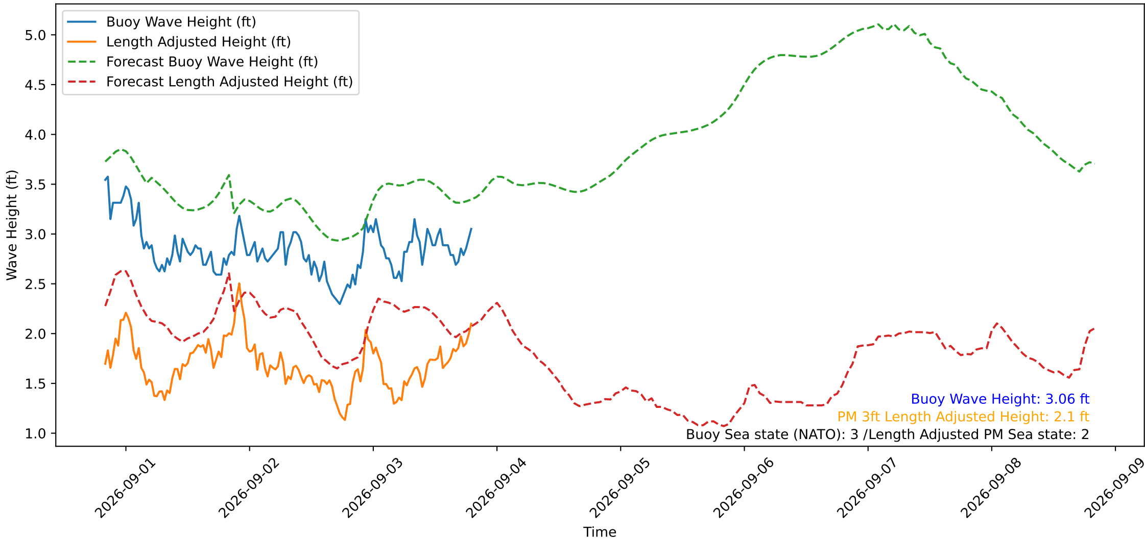
Wave Heights over Time for Red Beach at 2026-09-03 19:50:51
