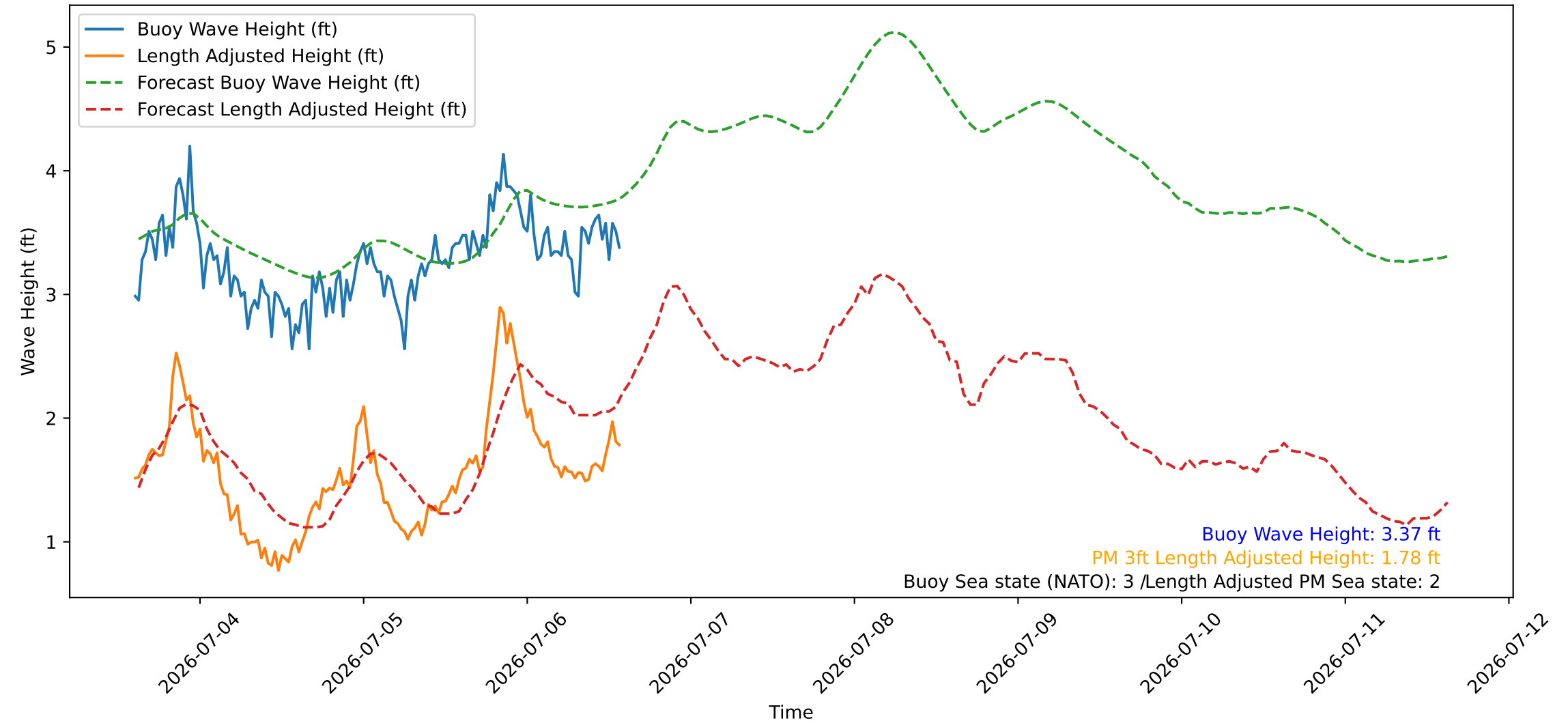
Wave Heights over Time for Green Beach at 2026-07-06 14:31:08
