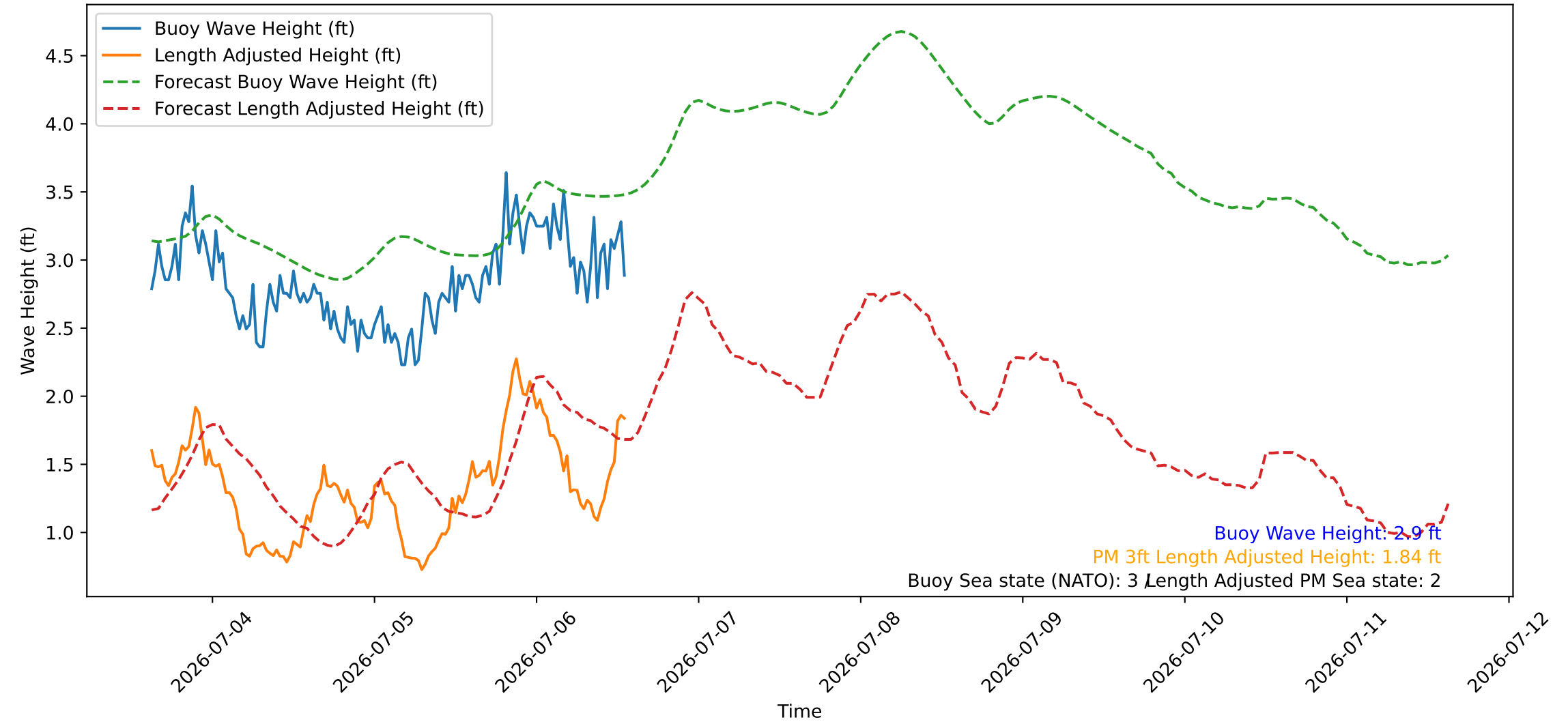
Wave Heights over Time for Red Beach at 2026-07-06 14:30:46
