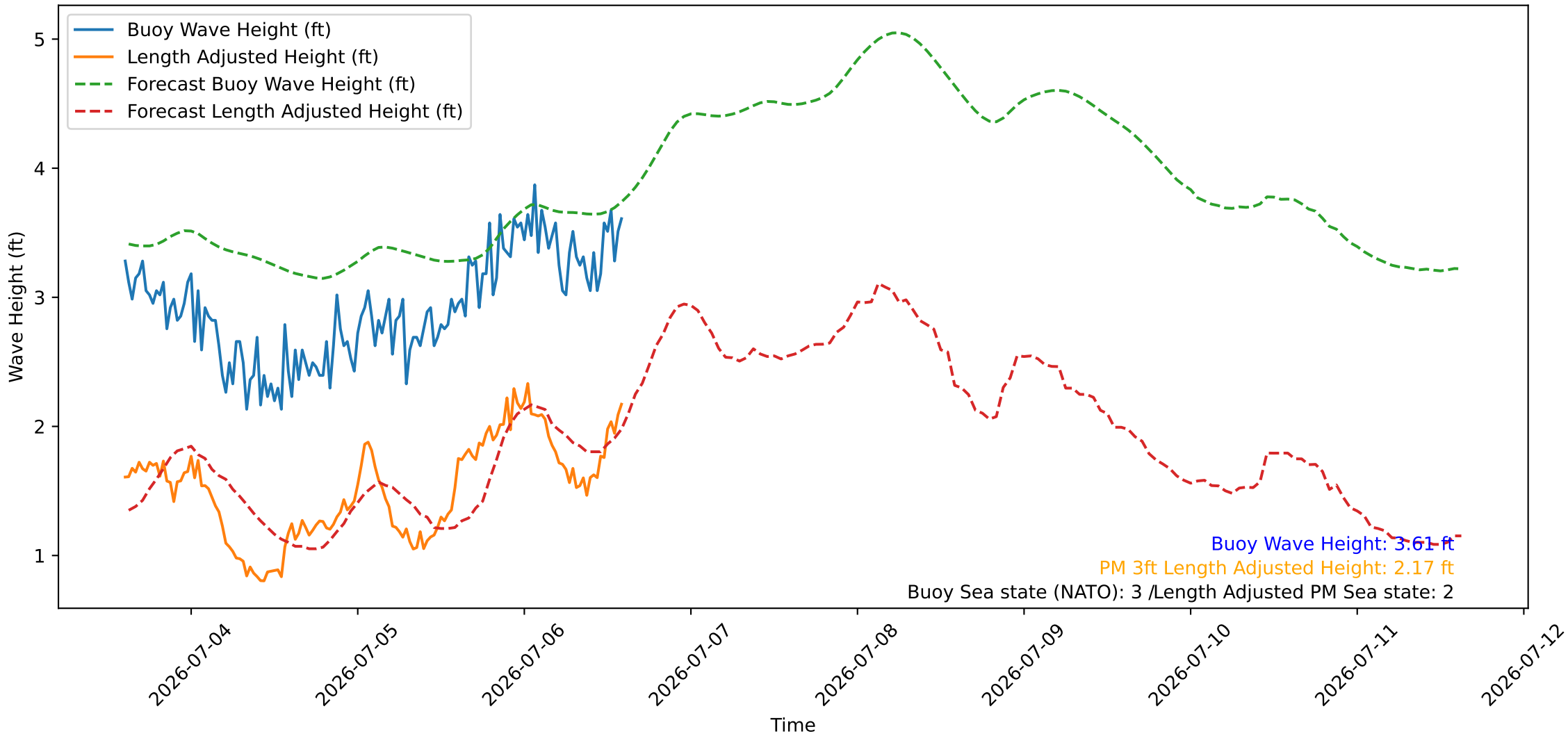
Wave Heights over Time for Oceanside Harbor at 2026-07-06 14:30:26
