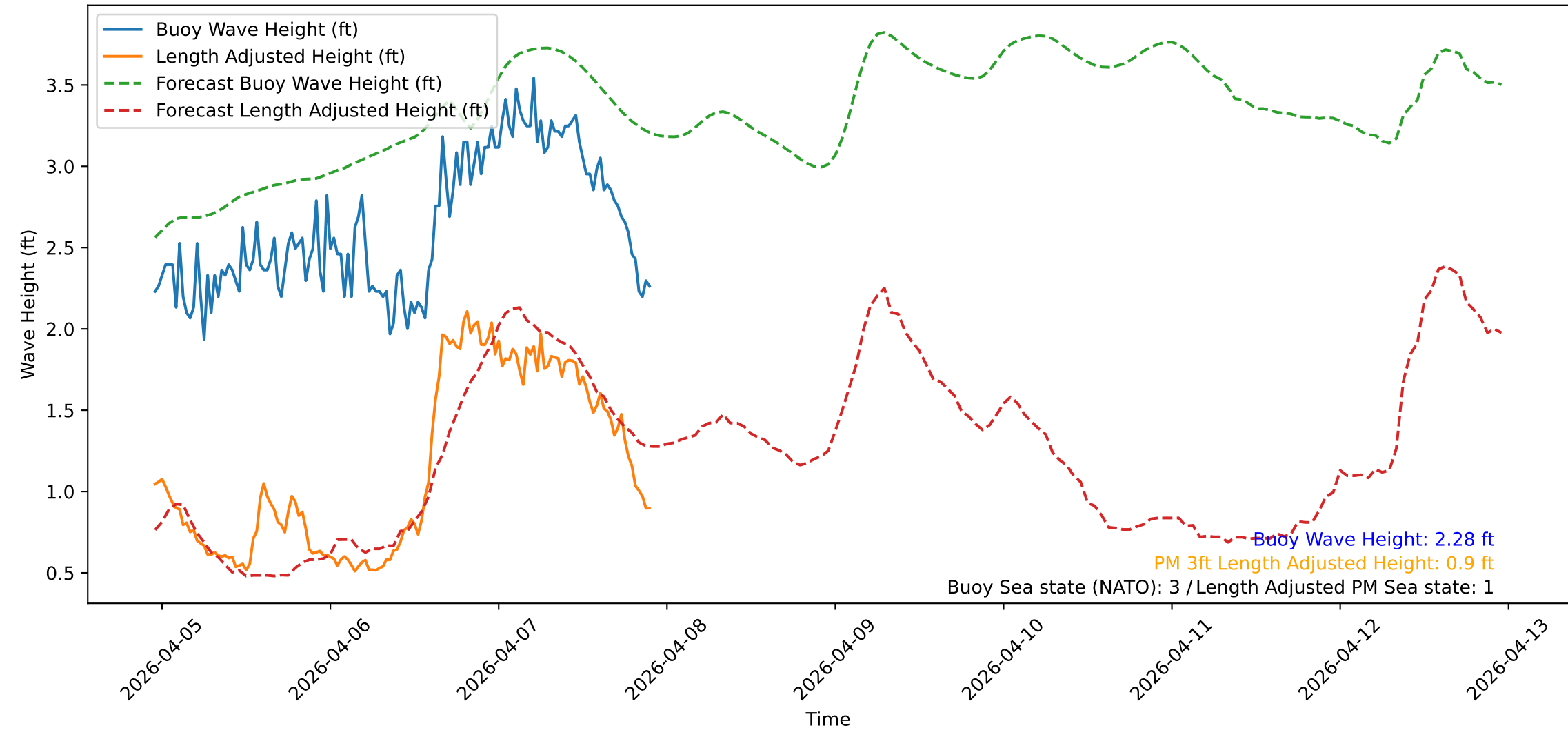
Wave Heights over Time for Red Beach at 2026-04-07 22:30:48
