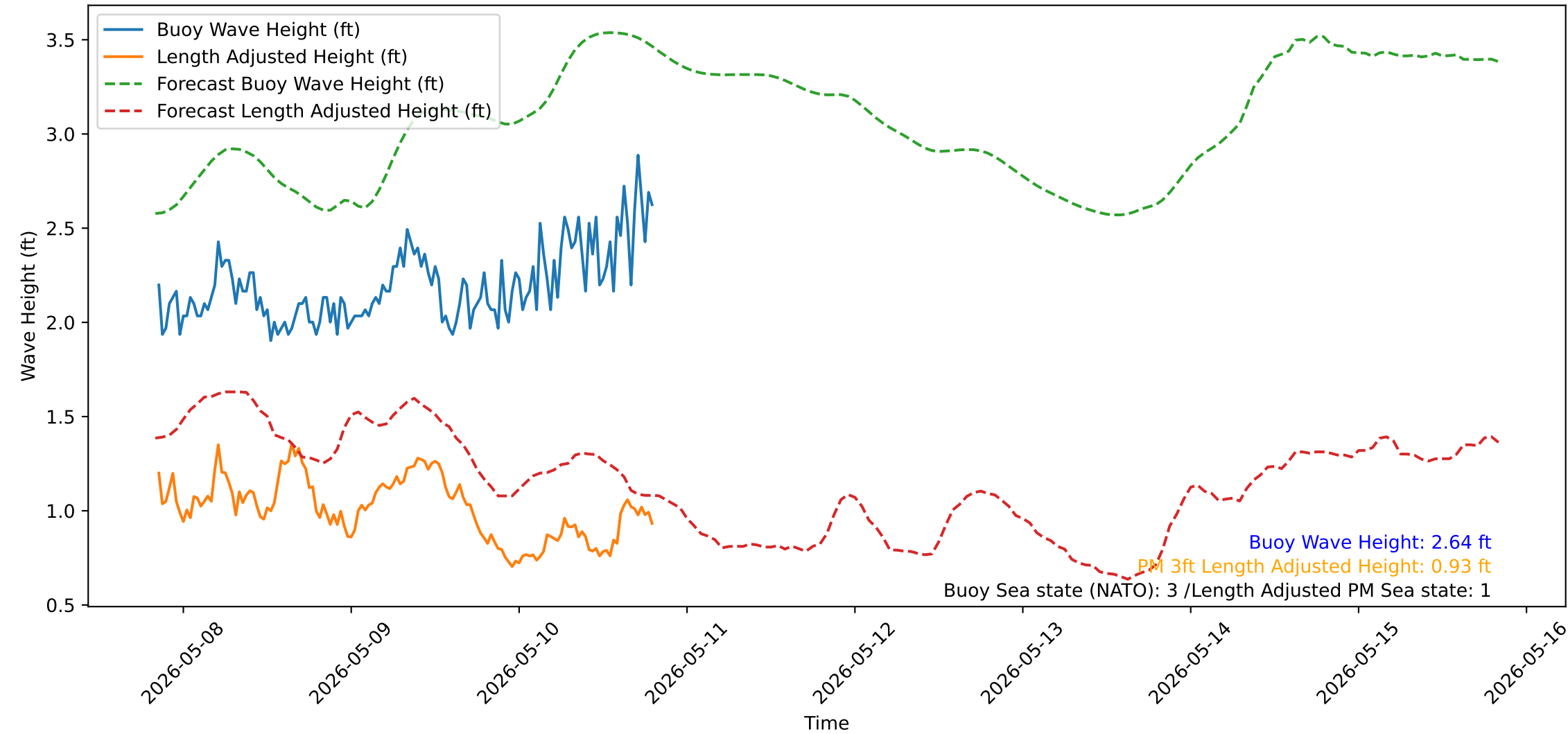
Wave Heights over Time for Red Beach at 2026-05-10 20:00:50
