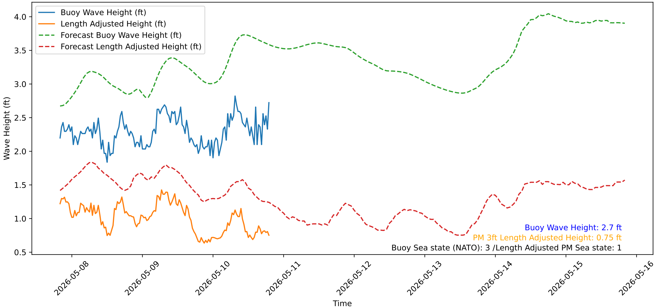
Wave Heights over Time for Green Beach at 2026-05-10 20:01:12
