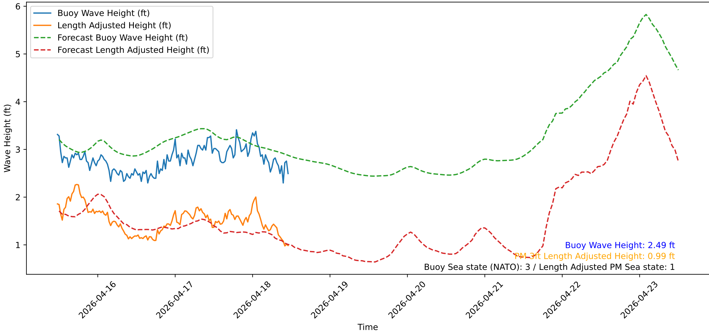
Wave Heights over Time for Oceanside Harbor at 2026-04-18 11:30:31
