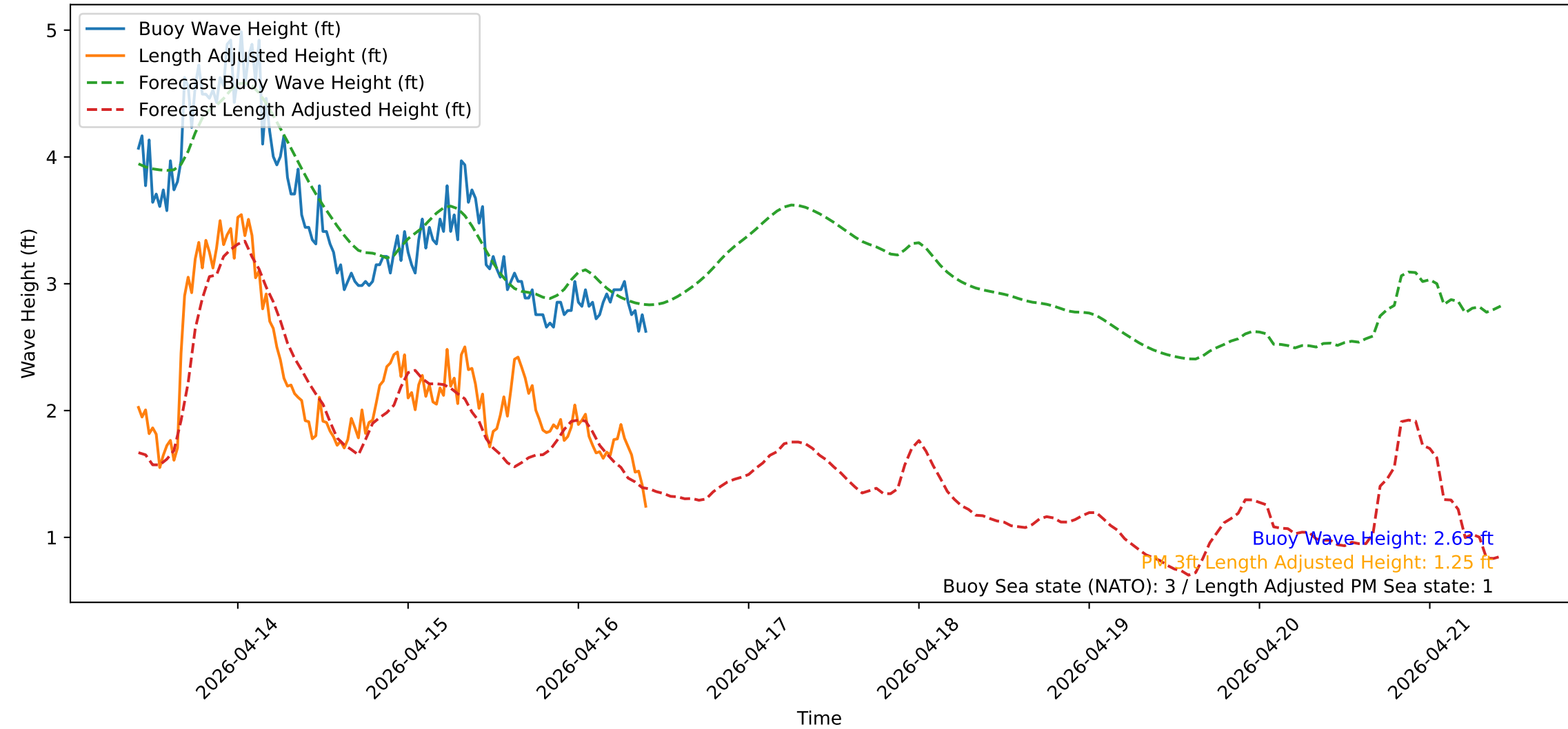
Wave Heights over Time for Green Beach at 2026-04-16 10:11:12
