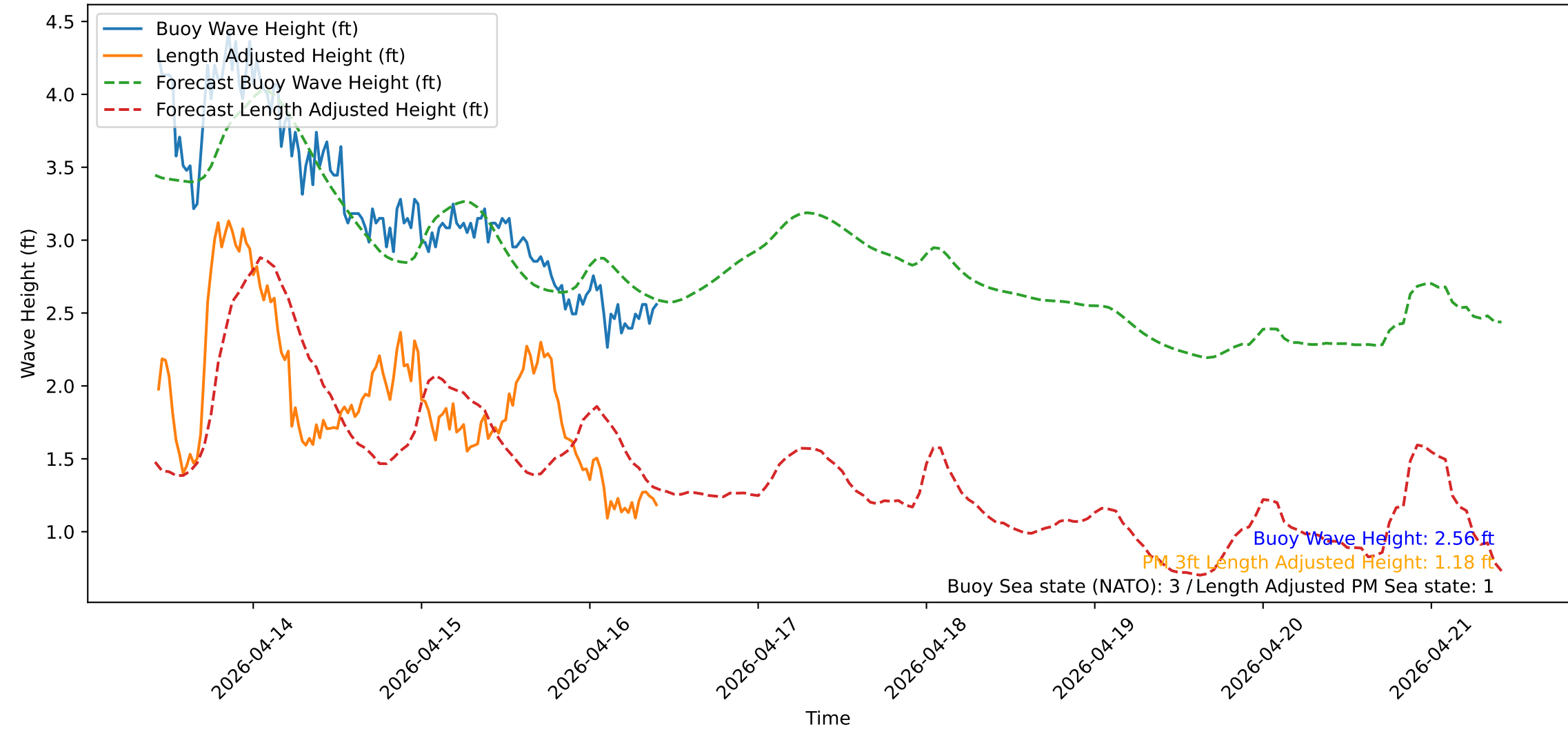
Wave Heights over Time for Red Beach at 2026-04-16 10:10:50
