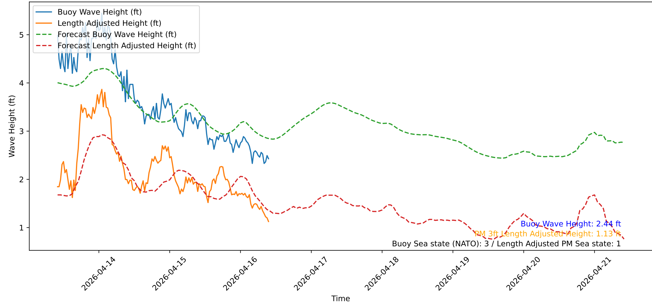
Wave Heights over Time for Oceanside Harbor at 2026-04-16 10:10:31
