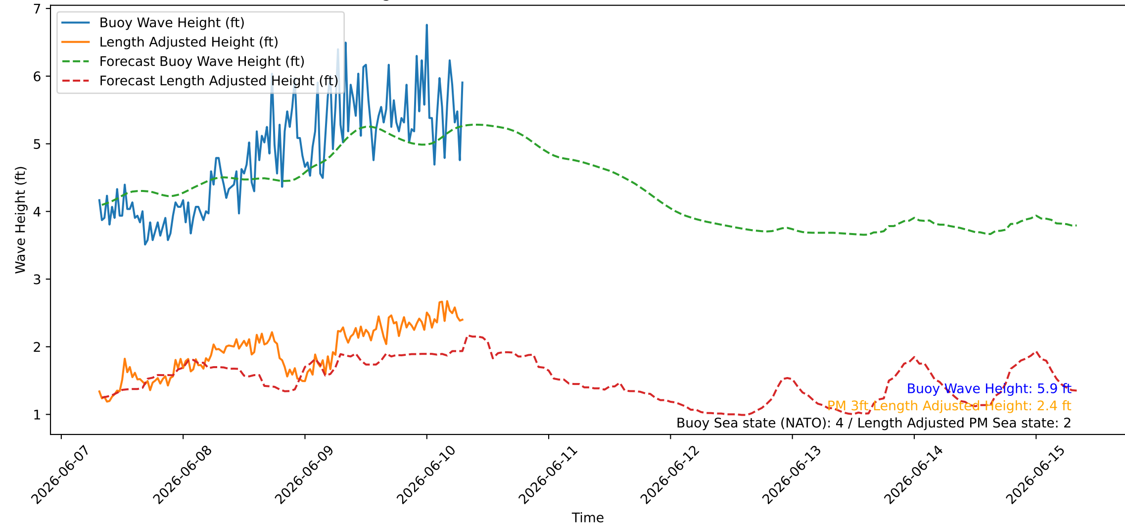
Wave Heights over Time for Oceanside Harbor at 2026-06-10 07:40:26
