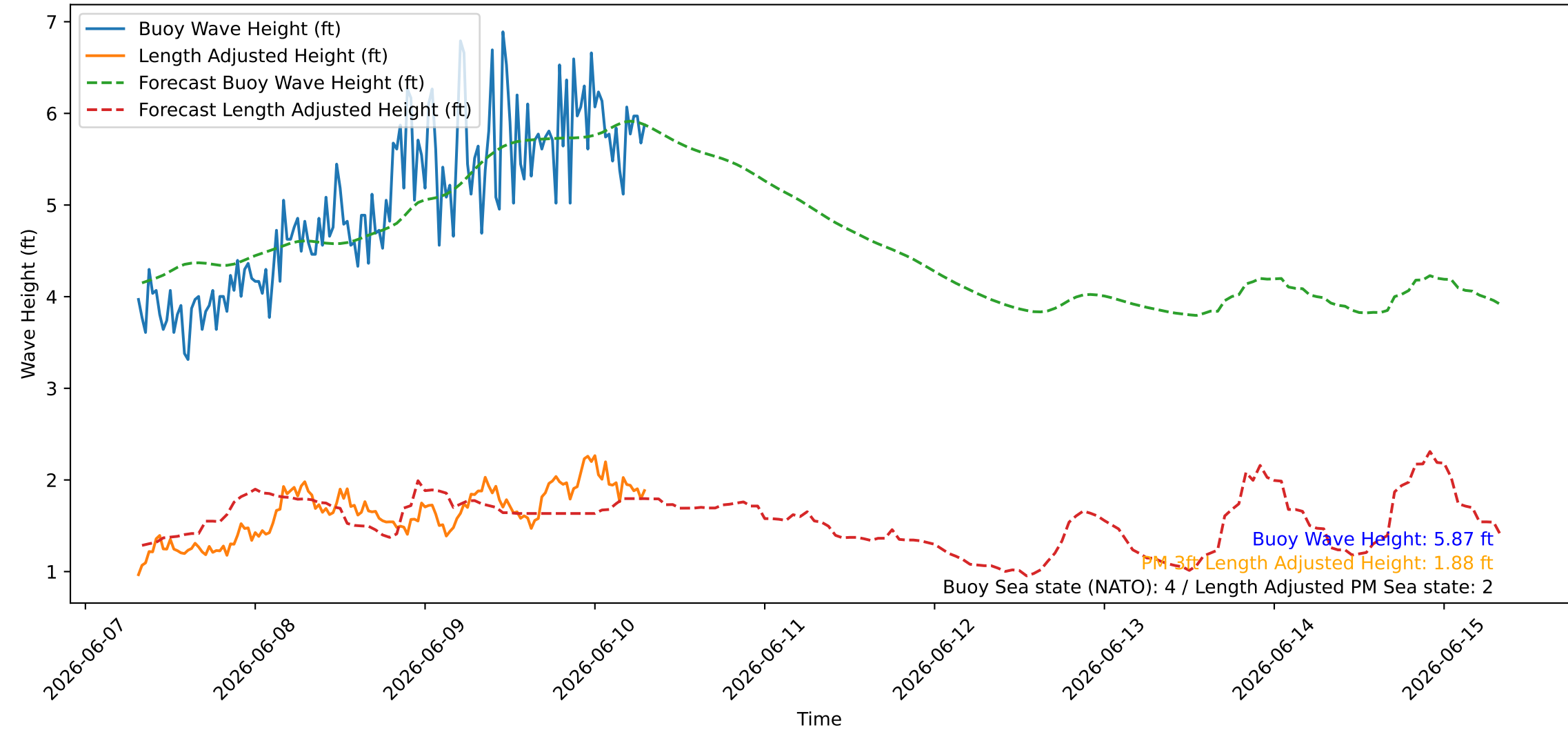
Wave Heights over Time for Green Beach at 2026-06-10 07:41:10
