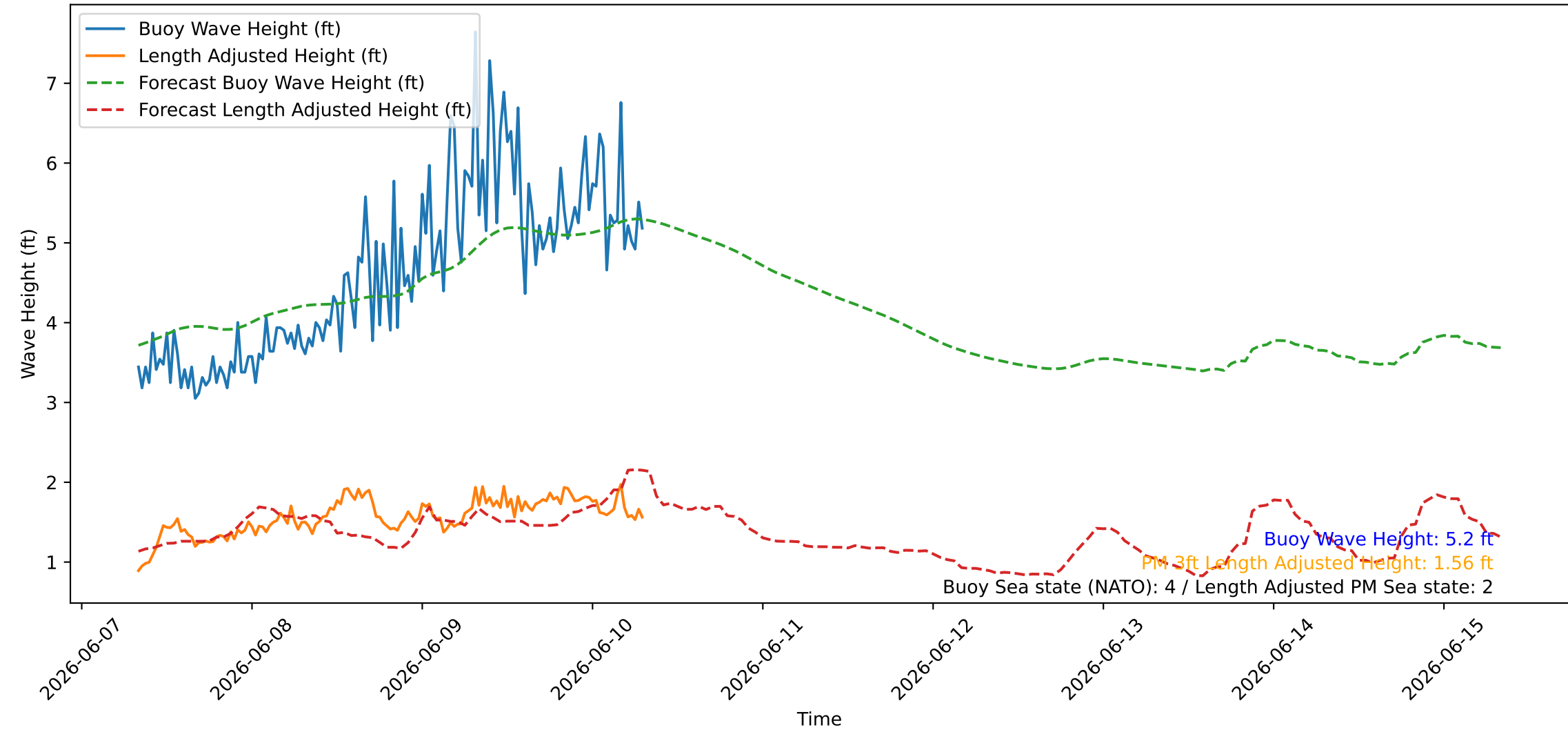
Wave Heights over Time for Red Beach at 2026-06-10 07:40:46
