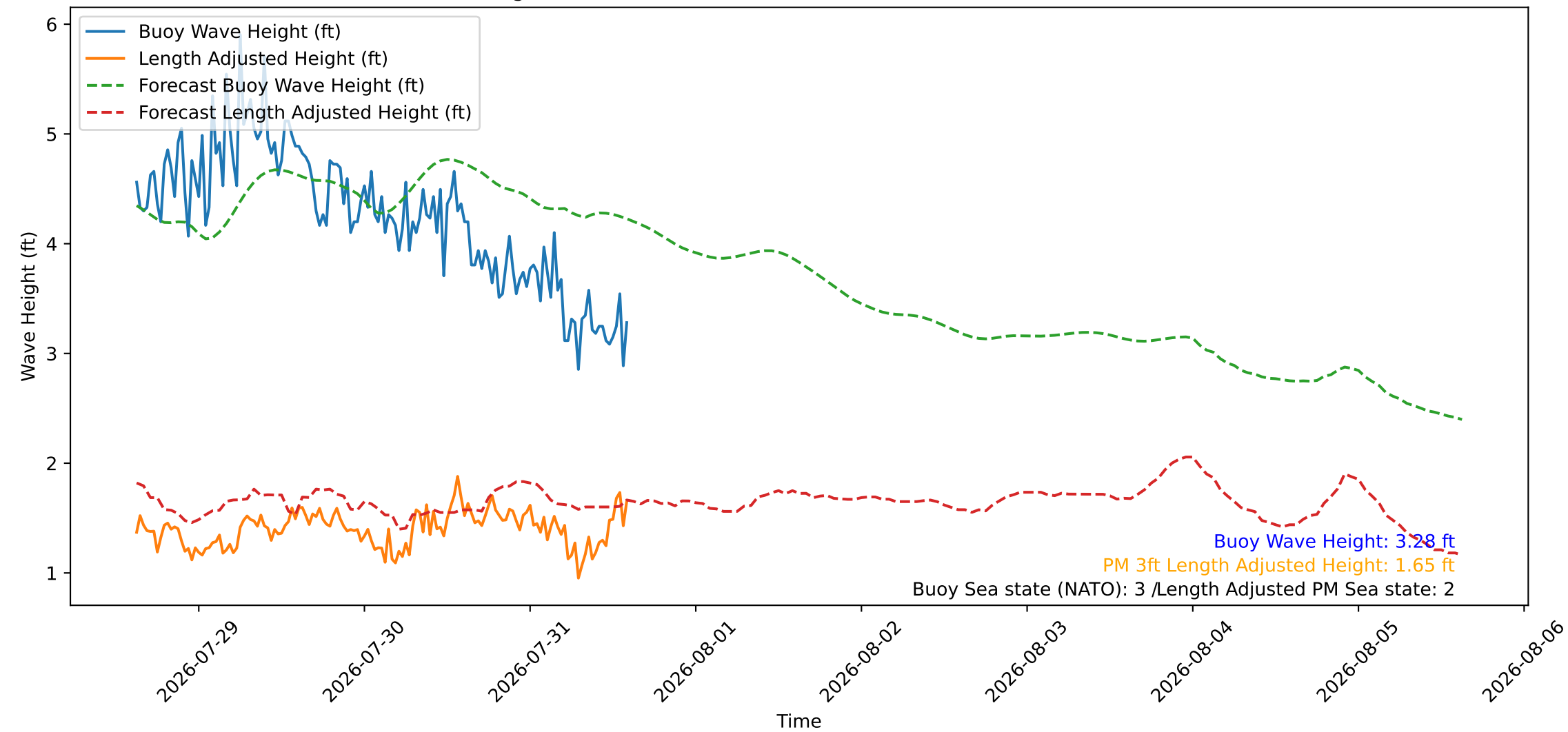
Wave Heights over Time for Oceanside Harbor at 2026-07-31 15:00:27
