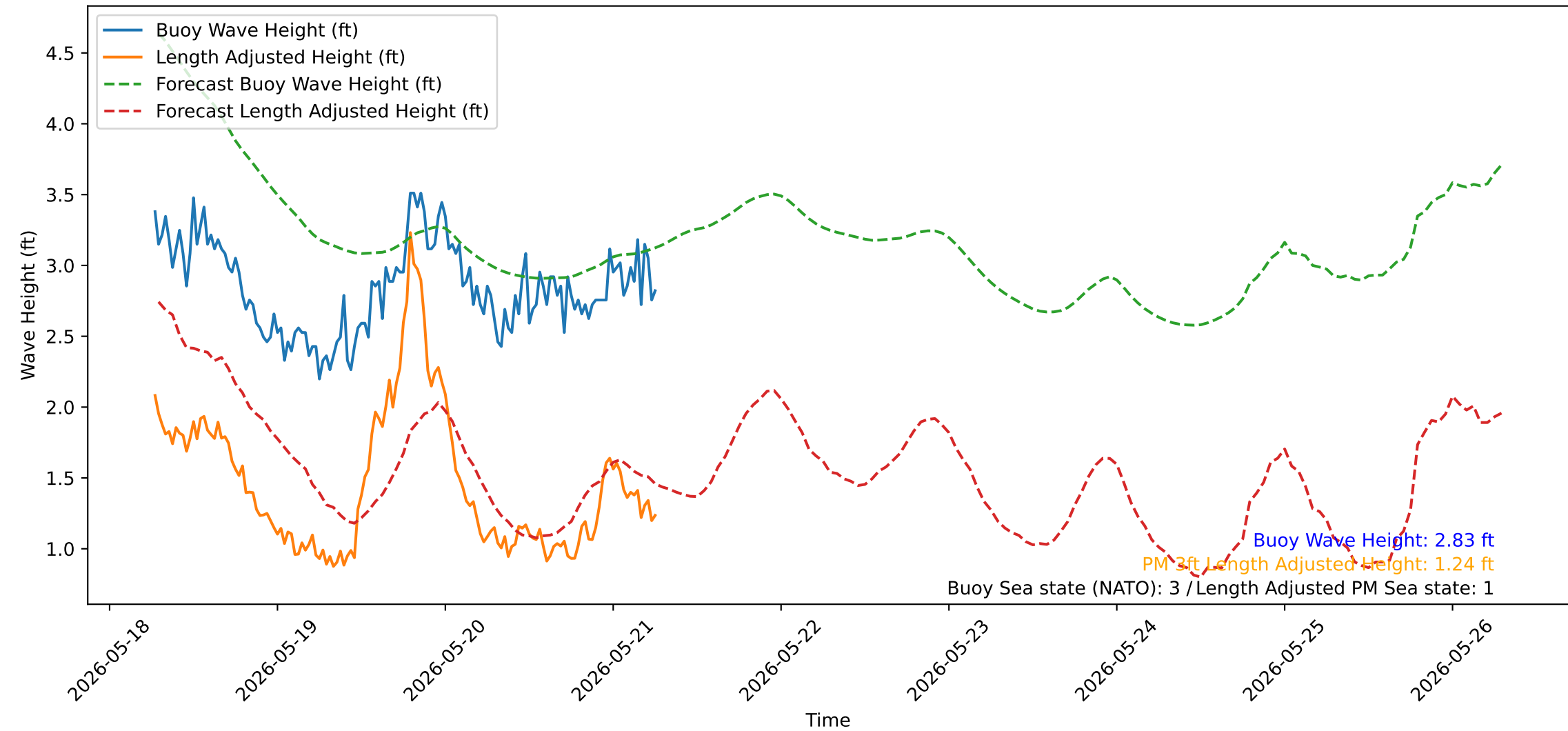
Wave Heights over Time for Oceanside Harbor at 2026-05-21 06:40:31
