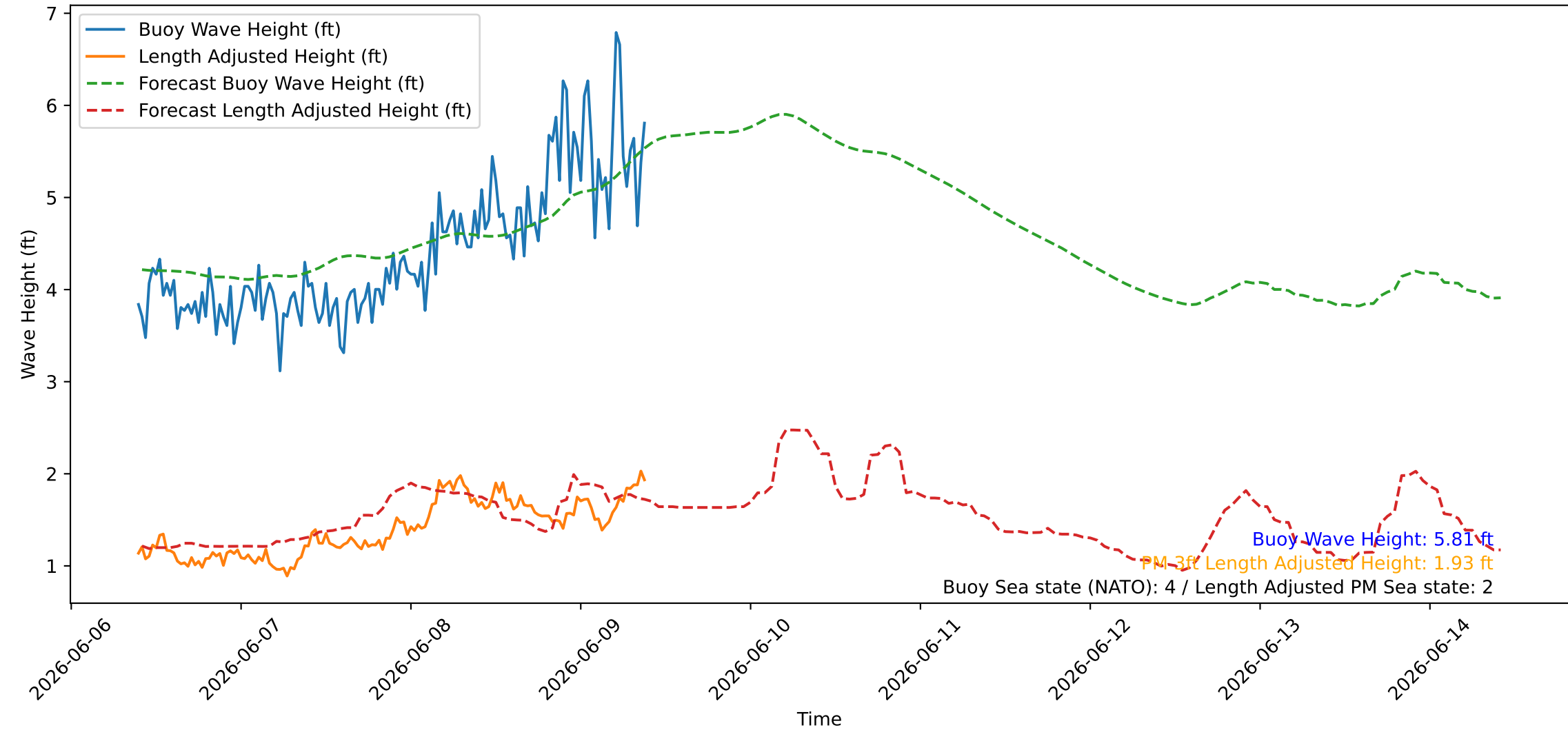
Wave Heights over Time for Green Beach at 2026-06-09 09:41:08
