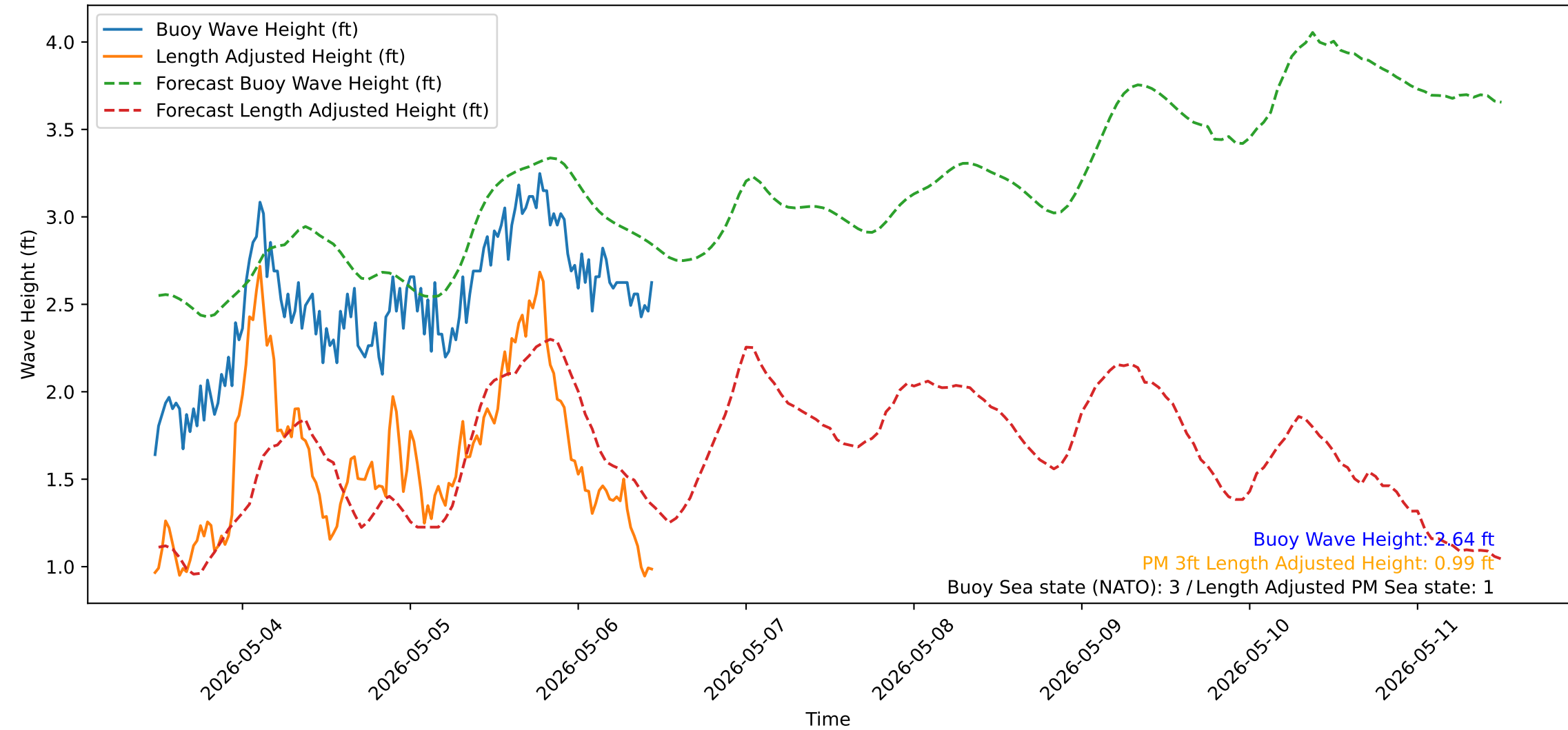
Wave Heights over Time for Oceanside Harbor at 2026-05-06 11:30:33
