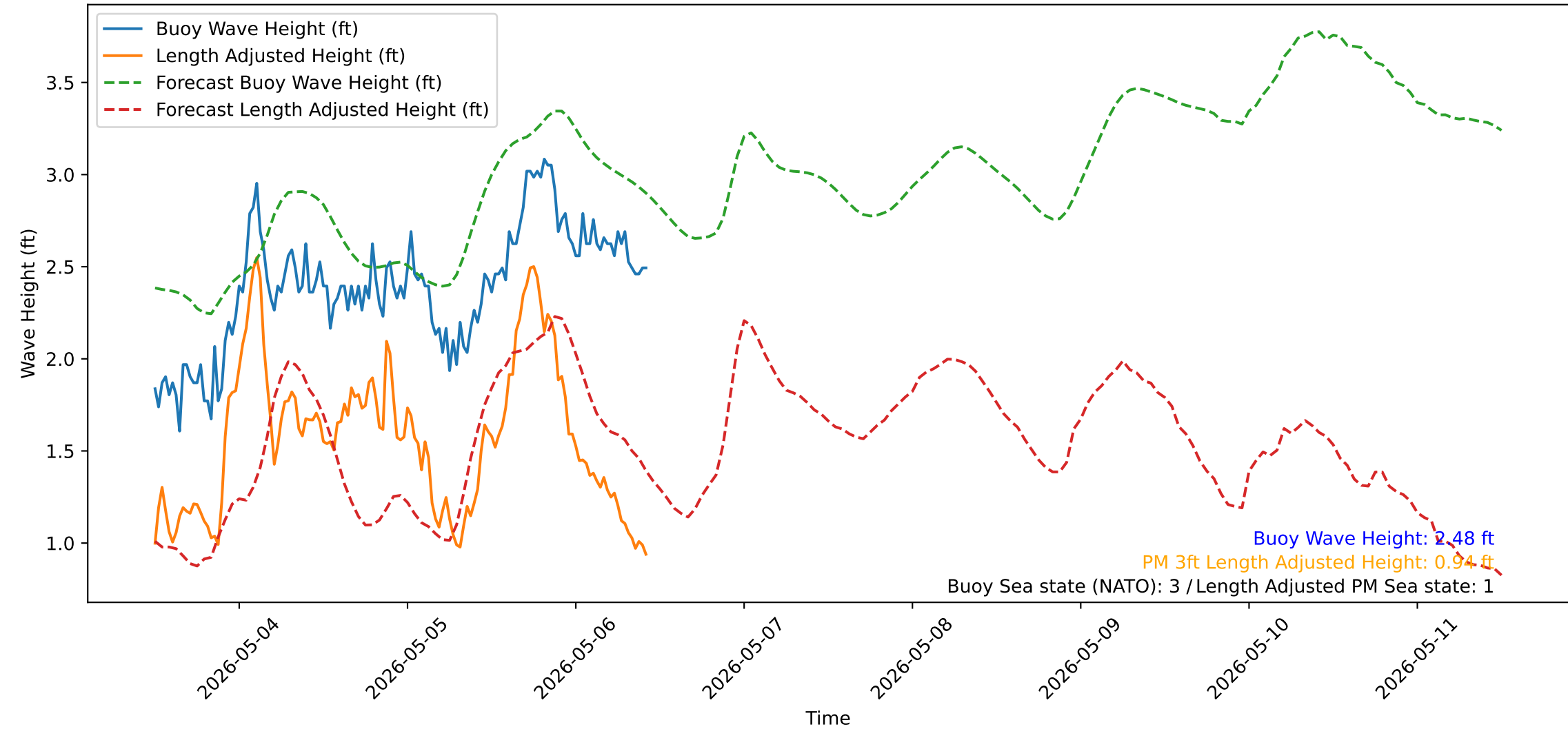
Wave Heights over Time for Red Beach at 2026-05-06 11:30:52
