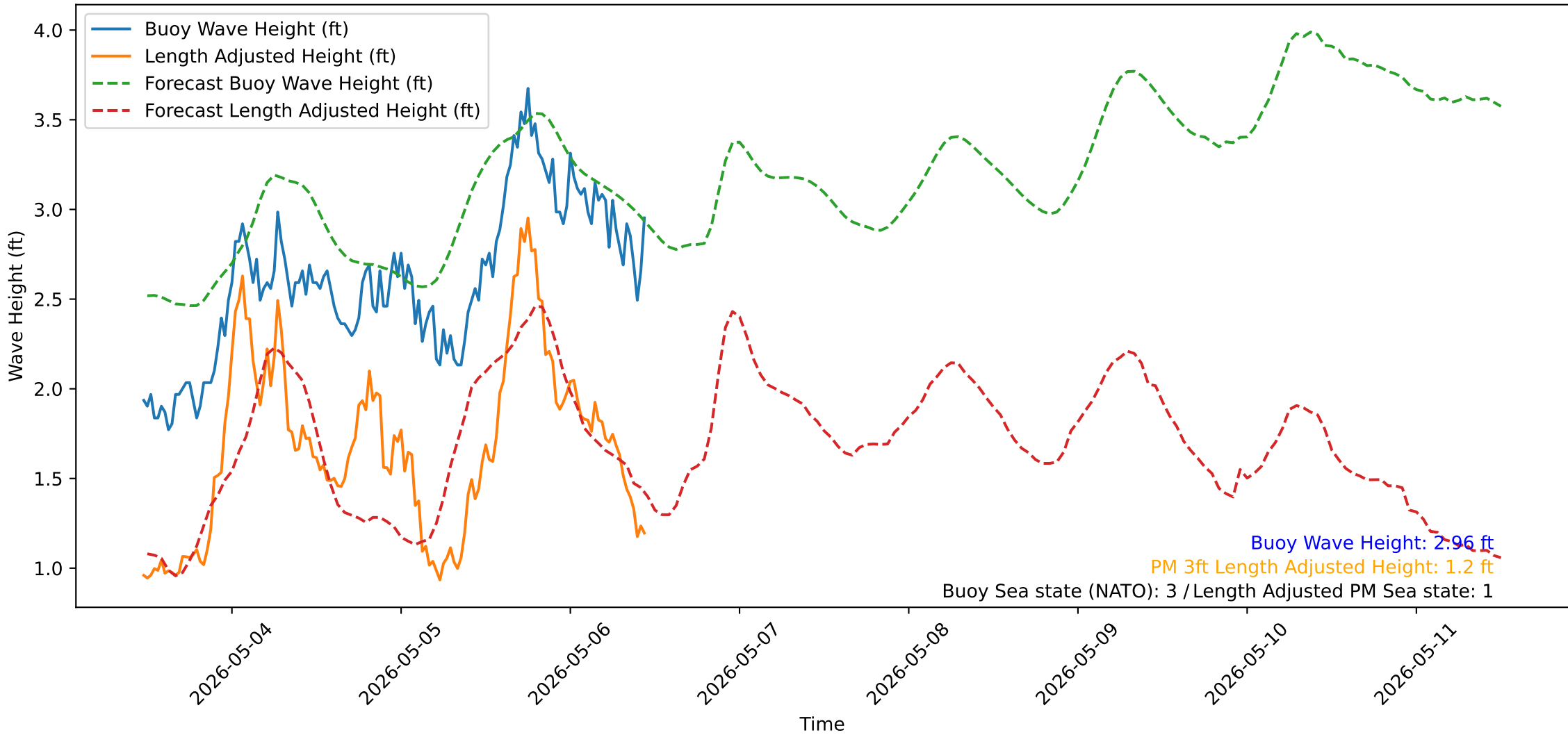
Wave Heights over Time for Green Beach at 2026-05-06 11:31:14
