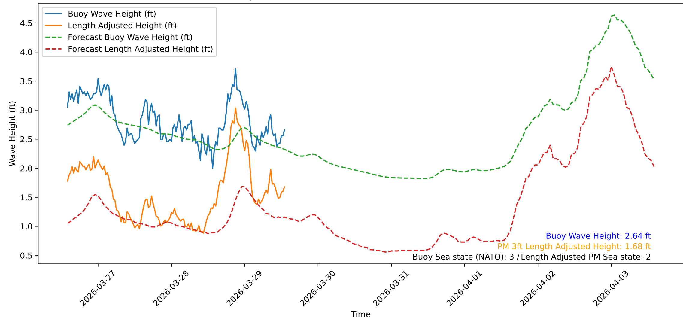
Wave Heights over Time for Green Beach at 2026-03-29 13:51:10
