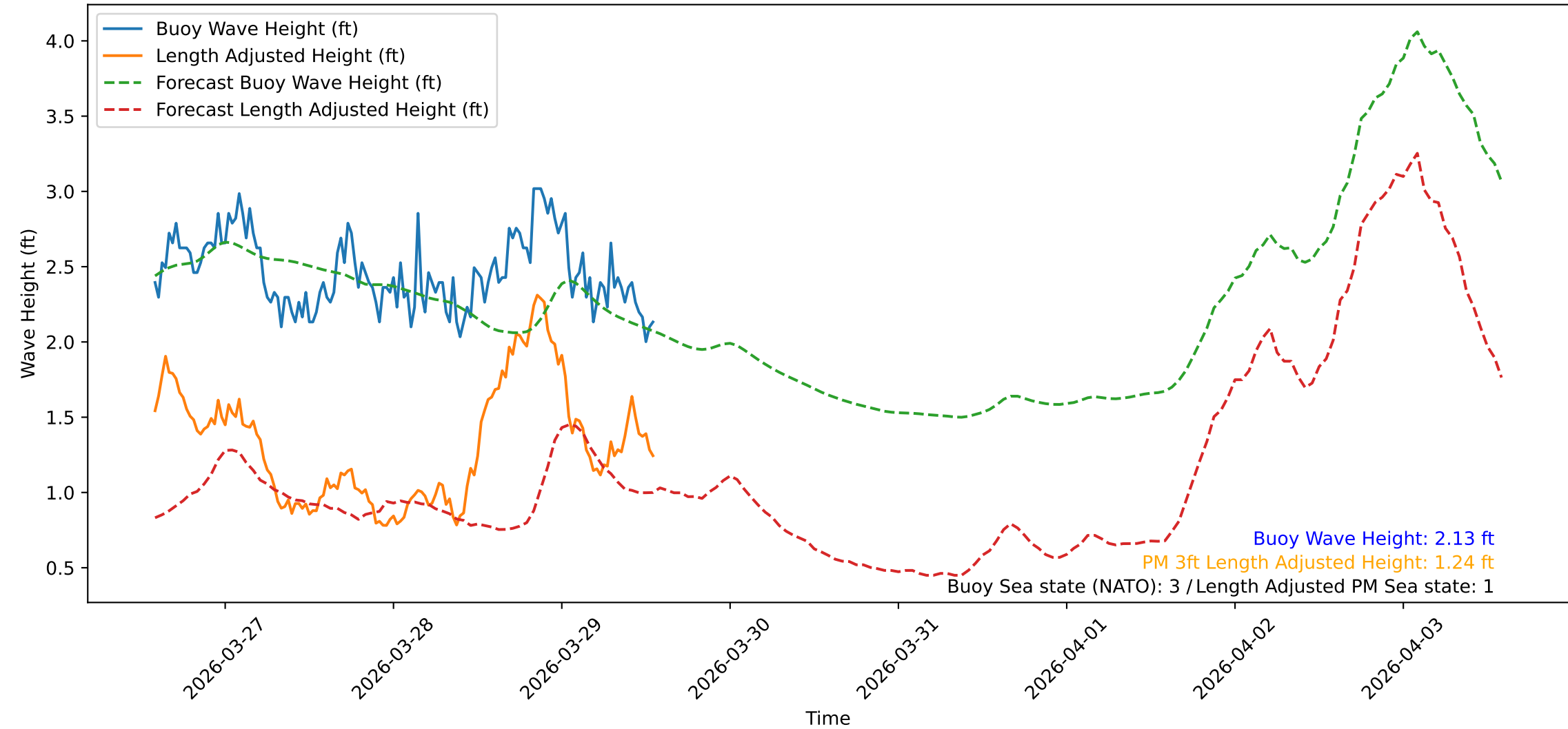
Wave Heights over Time for Red Beach at 2026-03-29 13:50:48
