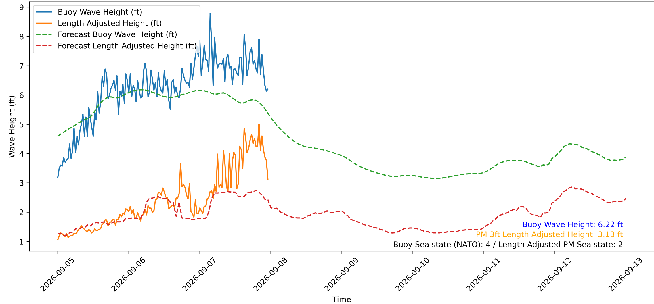
Wave Heights over Time for Green Beach at 2026-09-07 23:41:12
