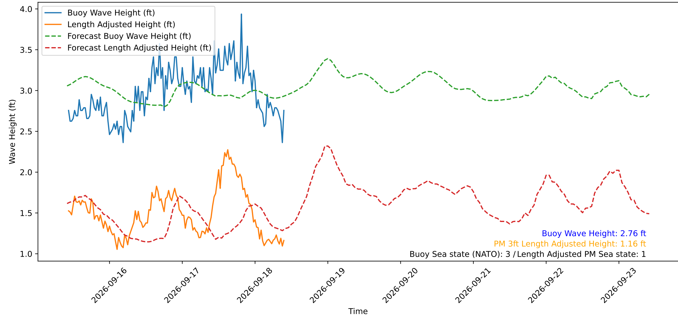
Wave Heights over Time for Oceanside Harbor at 2026-09-18 10:20:30
