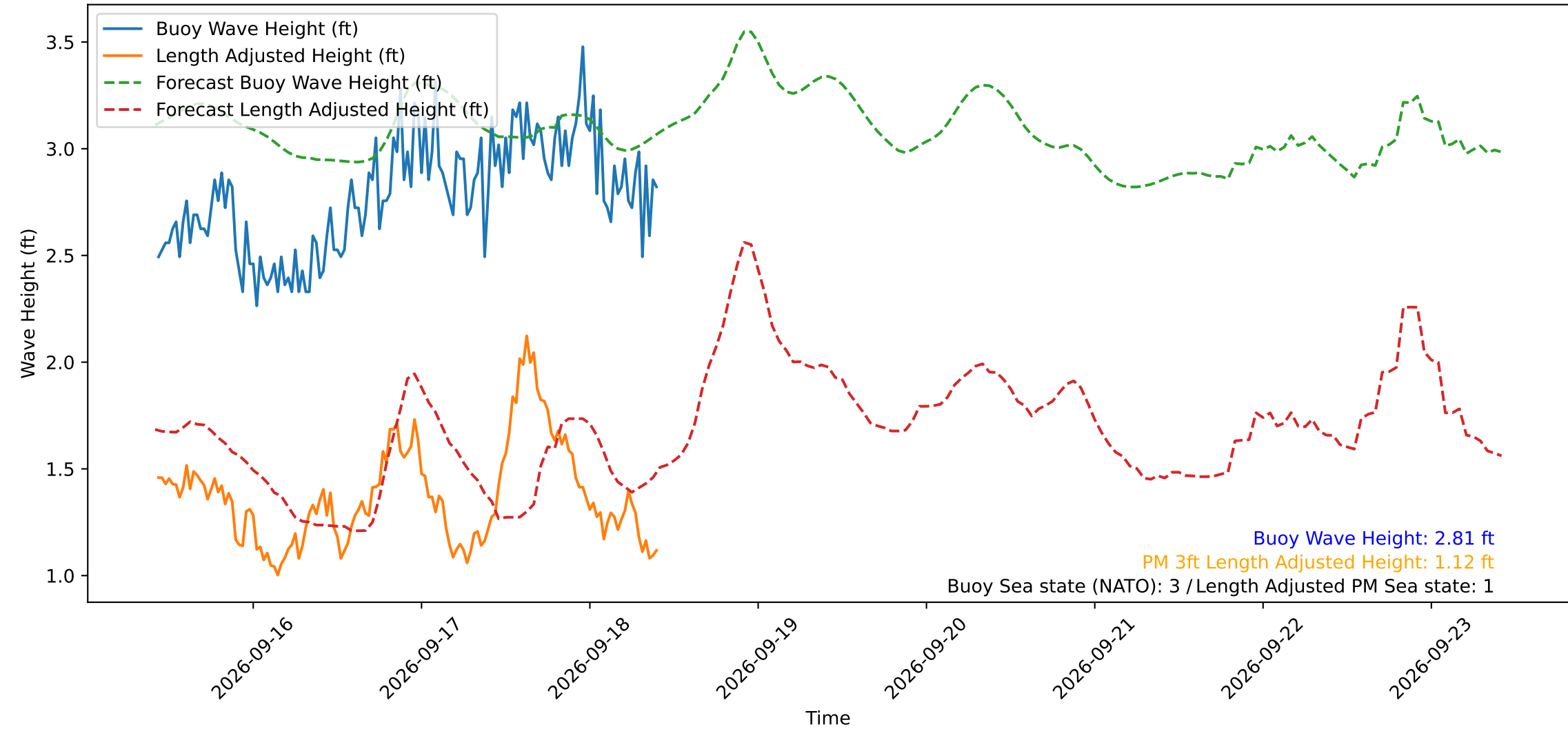
Wave Heights over Time for Green Beach at 2026-09-18 10:21:18
