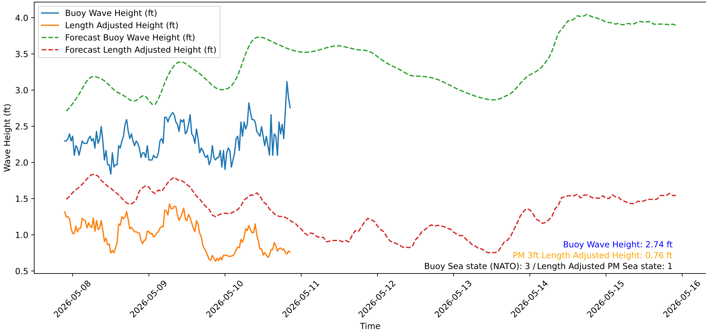
Wave Heights over Time for Green Beach at 2026-05-10 21:31:13
