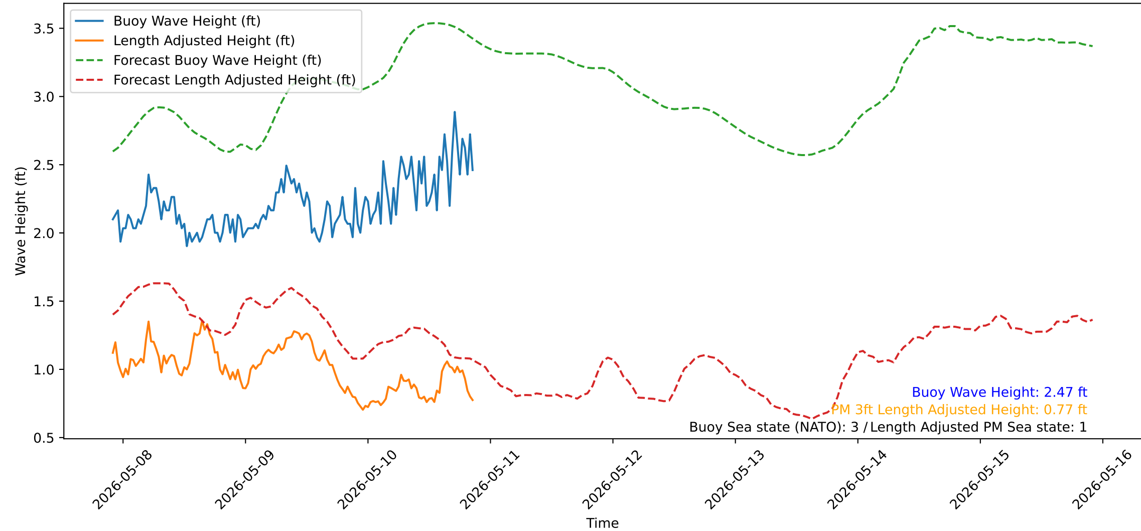
Wave Heights over Time for Red Beach at 2026-05-10 21:30:51
