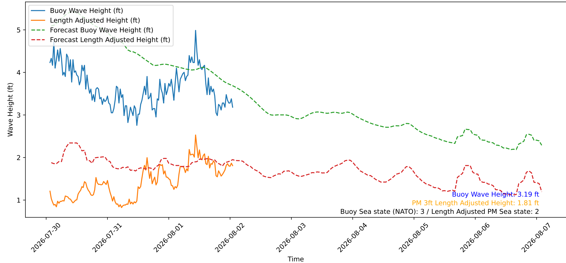
Wave Heights over Time for Green Beach at 2026-08-02 01:41:09
