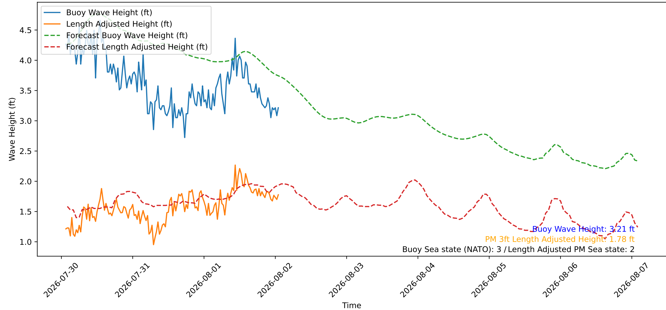
Wave Heights over Time for Oceanside Harbor at 2026-08-02 01:40:26
