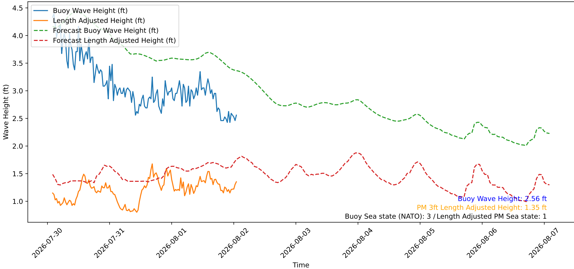
Wave Heights over Time for Red Beach at 2026-08-02 01:40:46
