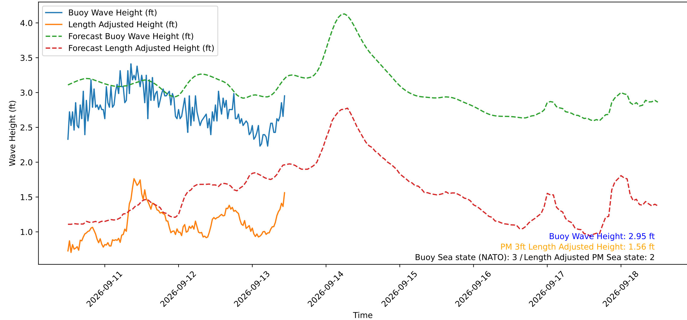
Wave Heights over Time for Red Beach at 2026-09-13 11:30:50
