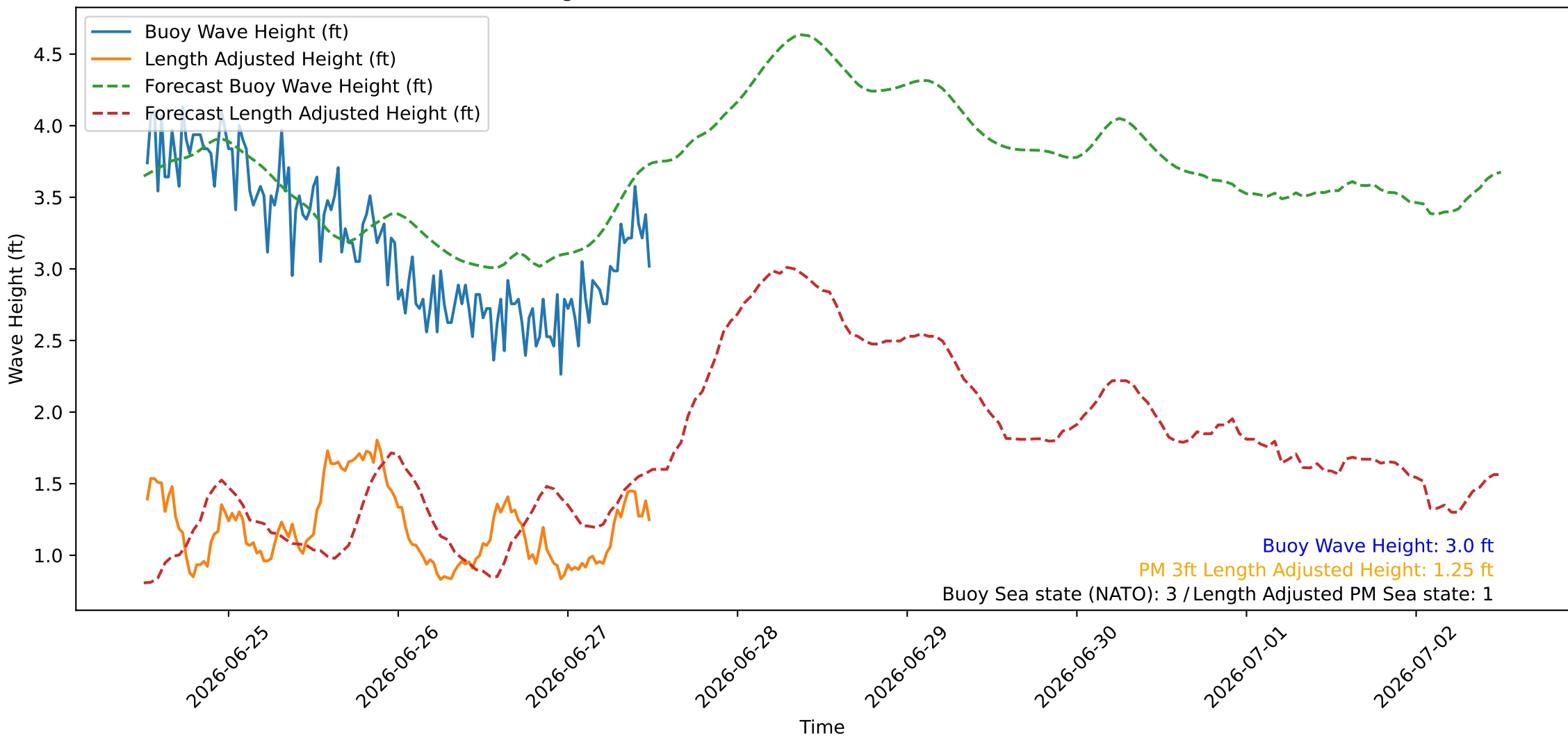
Wave Heights over Time for Green Beach at 2026-06-27 12:21:09
