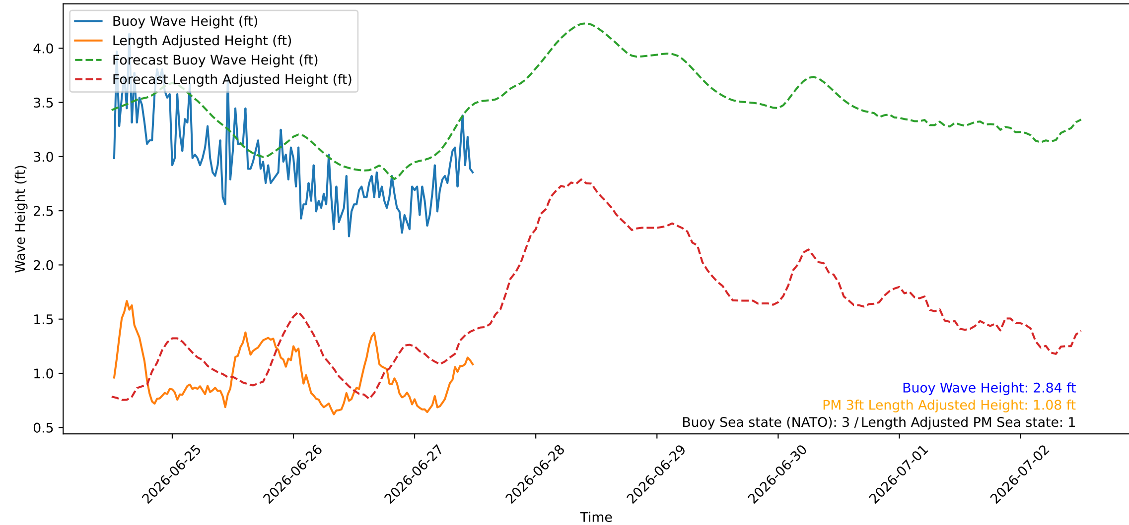
Wave Heights over Time for Red Beach at 2026-06-27 12:20:47
