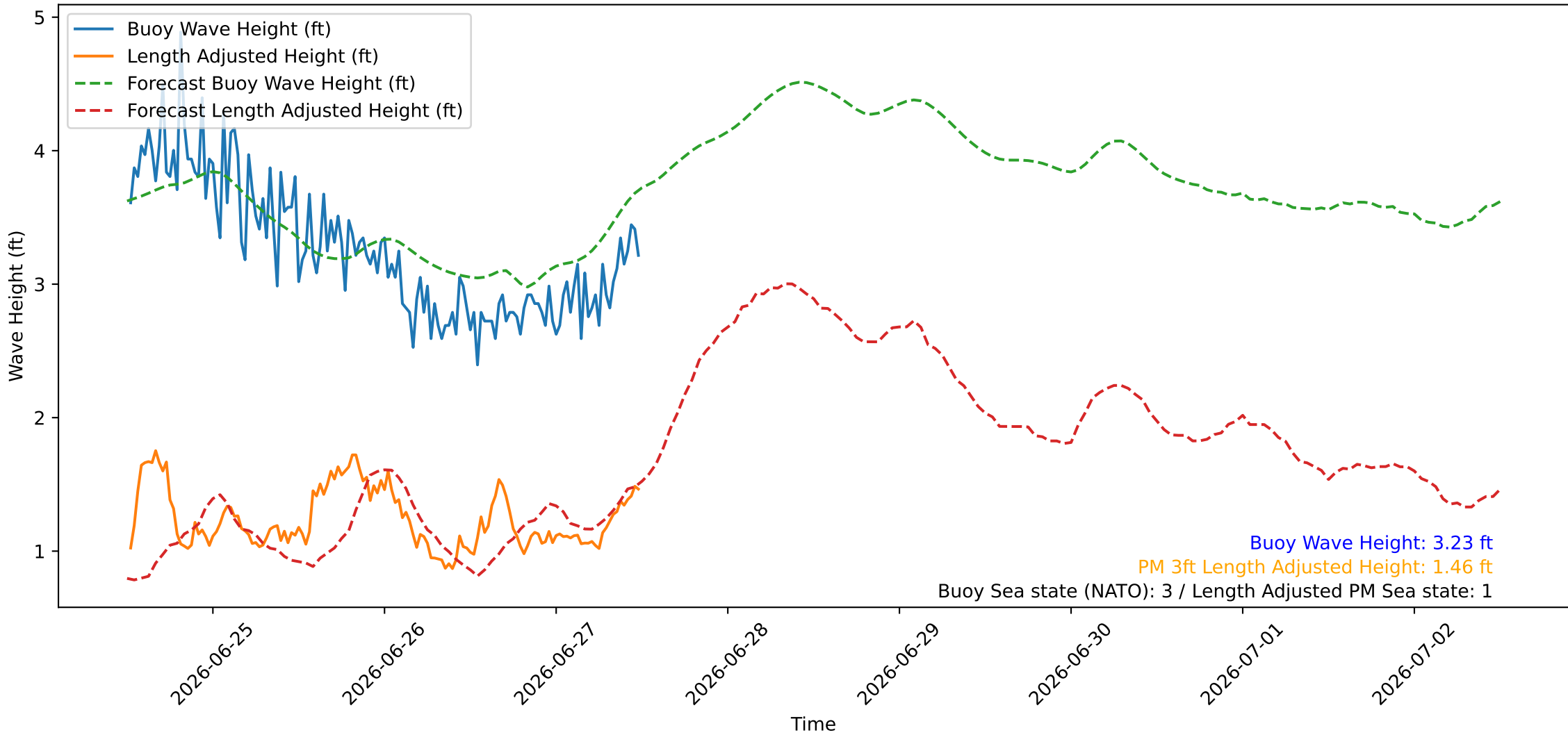
Wave Heights over Time for Oceanside Harbor at 2026-06-27 12:20:26
