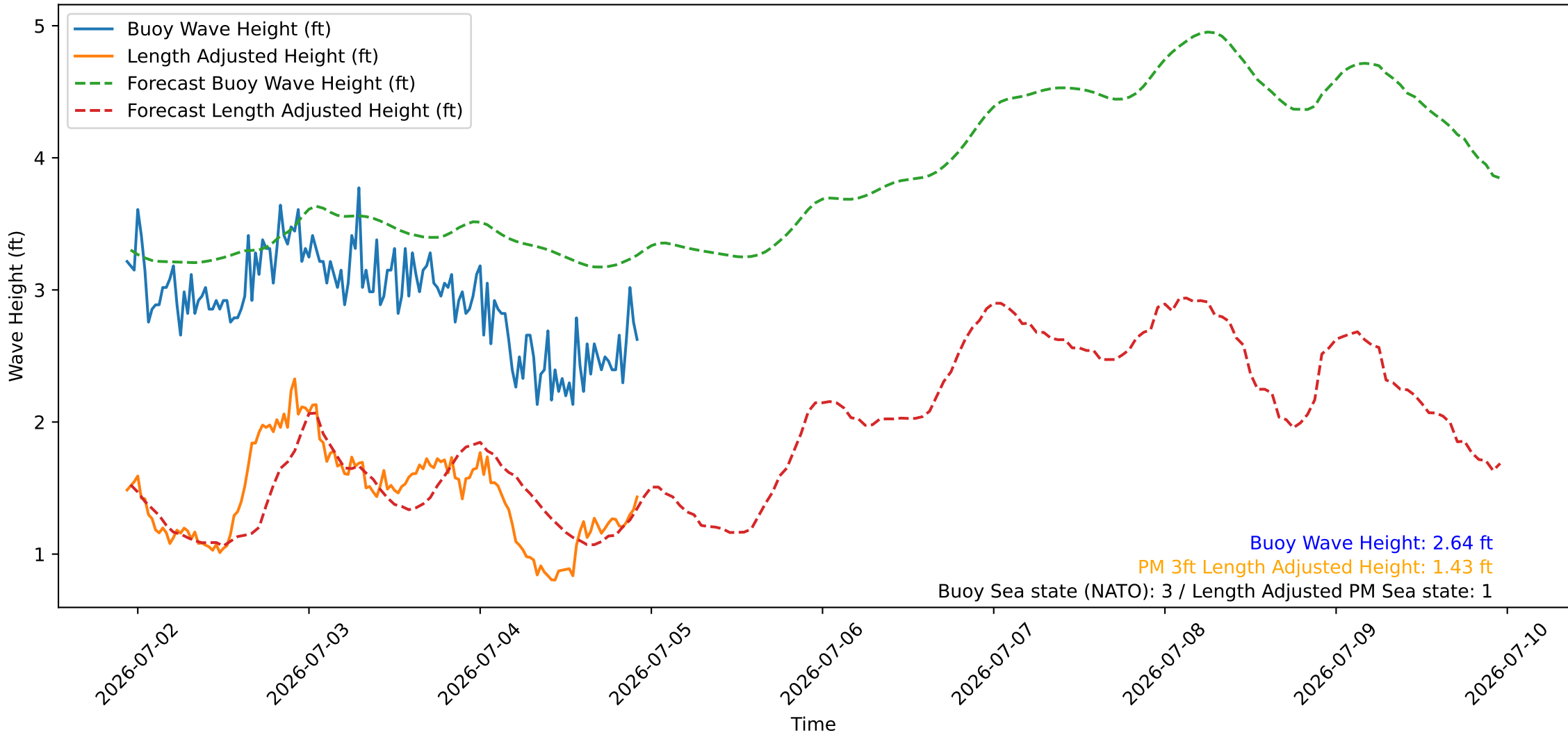
Wave Heights over Time for Oceanside Harbor at 2026-07-04 22:40:25
