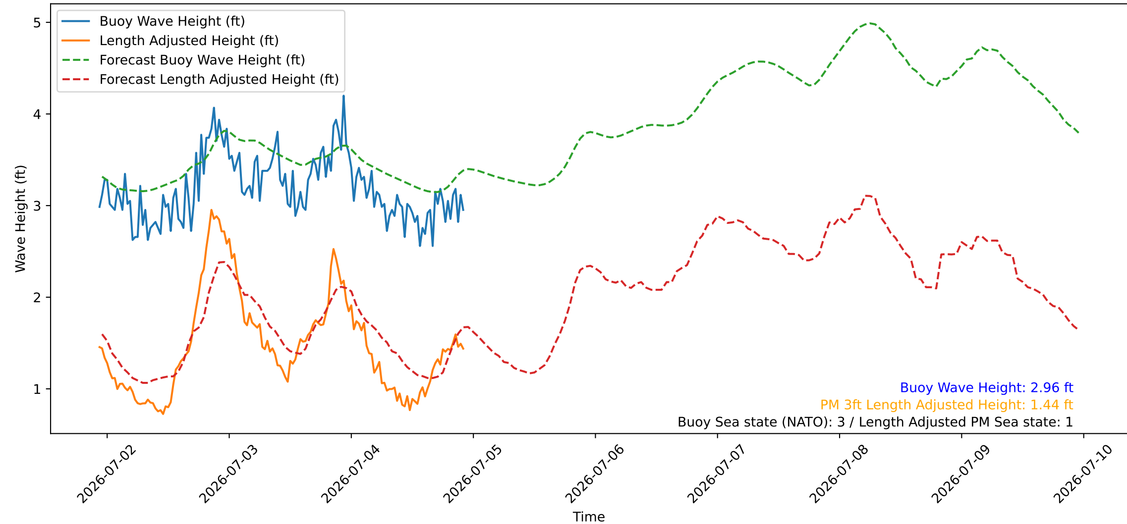
Wave Heights over Time for Green Beach at 2026-07-04 22:41:08
