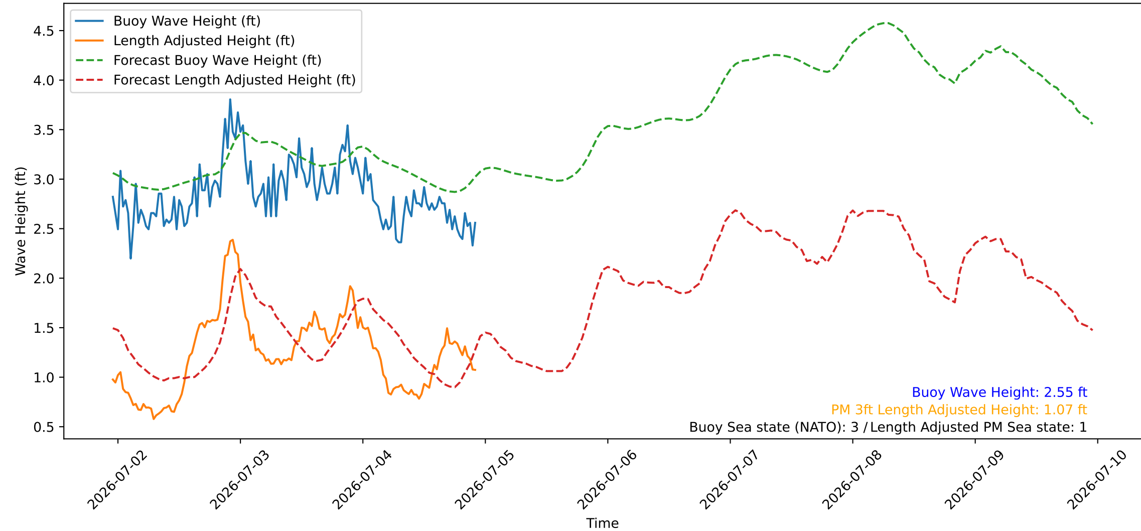
Wave Heights over Time for Red Beach at 2026-07-04 22:40:45
