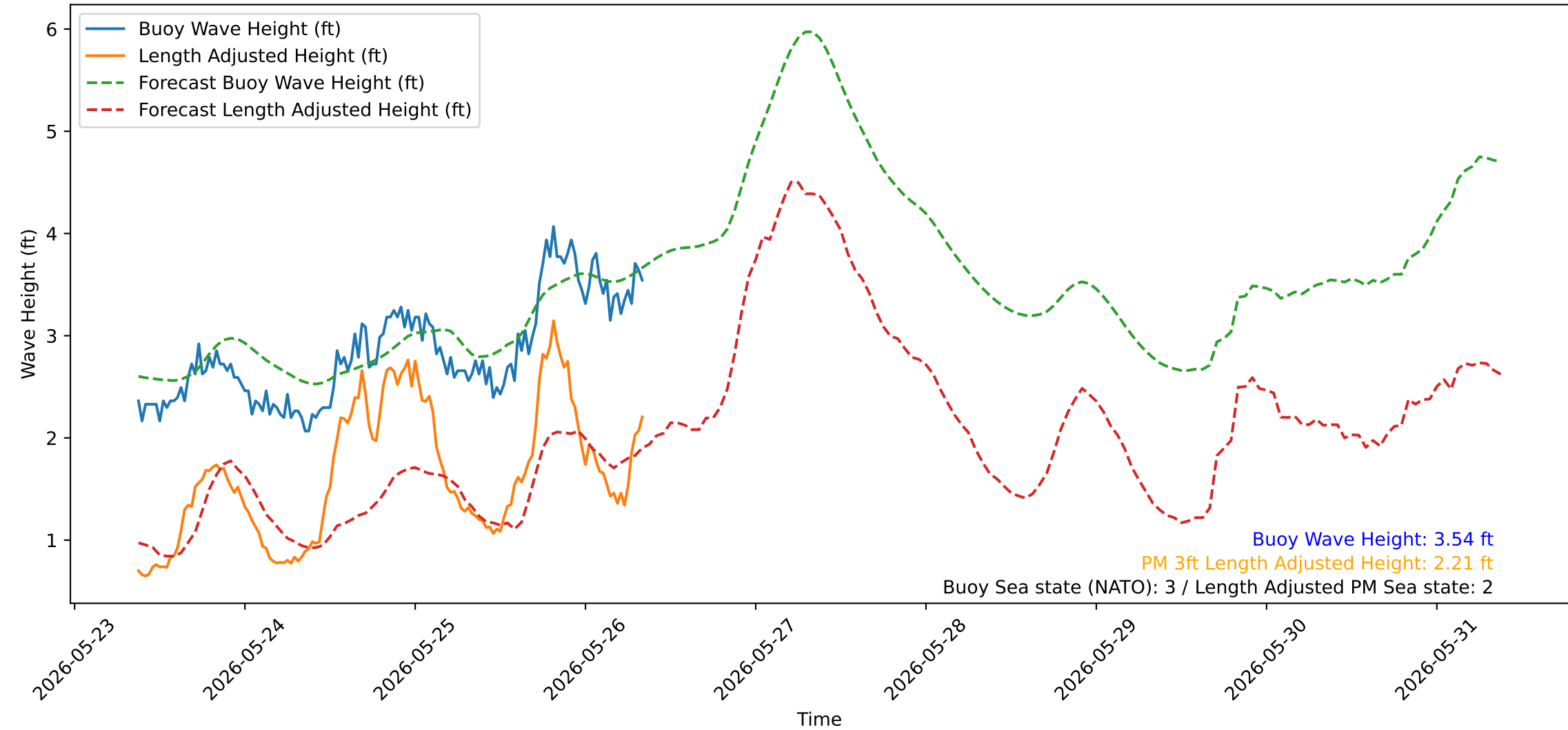
Wave Heights over Time for Green Beach at 2026-05-26 09:01:10
