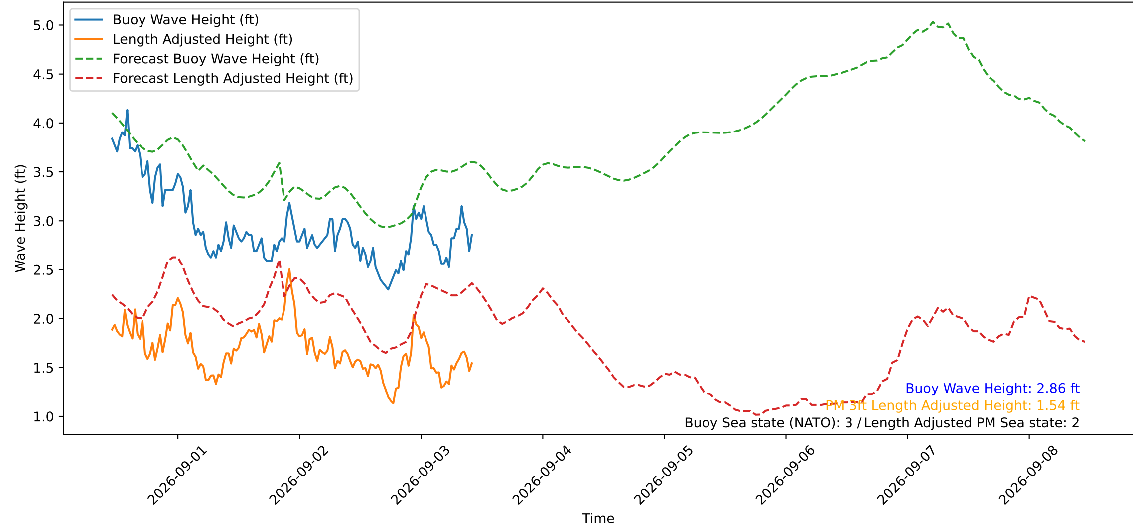
Wave Heights over Time for Red Beach at 2026-09-03 10:40:50
