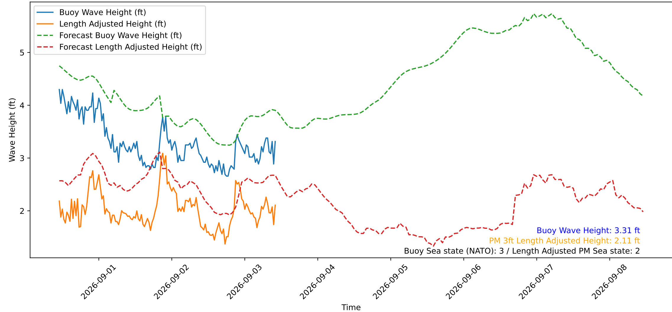
Wave Heights over Time for Green Beach at 2026-09-03 10:41:13
