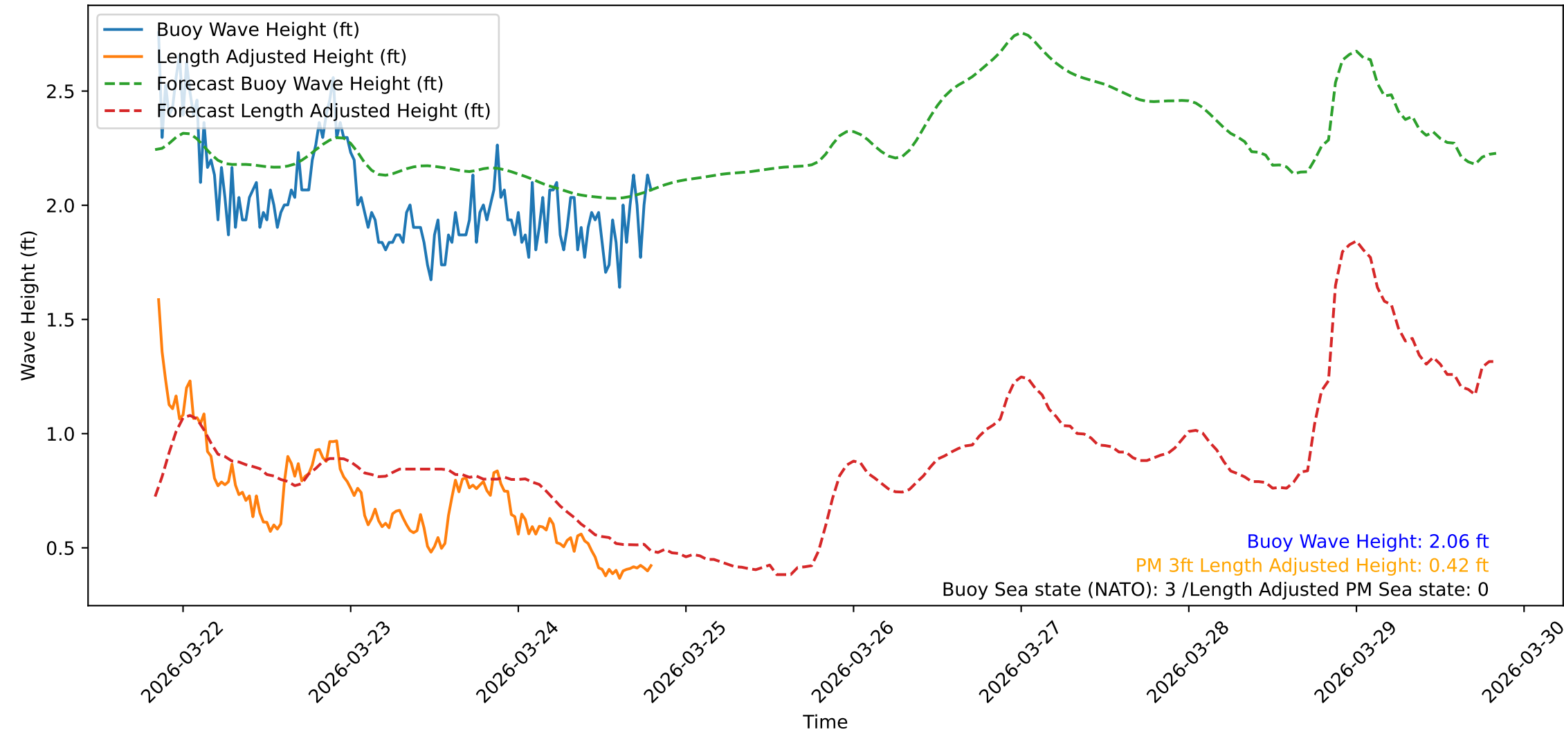
Wave Heights over Time for Red Beach at 2026-03-24 20:00:46
