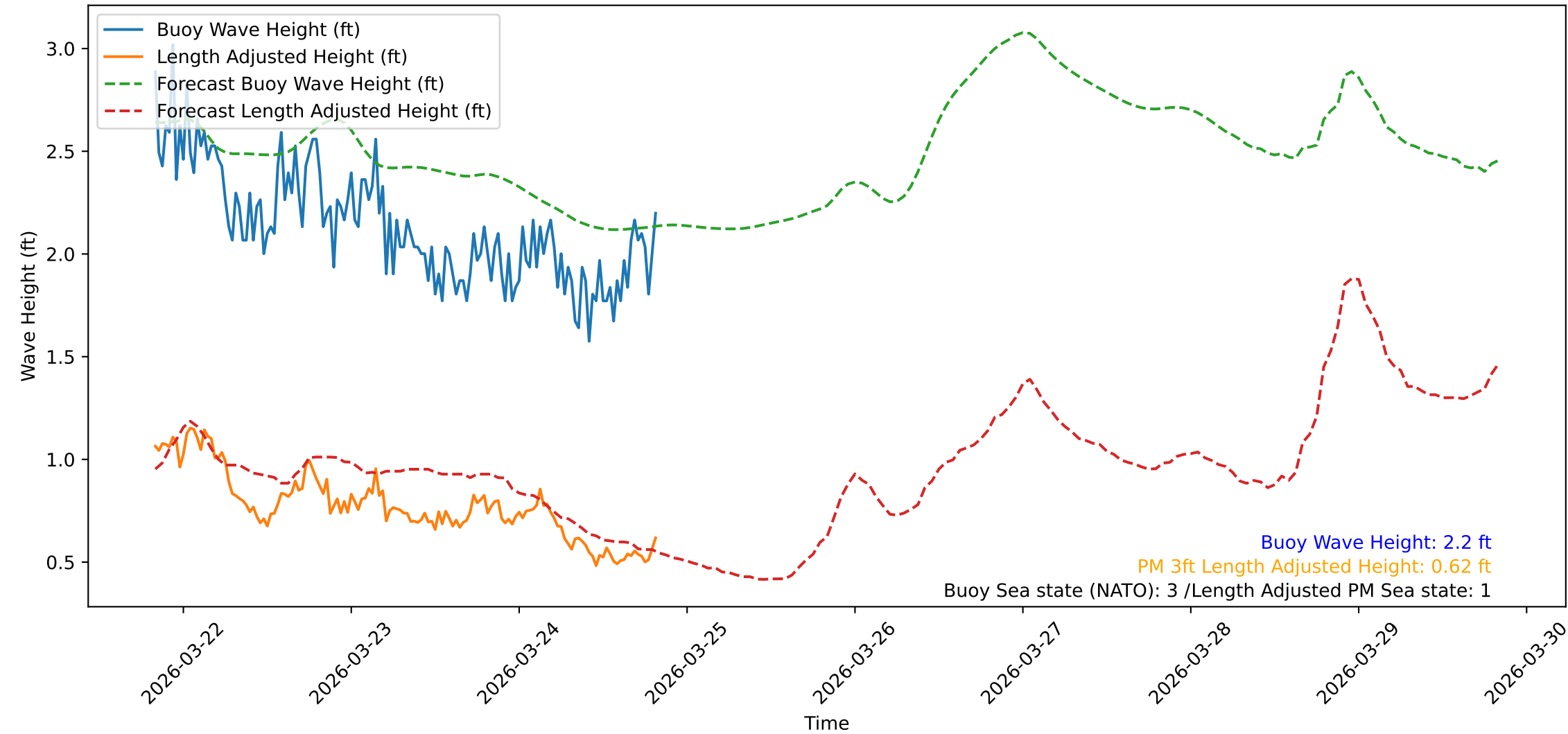
Wave Heights over Time for Oceanside Harbor at 2026-03-24 20:00:30
