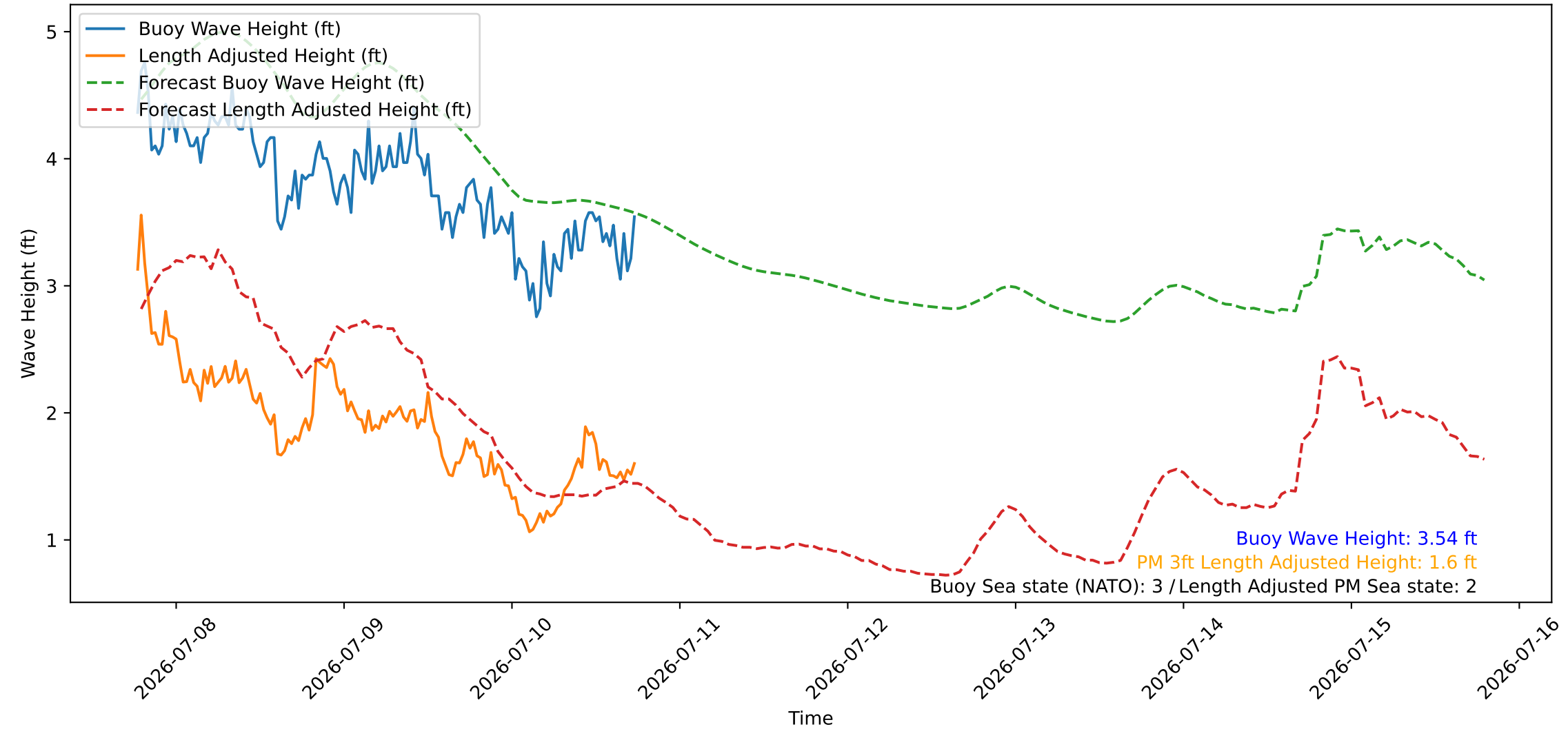
Wave Heights over Time for Green Beach at 2026-07-10 18:31:08
