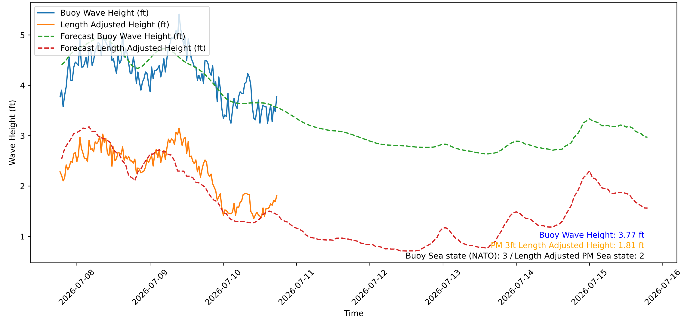
Wave Heights over Time for Oceanside Harbor at 2026-07-10 18:30:26
