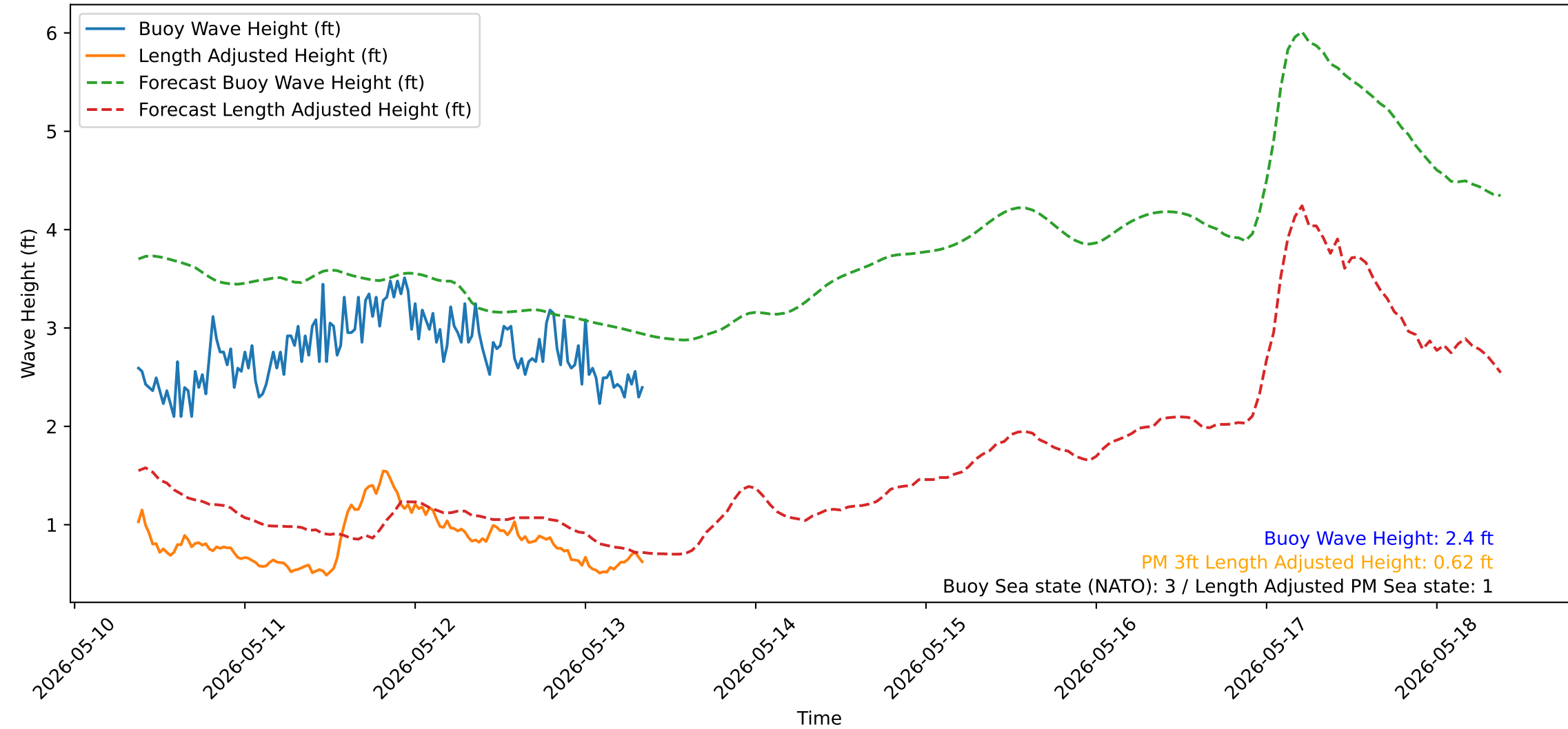
Wave Heights over Time for Green Beach at 2026-05-13 09:01:14
