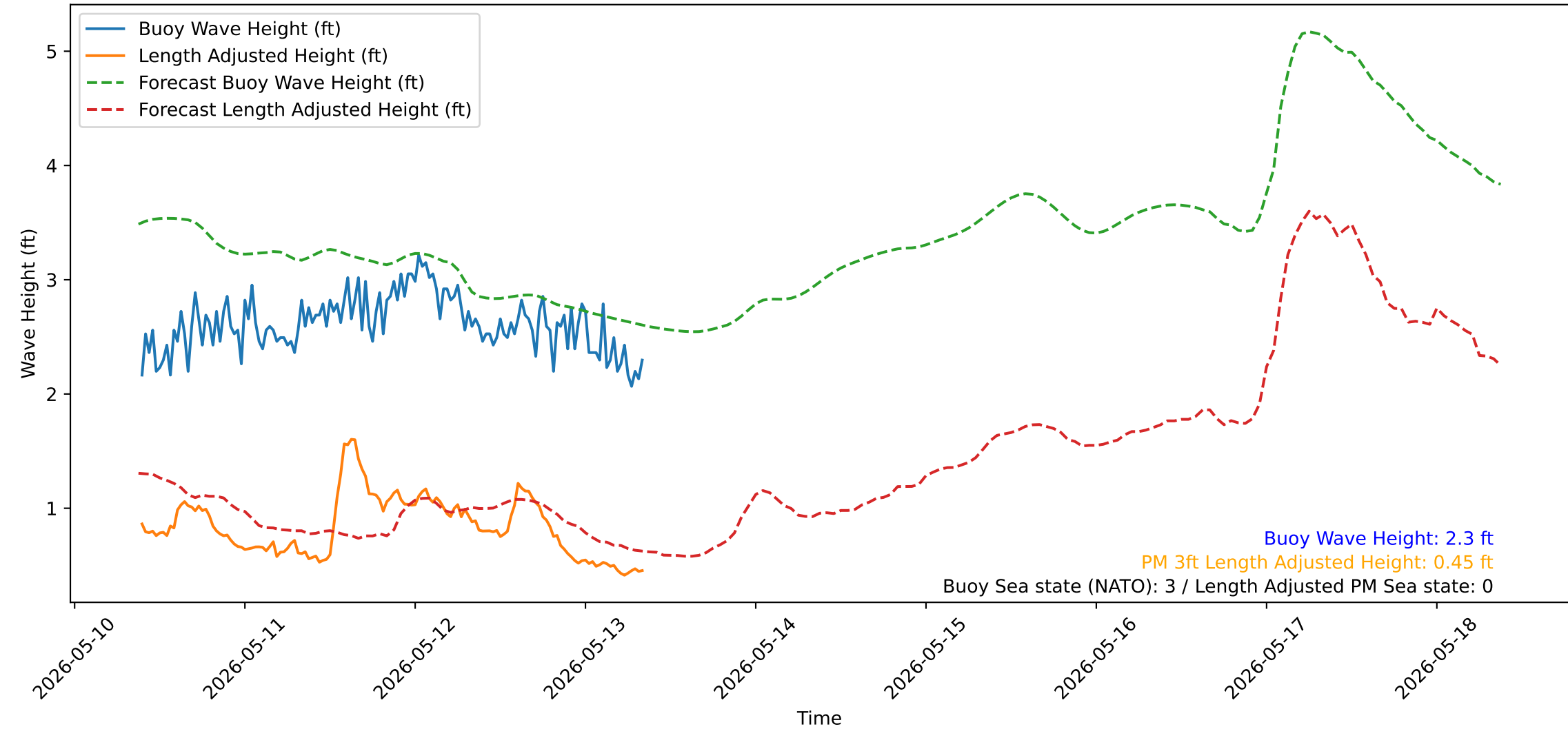
Wave Heights over Time for Red Beach at 2026-05-13 09:00:52
