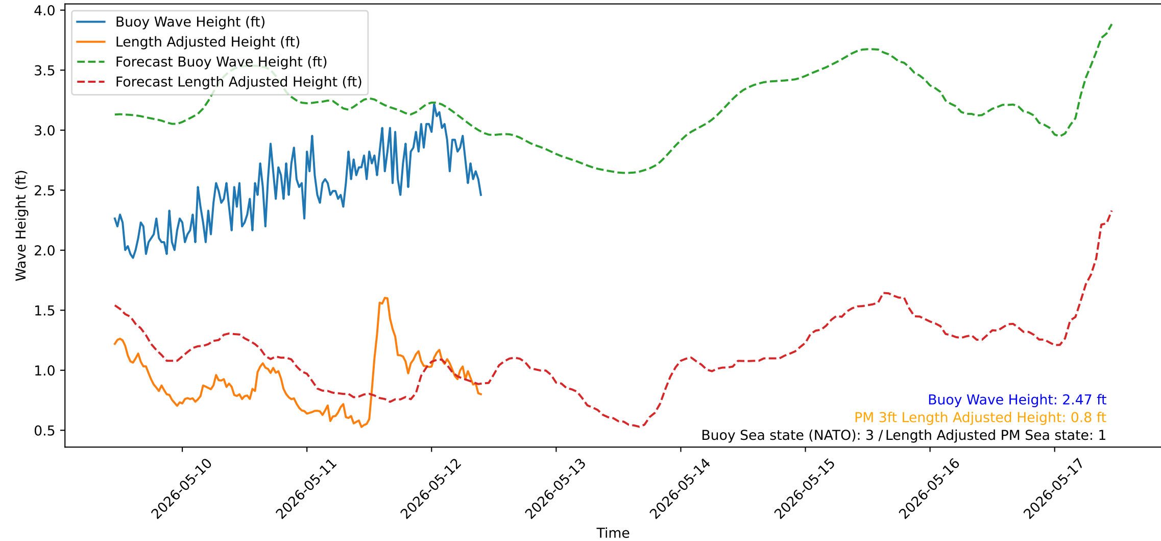
Wave Heights over Time for Red Beach at 2026-05-12 10:30:50
