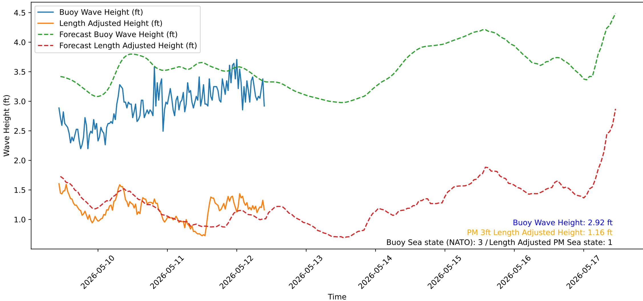
Wave Heights over Time for Oceanside Harbor at 2026-05-12 10:30:31
