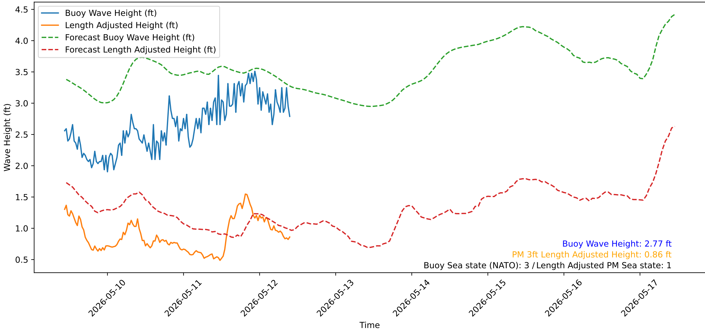
Wave Heights over Time for Green Beach at 2026-05-12 10:31:13
