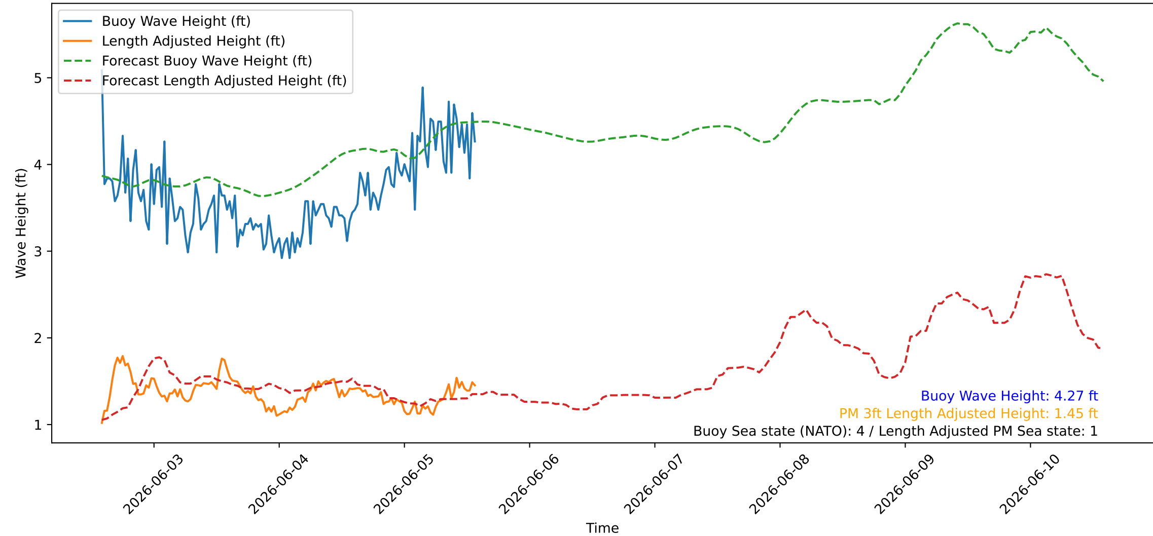
Wave Heights over Time for Oceanside Harbor at 2026-06-05 14:10:26
