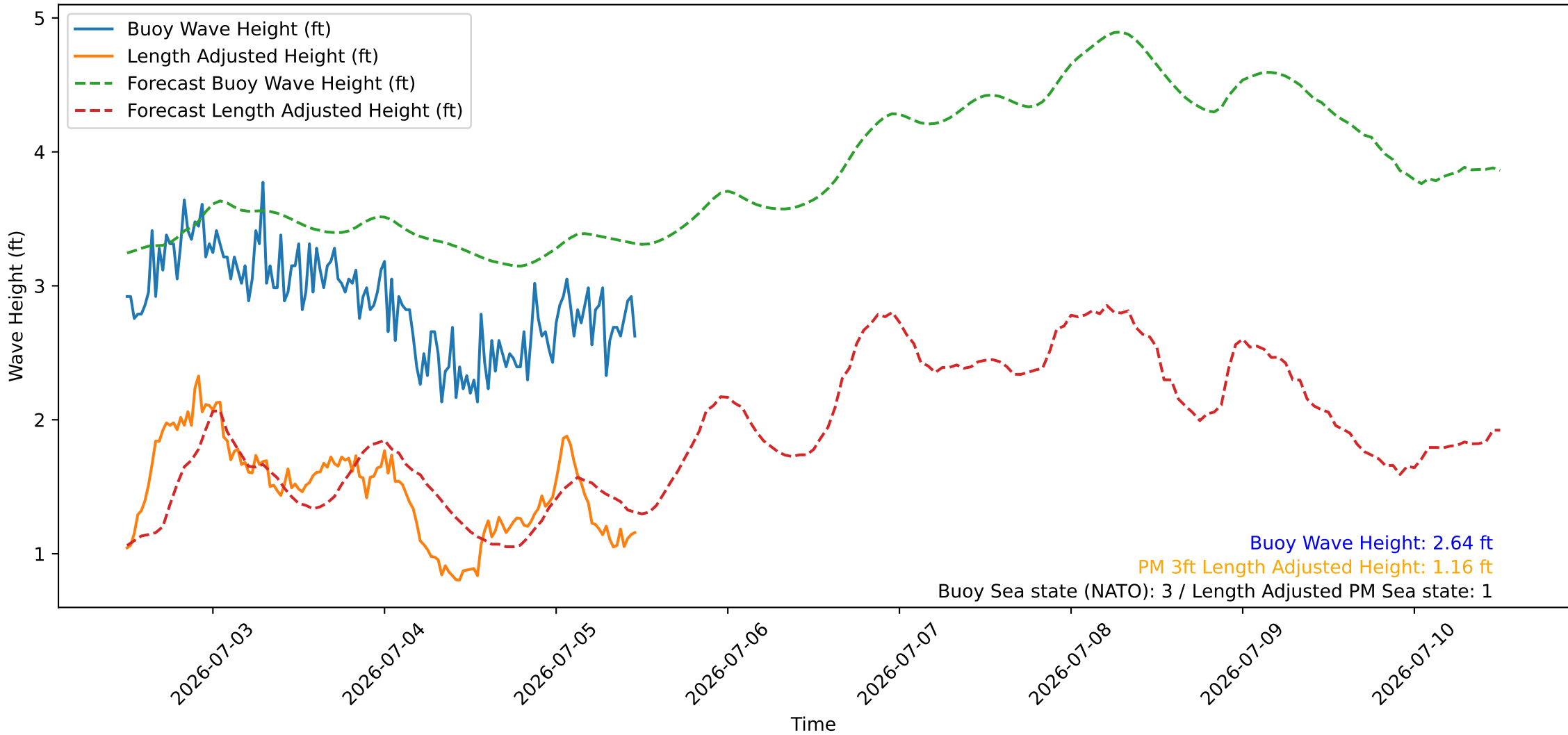
Wave Heights over Time for Oceanside Harbor at 2026-07-05 11:50:27
