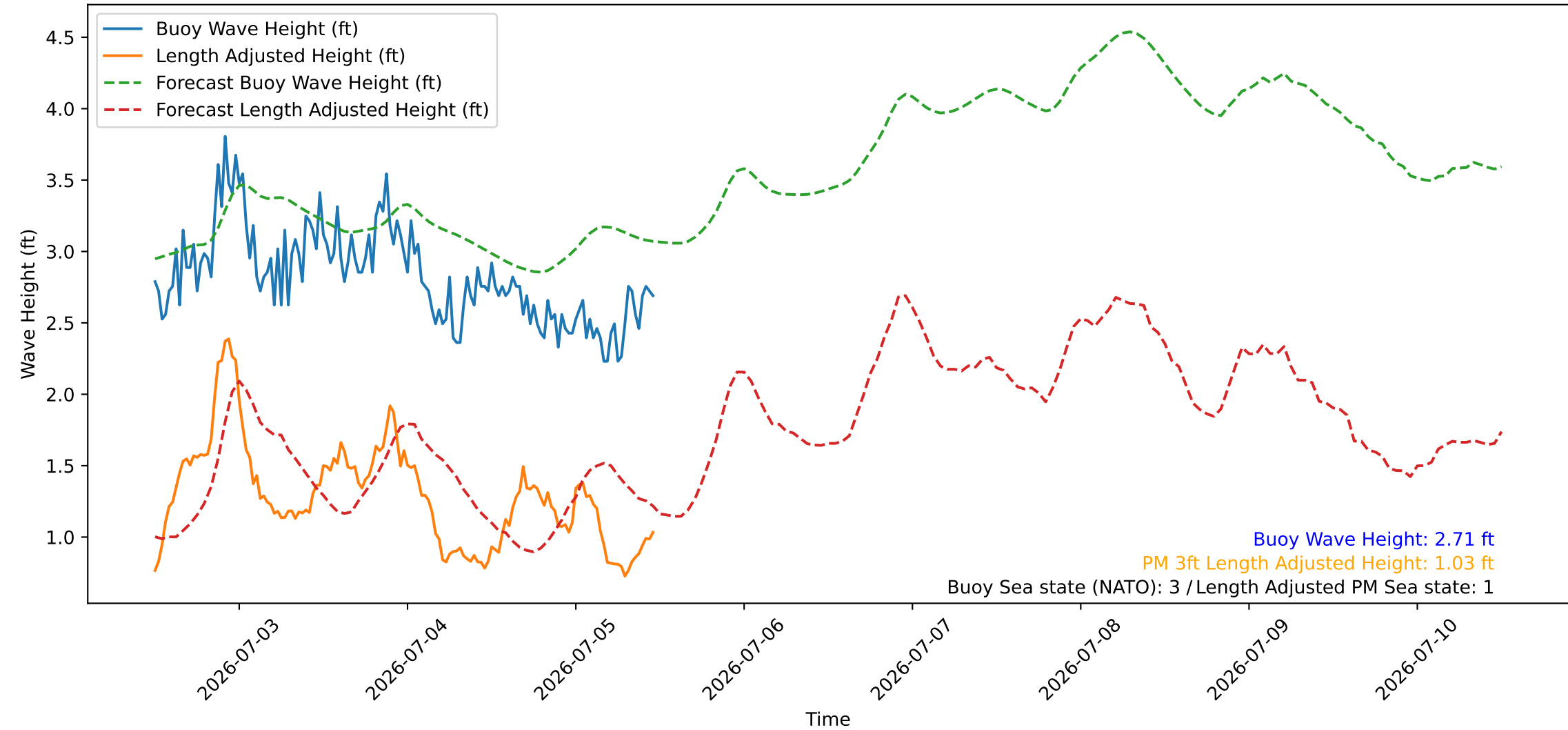
Wave Heights over Time for Red Beach at 2026-07-05 11:50:48
