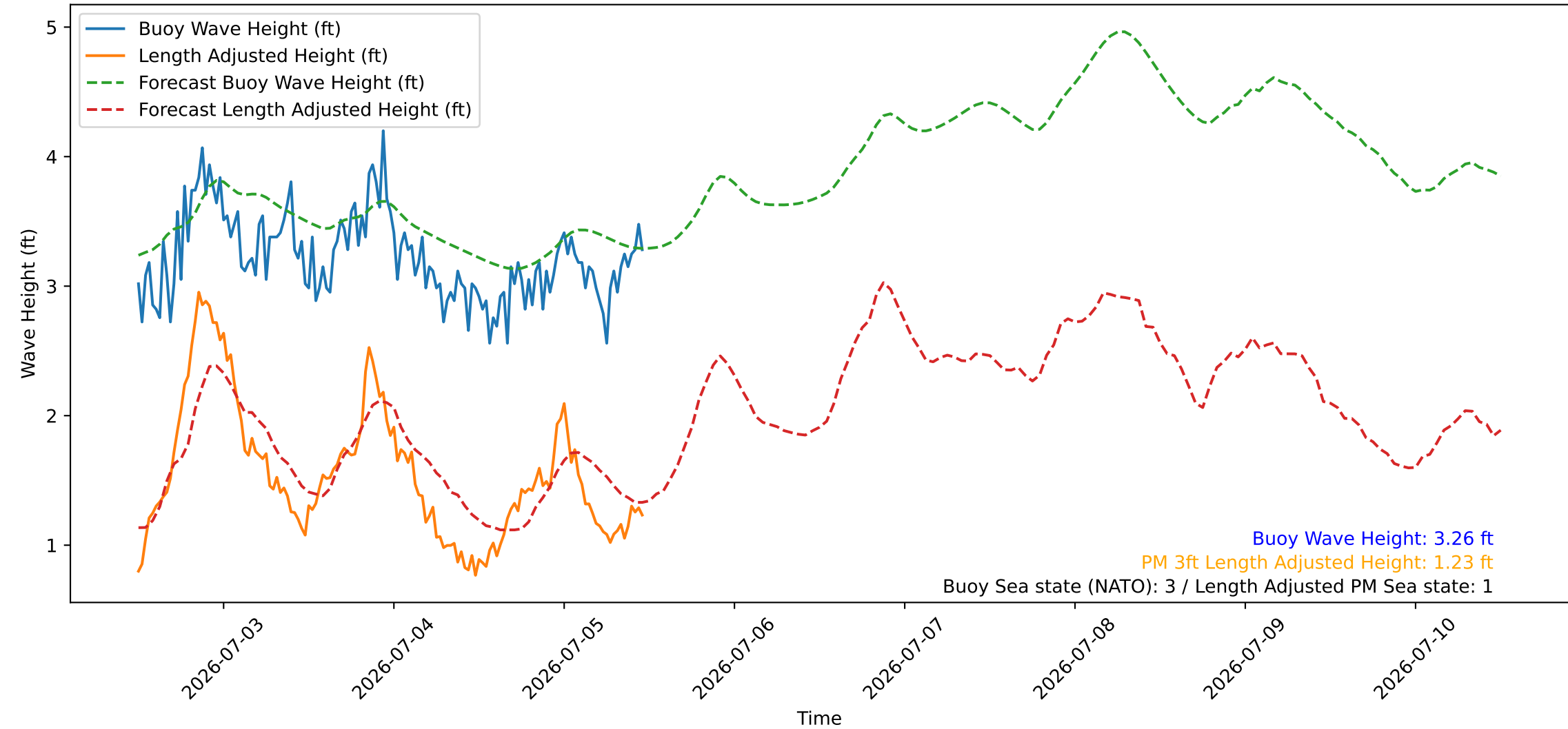
Wave Heights over Time for Green Beach at 2026-07-05 11:51:11
