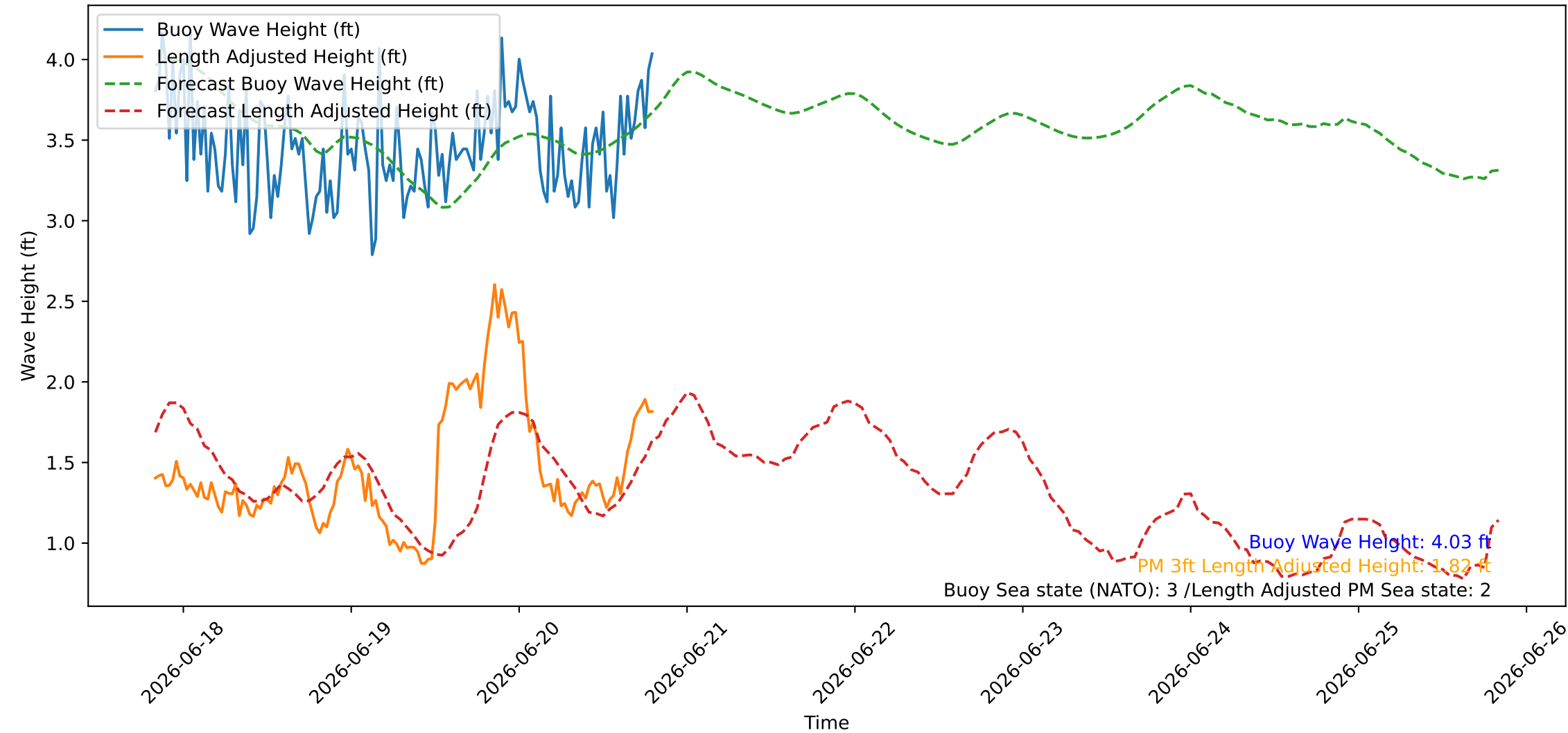
Wave Heights over Time for Oceanside Harbor at 2026-06-20 20:00:25
