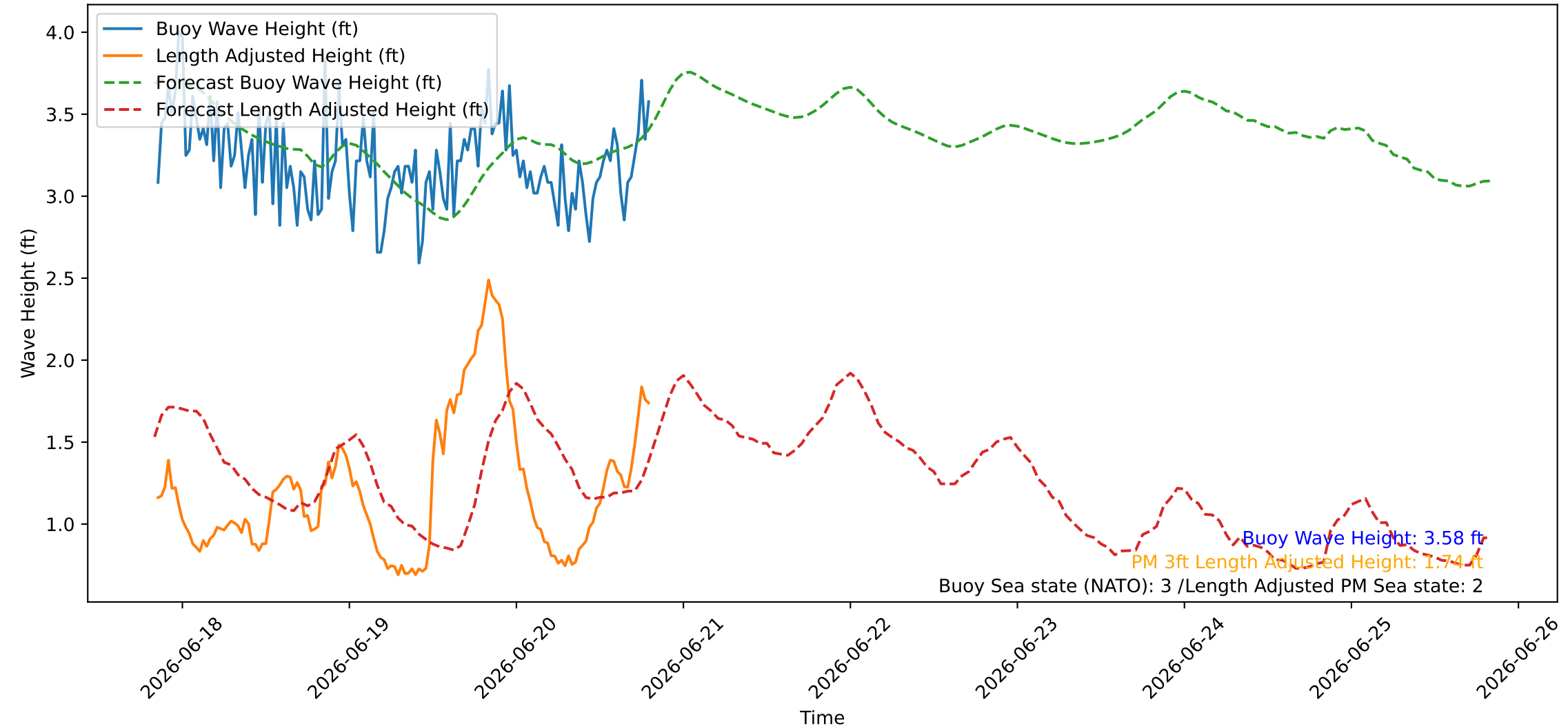
Wave Heights over Time for Red Beach at 2026-06-20 20:00:44
