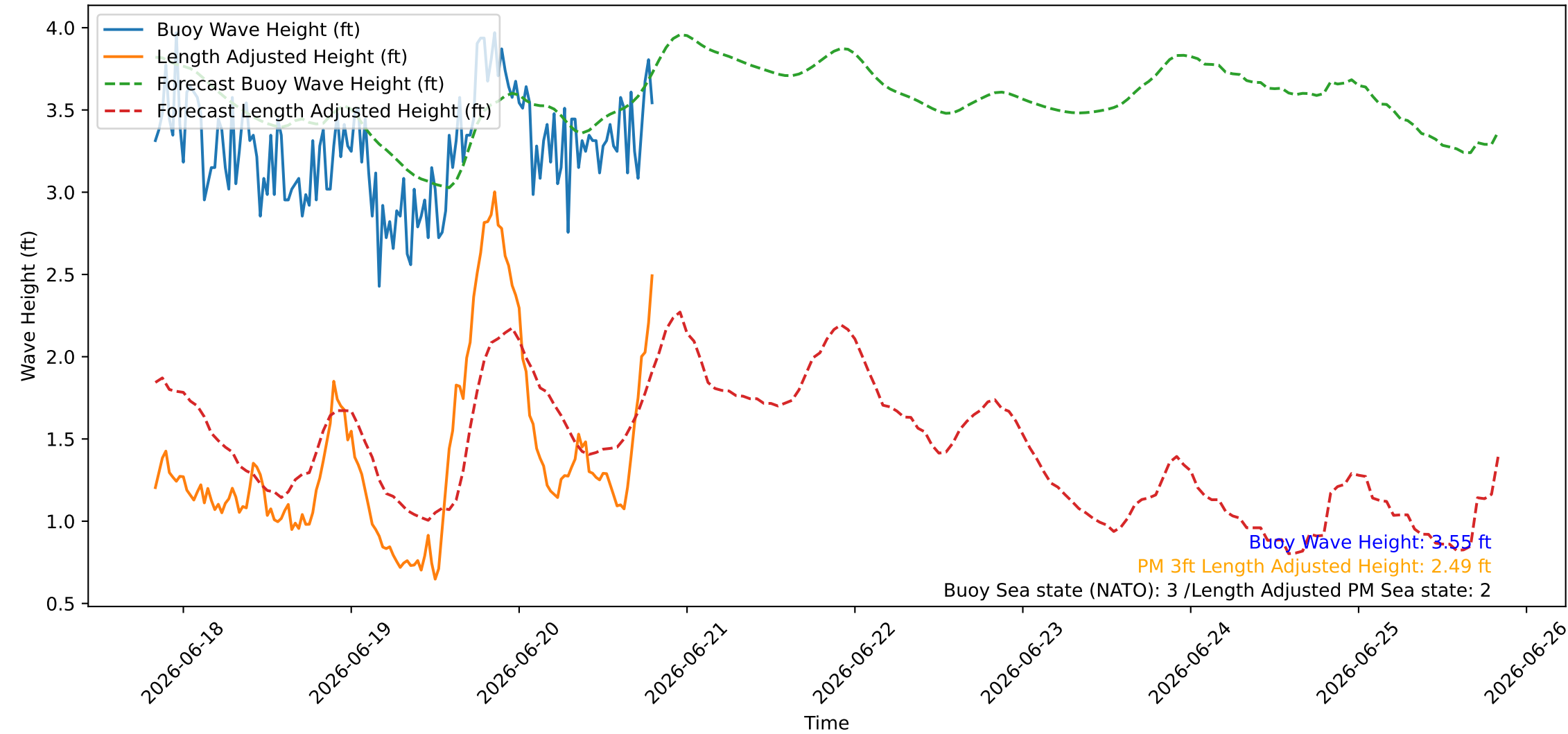
Wave Heights over Time for Green Beach at 2026-06-20 20:01:07
