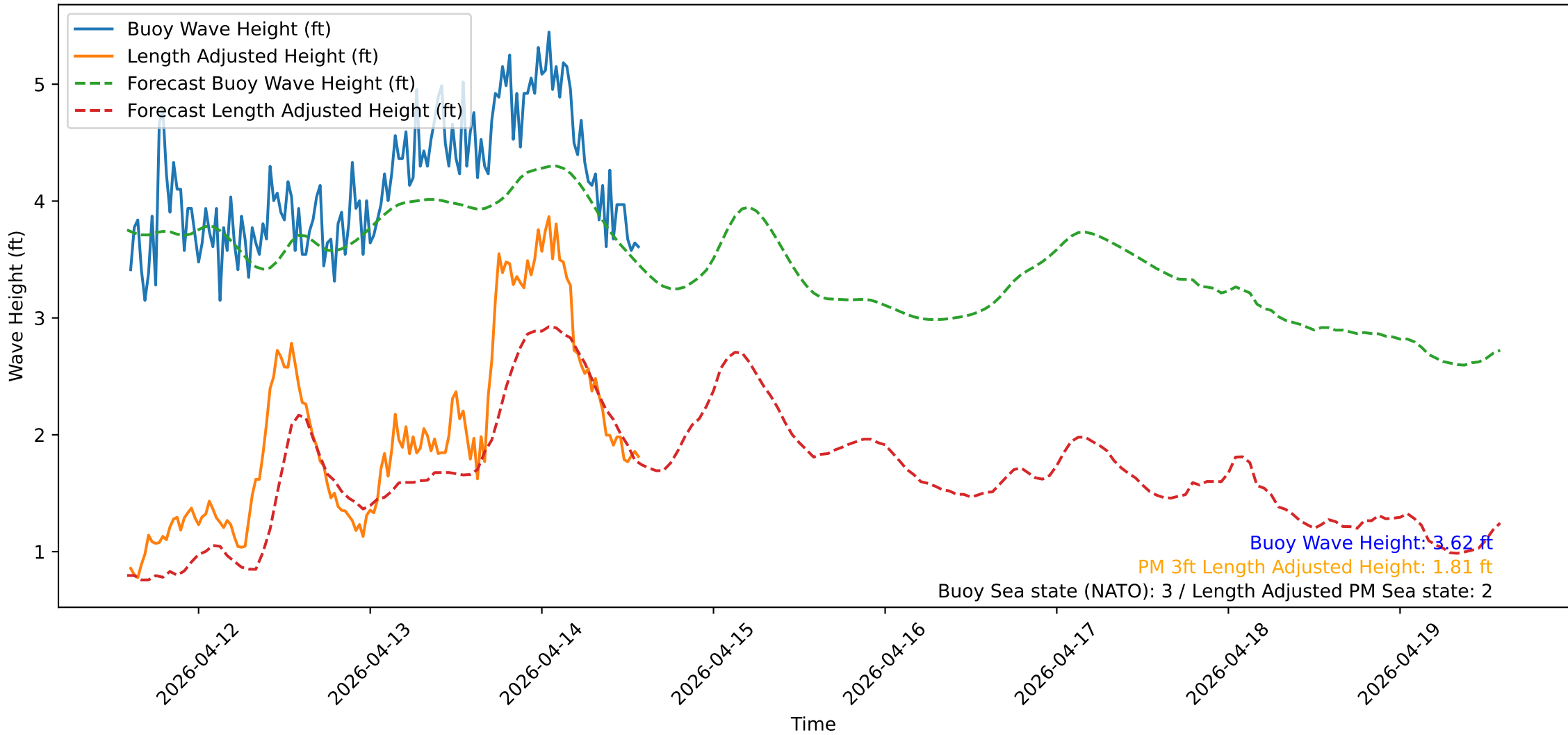
Wave Heights over Time for Oceanside Harbor at 2026-04-14 14:20:31
