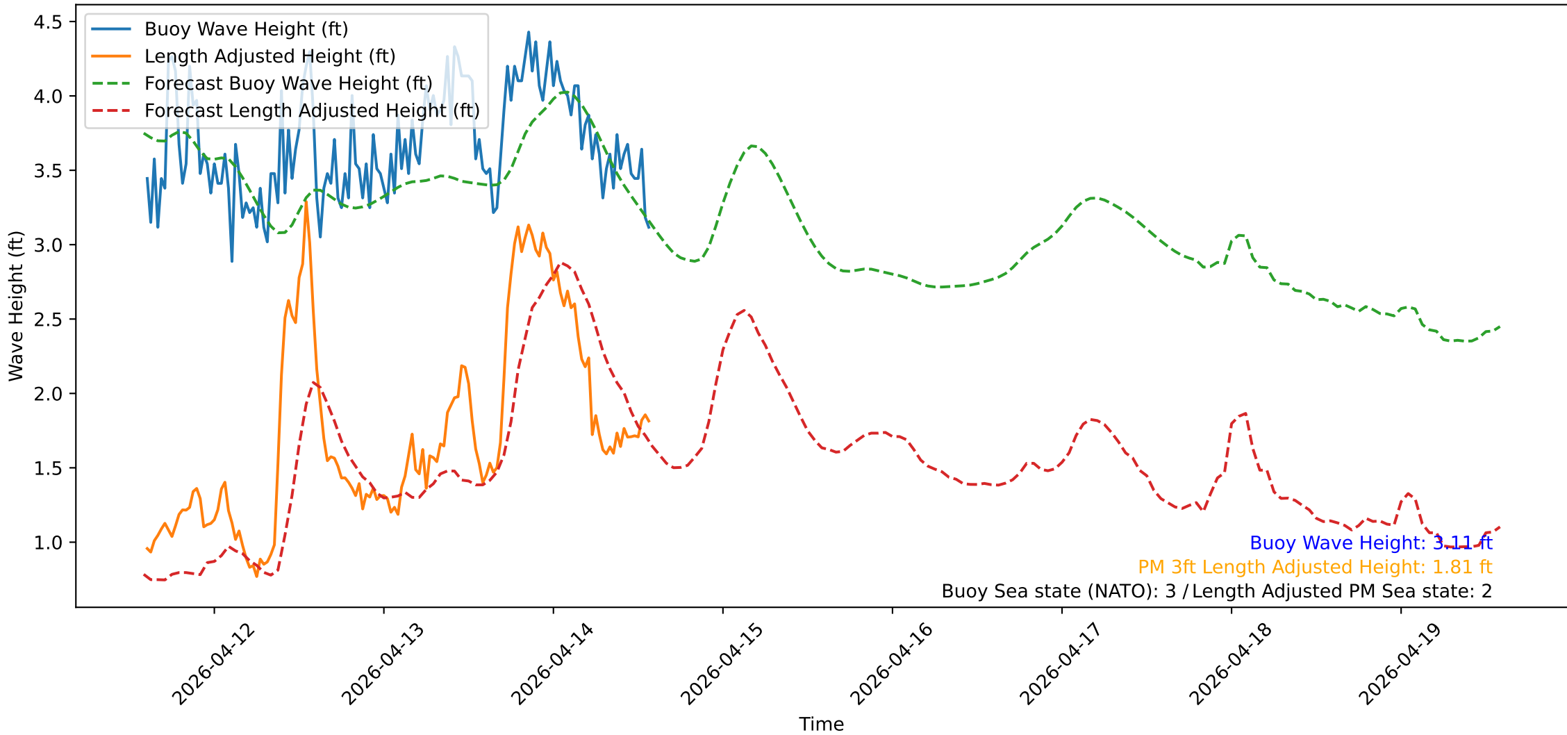
Wave Heights over Time for Red Beach at 2026-04-14 14:20:52
