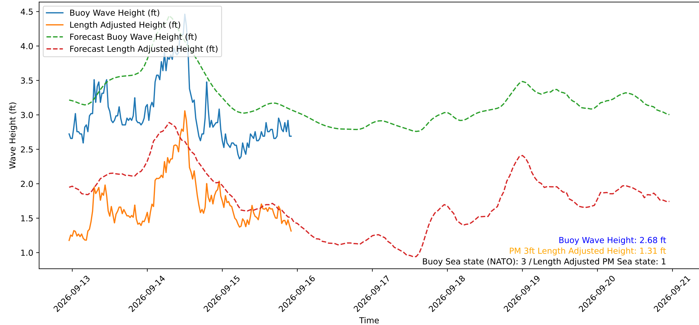
Wave Heights over Time for Oceanside Harbor at 2026-09-15 22:50:30
