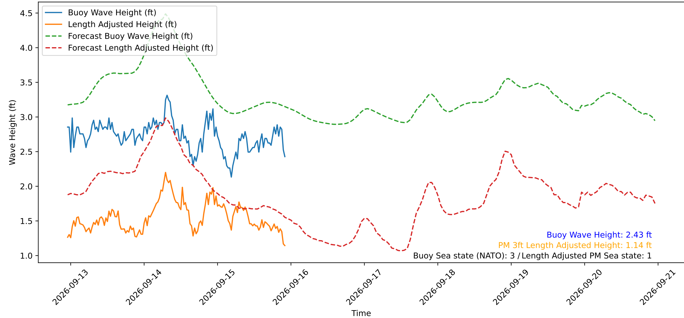
Wave Heights over Time for Green Beach at 2026-09-15 22:51:15
