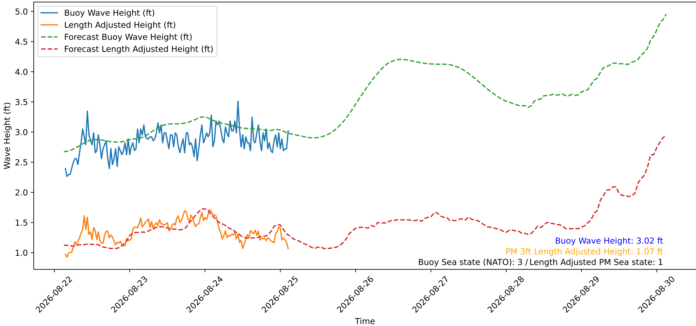
Wave Heights over Time for Oceanside Harbor at 2026-08-25 03:20:30
