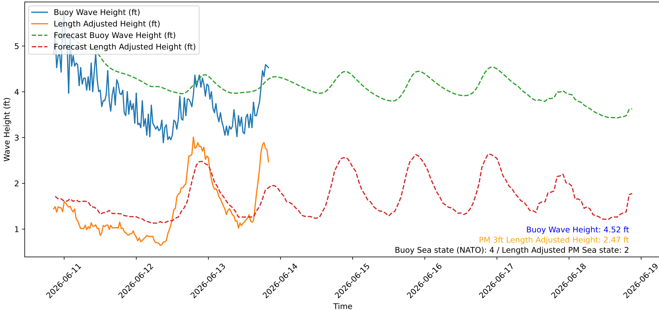
Wave Heights over Time for Green Beach at 2026-06-13 20:41:09
