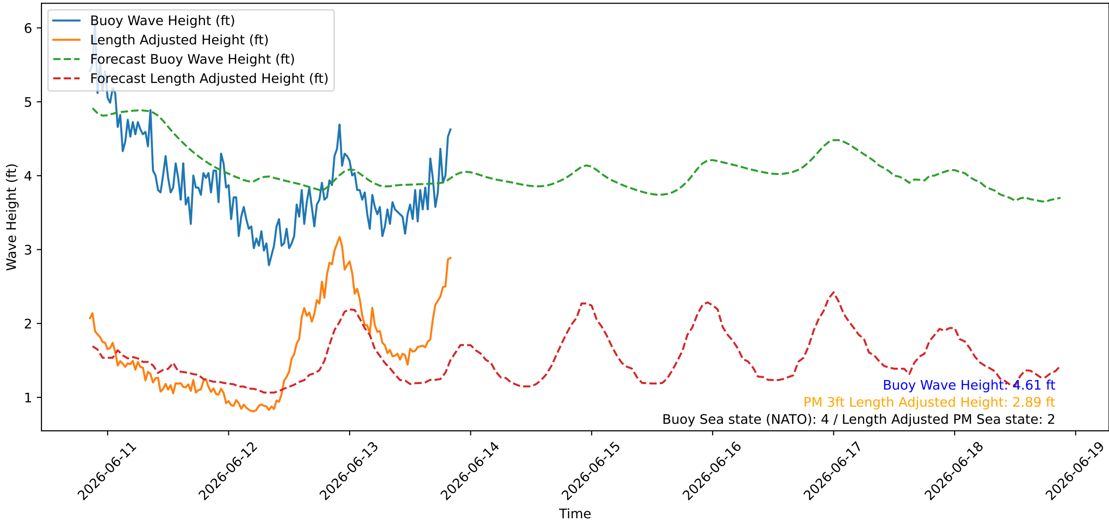
Wave Heights over Time for Oceanside Harbor at 2026-06-13 20:40:27
