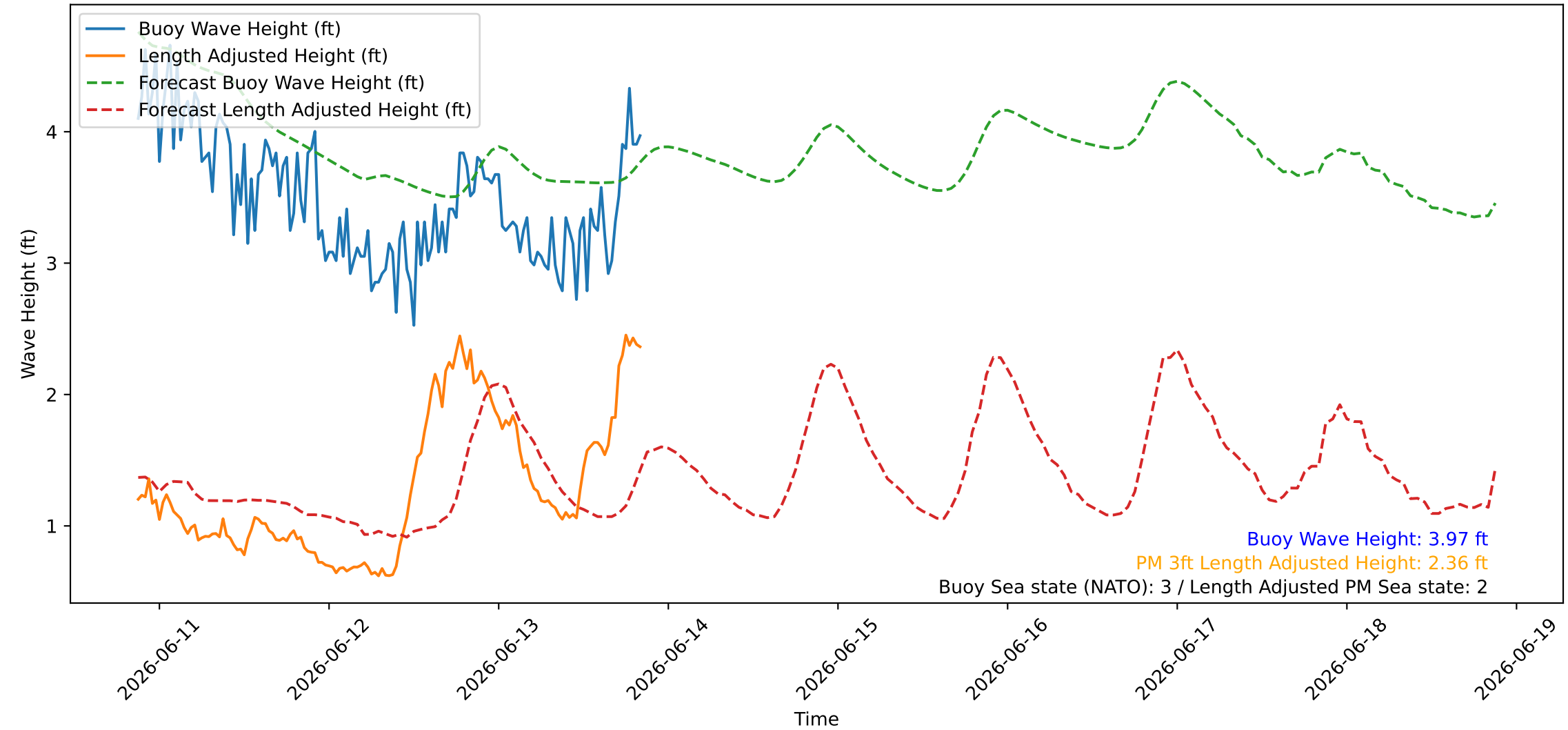
Wave Heights over Time for Red Beach at 2026-06-13 20:40:46
