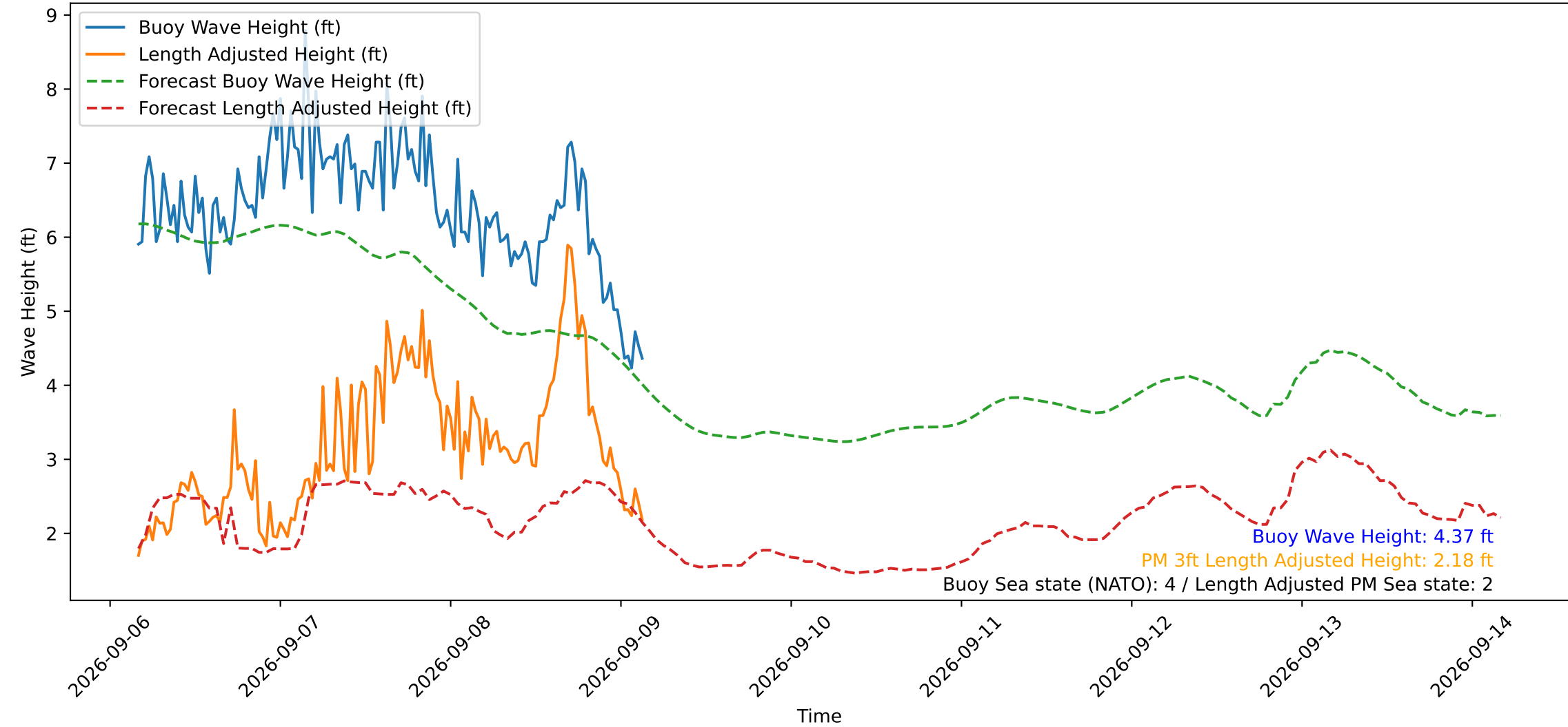
Wave Heights over Time for Green Beach at 2026-09-09 03:51:14
