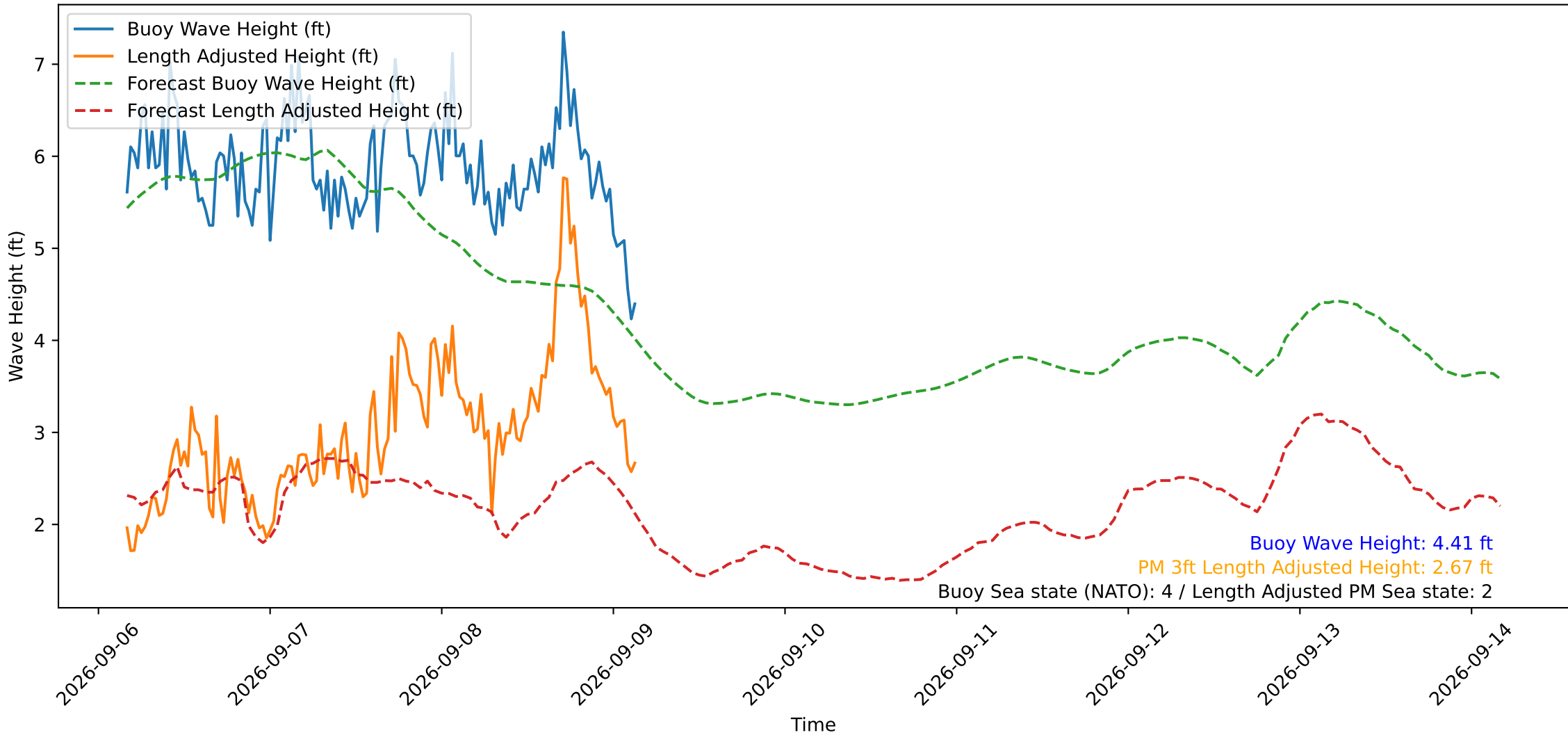
Wave Heights over Time for Oceanside Harbor at 2026-09-09 03:50:29
