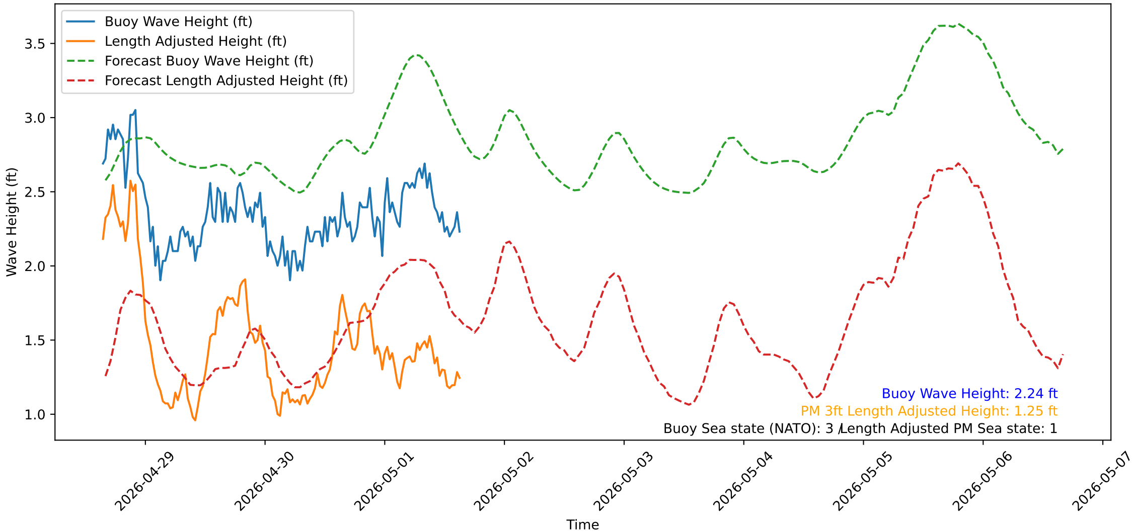
Wave Heights over Time for Oceanside Harbor at 2026-05-01 15:30:31
