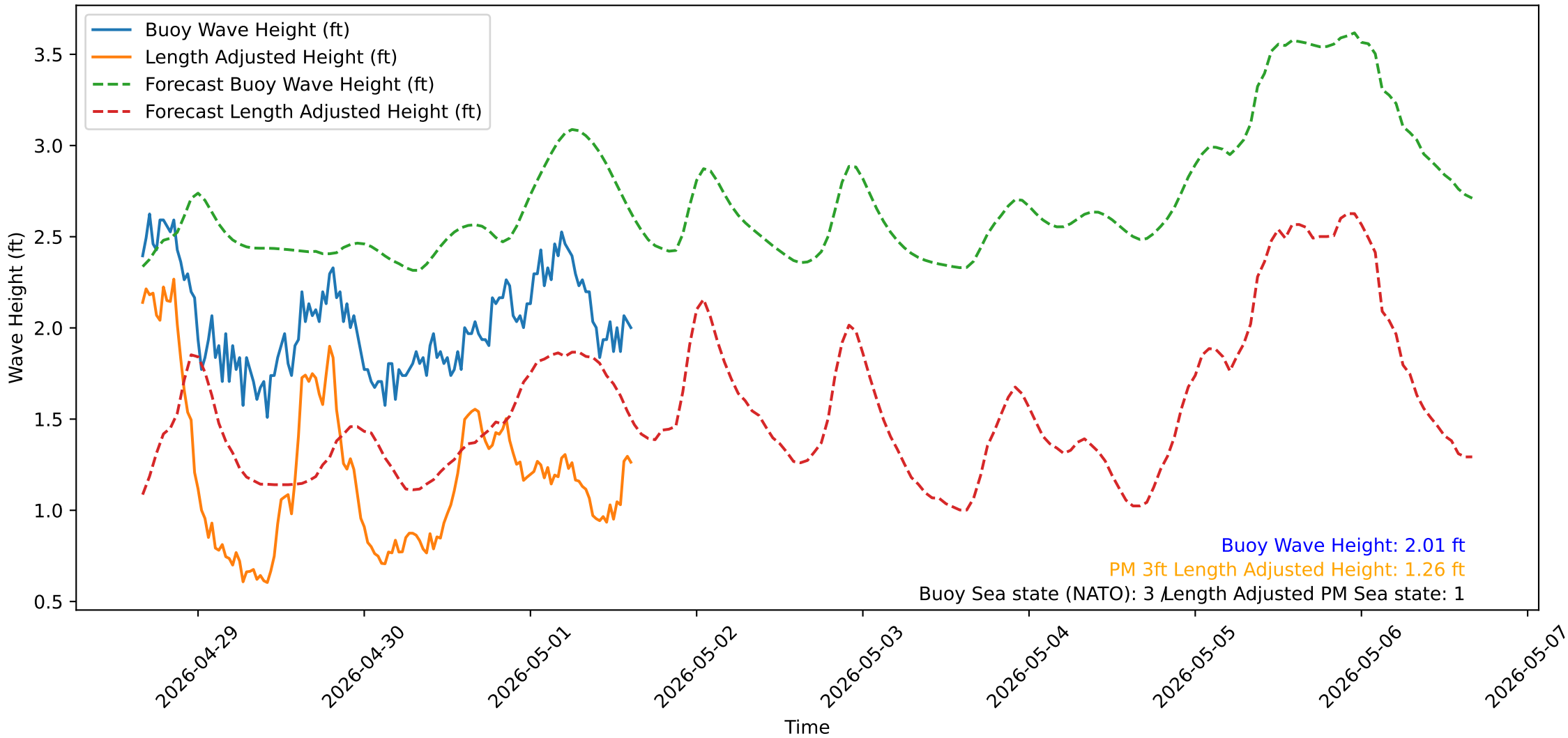
Wave Heights over Time for Red Beach at 2026-05-01 15:30:50
