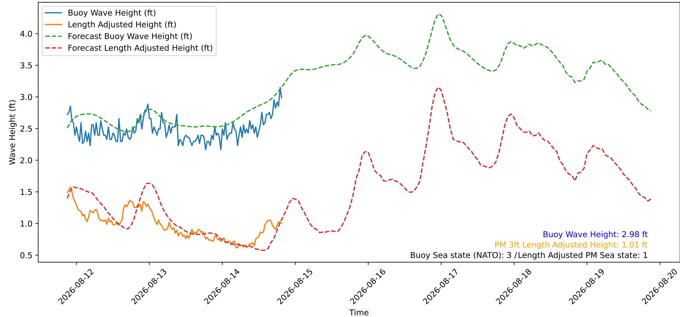
Wave Heights over Time for Red Beach at 2026-08-14 20:30:47
