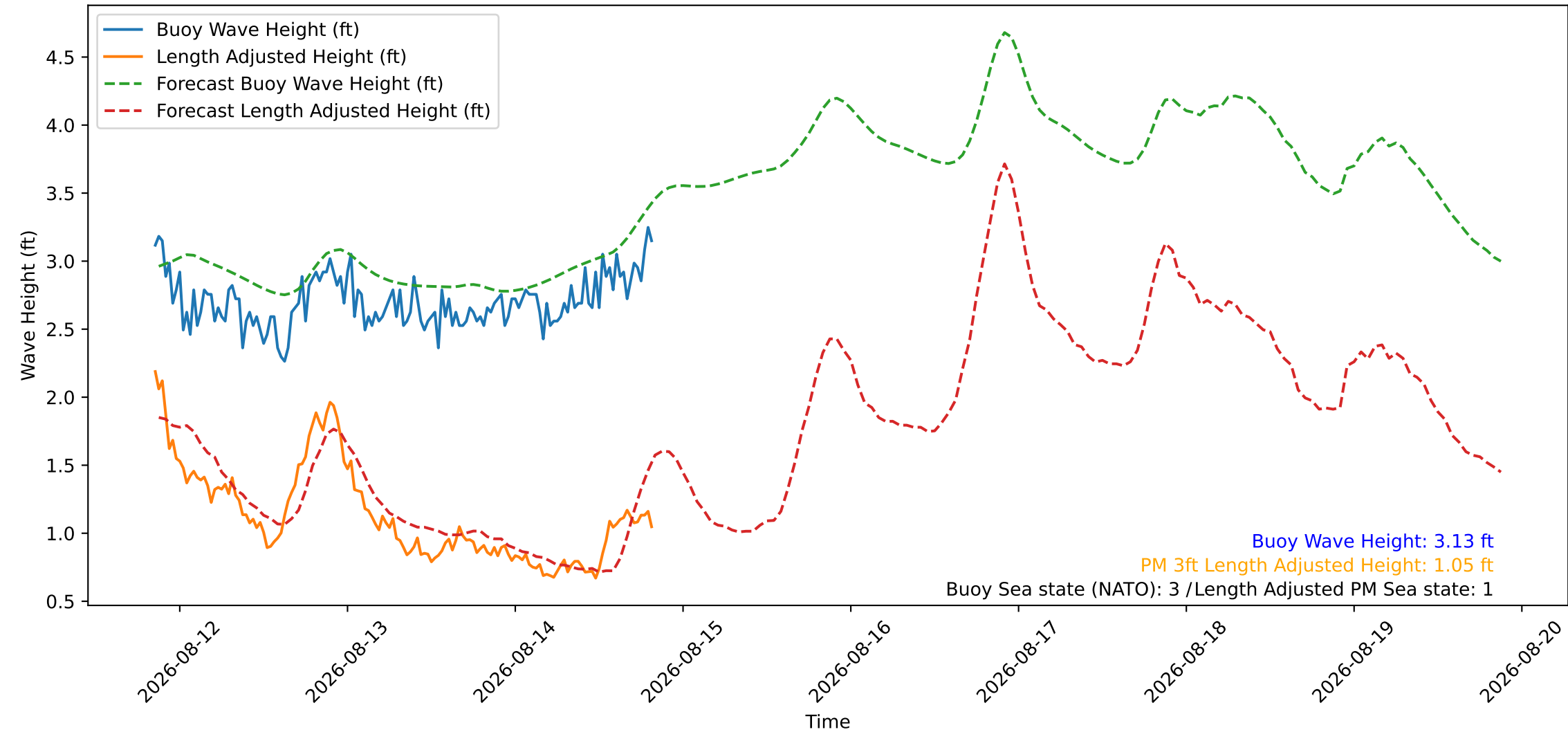
Wave Heights over Time for Green Beach at 2026-08-14 20:31:09
