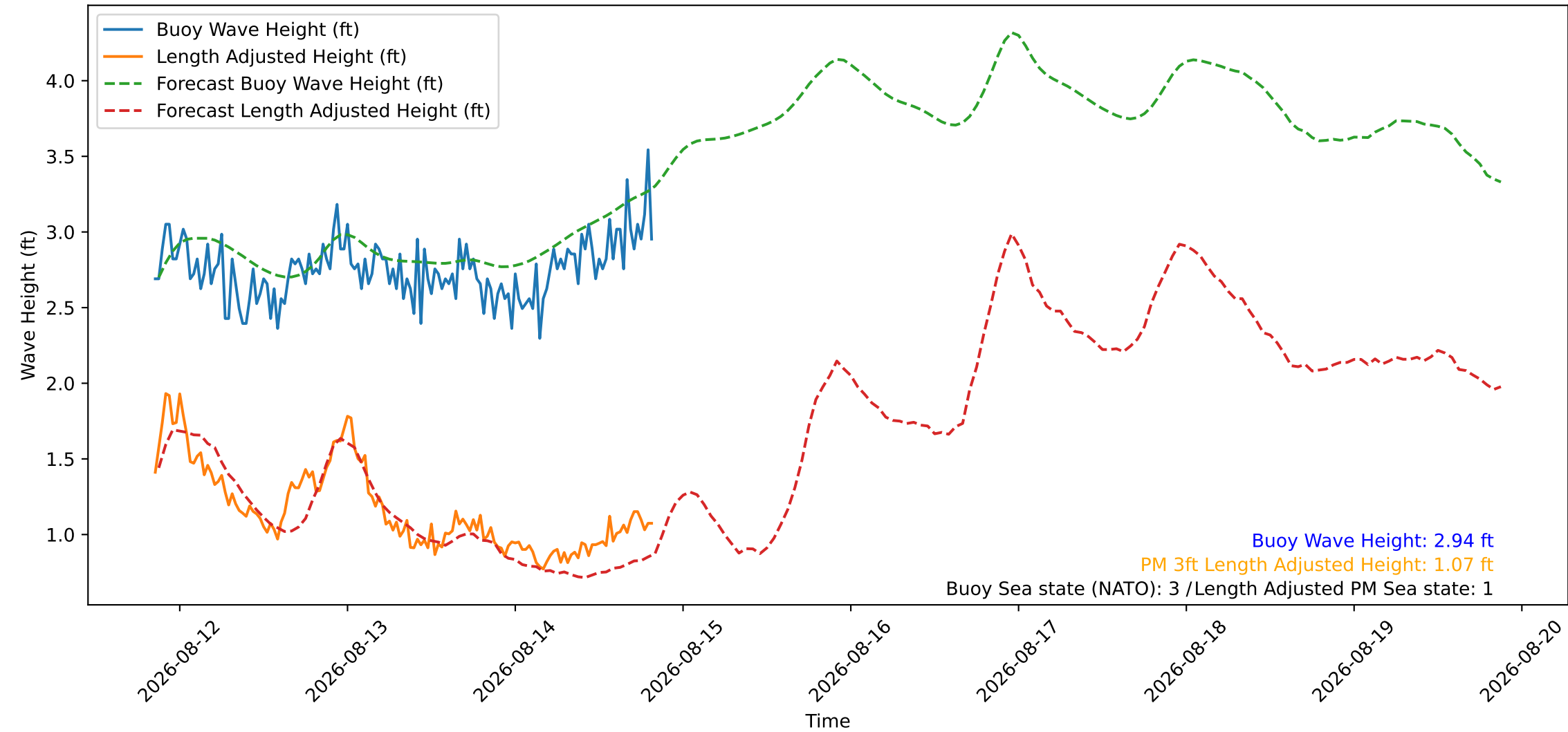
Wave Heights over Time for Oceanside Harbor at 2026-08-14 20:30:27
