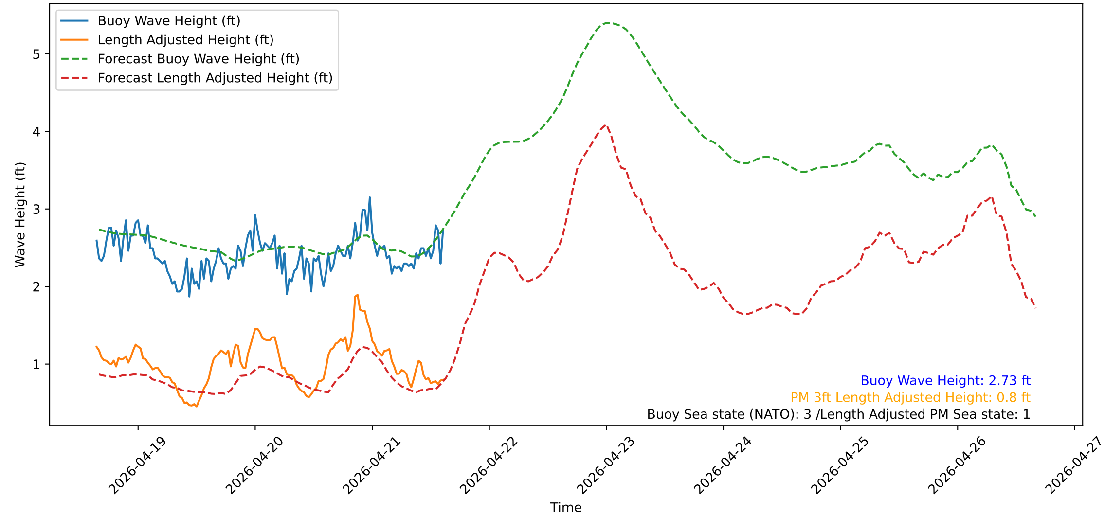
Wave Heights over Time for Green Beach at 2026-04-21 15:31:13
