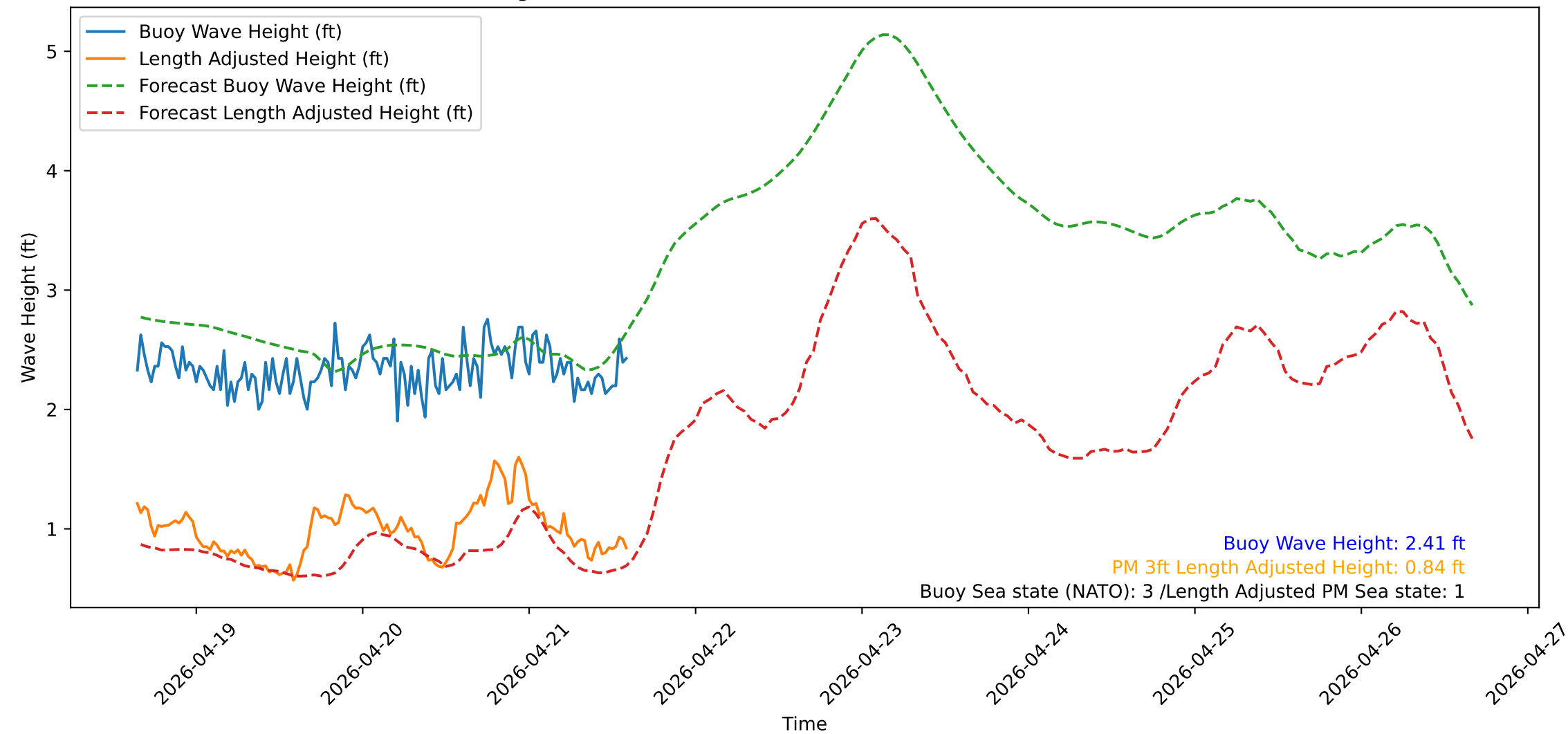
Wave Heights over Time for Oceanside Harbor at 2026-04-21 15:30:32
