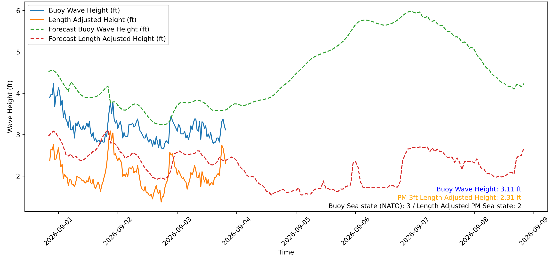
Wave Heights over Time for Green Beach at 2026-09-03 20:11:12
