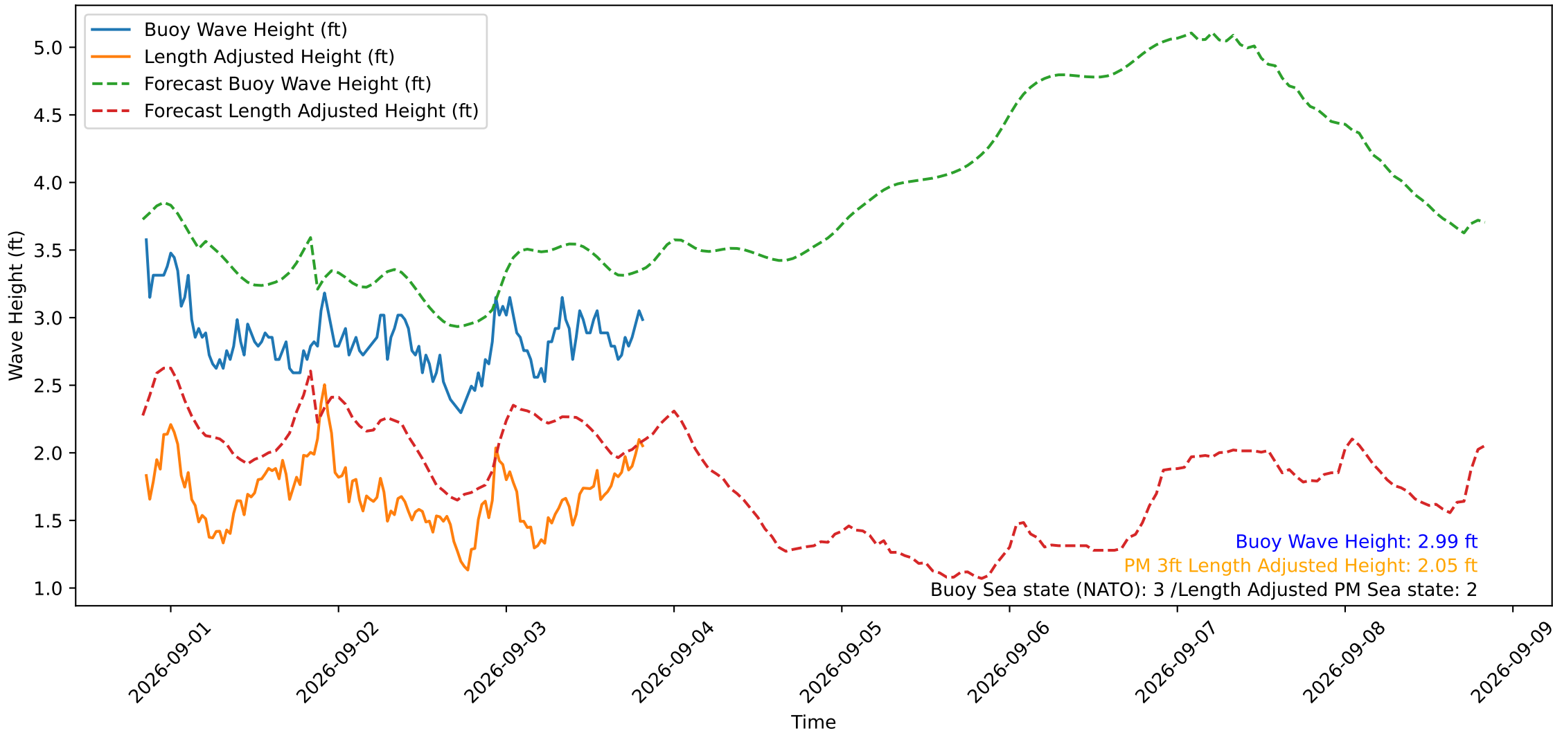
Wave Heights over Time for Red Beach at 2026-09-03 20:10:49
