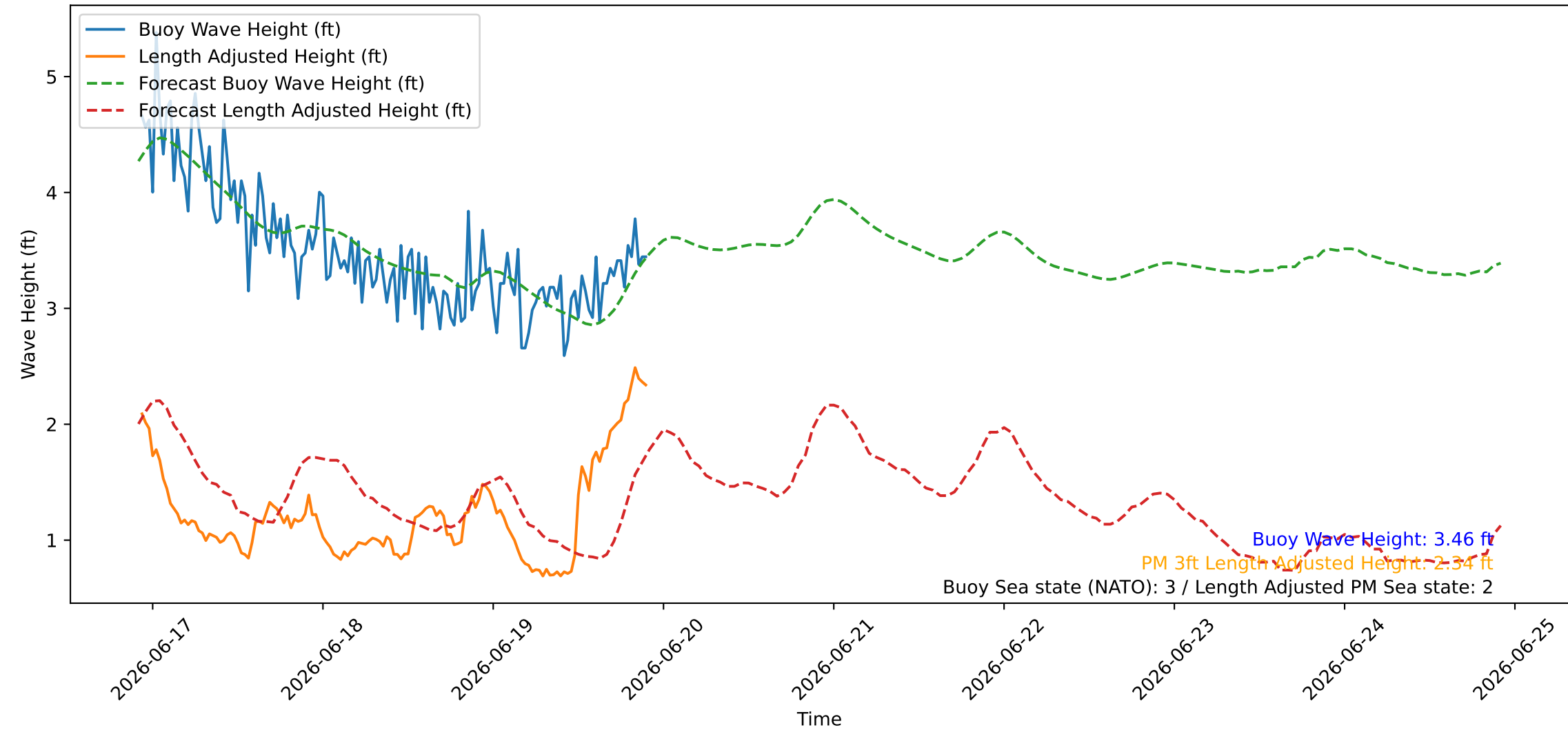
Wave Heights over Time for Red Beach at 2026-06-19 22:20:46
