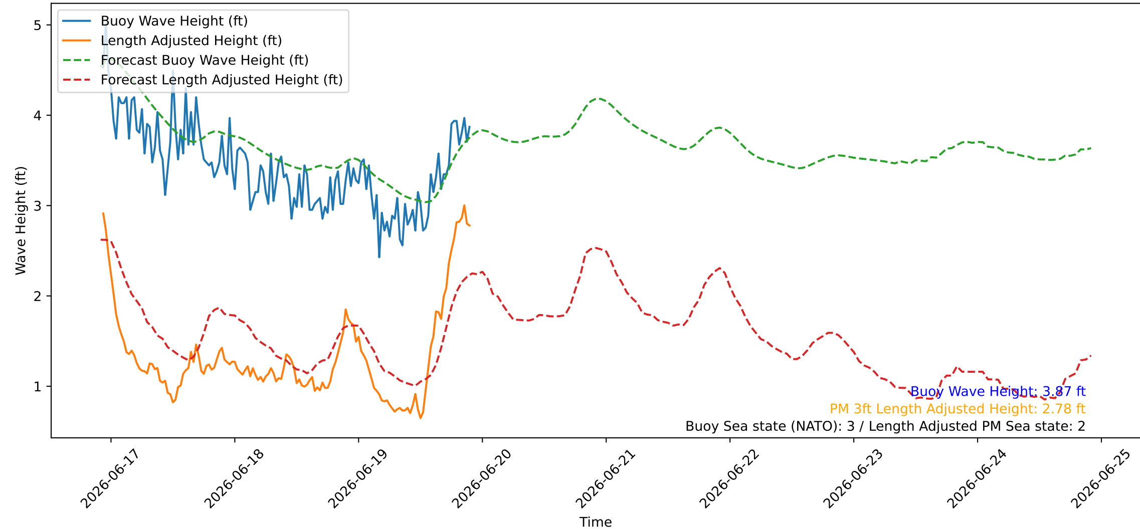
Wave Heights over Time for Green Beach at 2026-06-19 22:21:08
