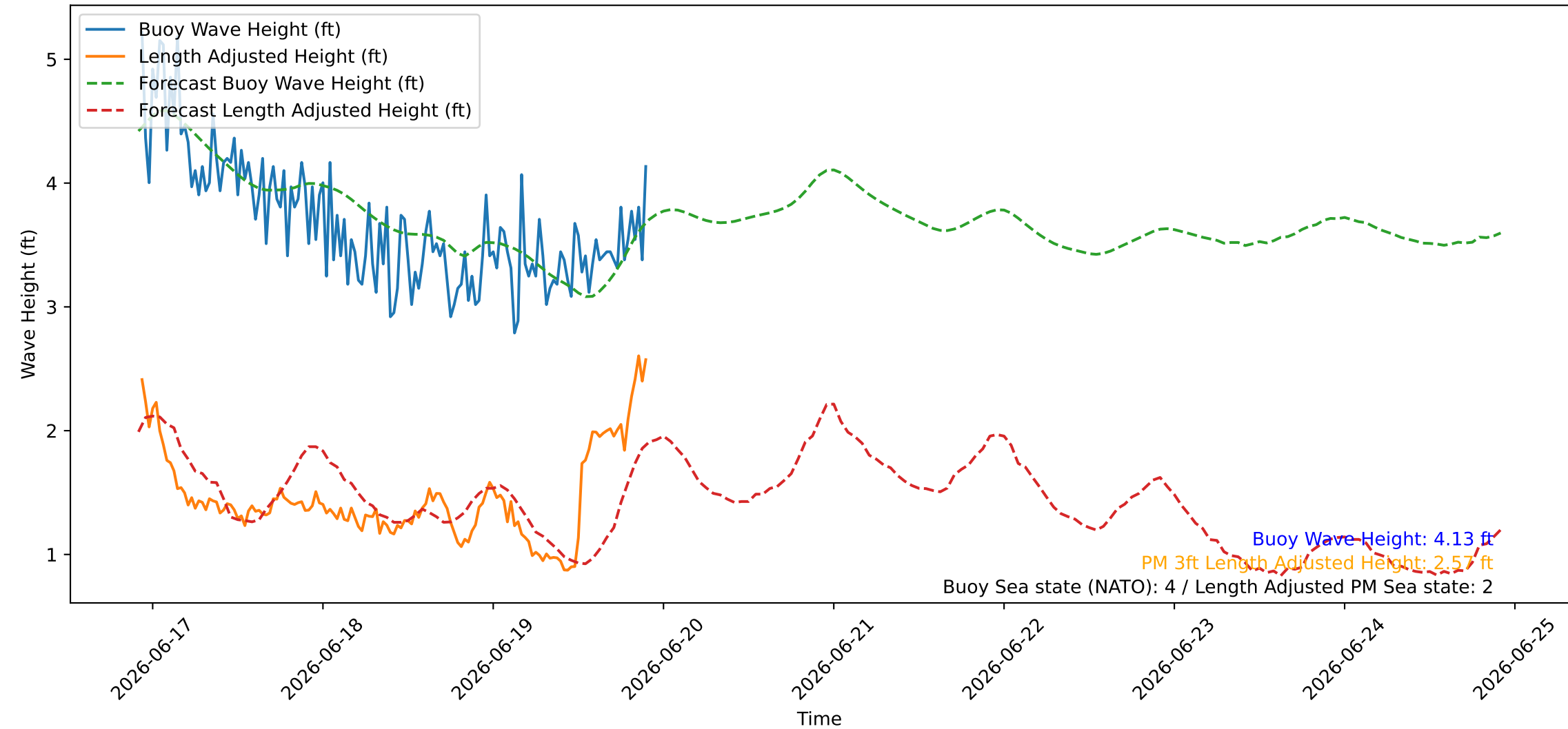
Wave Heights over Time for Oceanside Harbor at 2026-06-19 22:20:26
