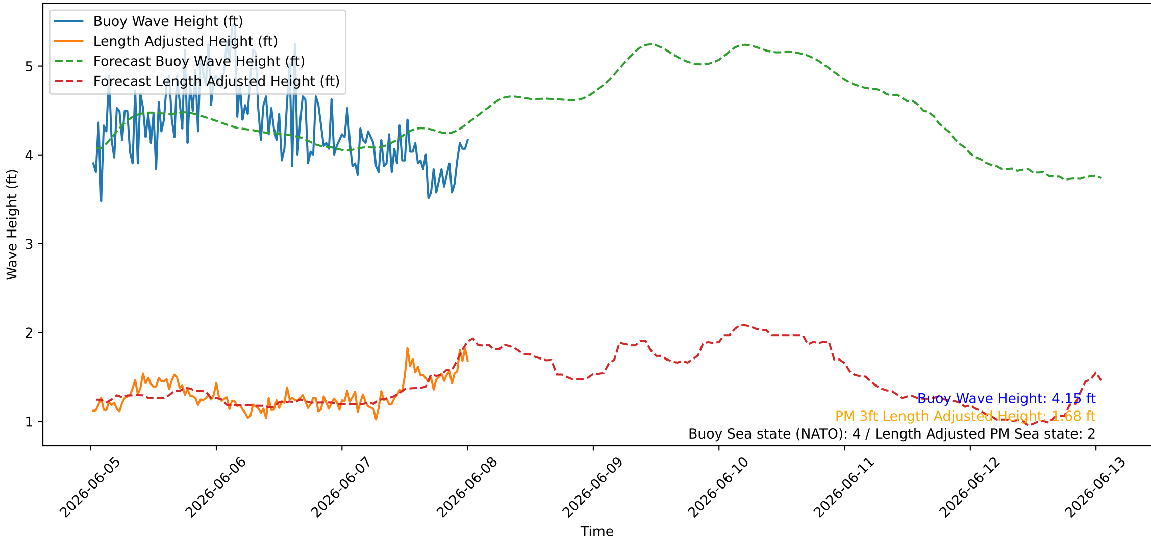
Wave Heights over Time for Oceanside Harbor at 2026-06-08 00:40:26
